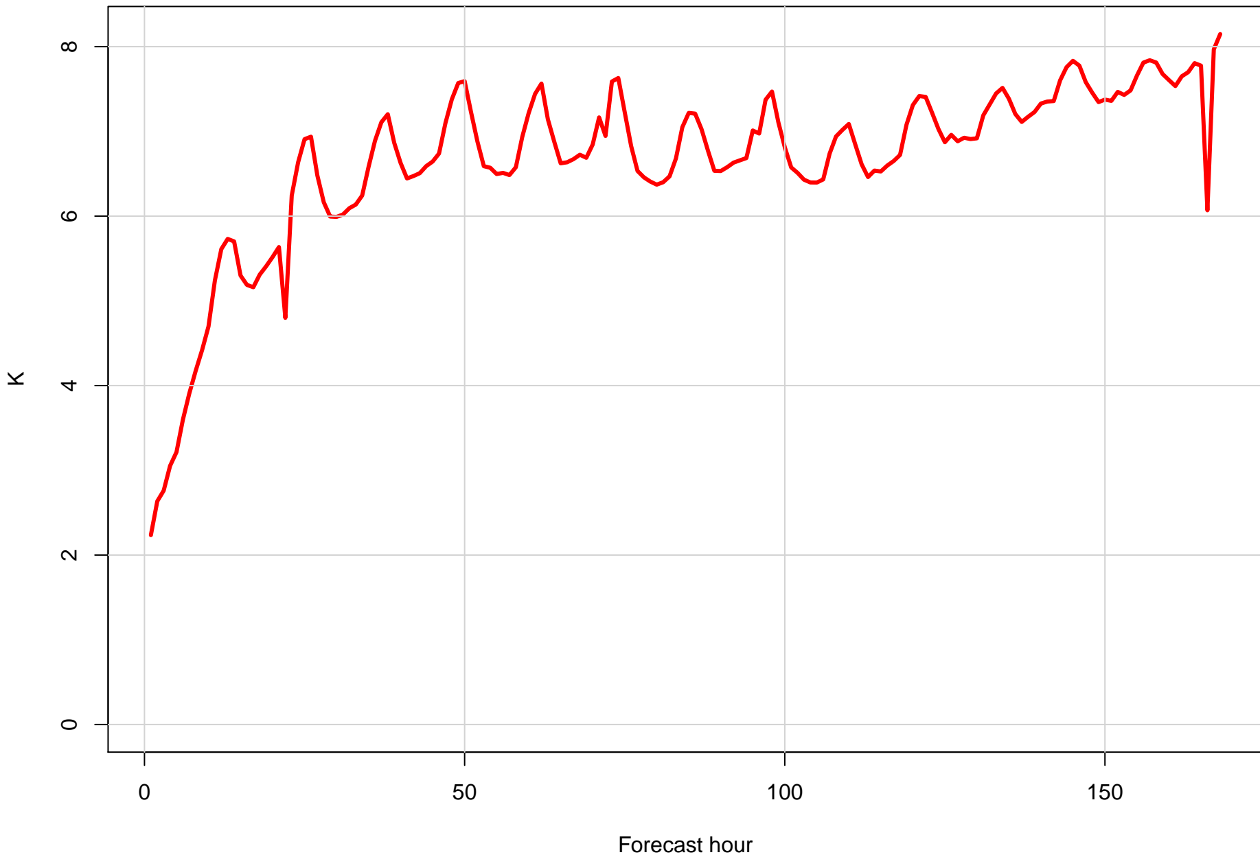
Surface dew point RMSE at KBQP by forecast hour
