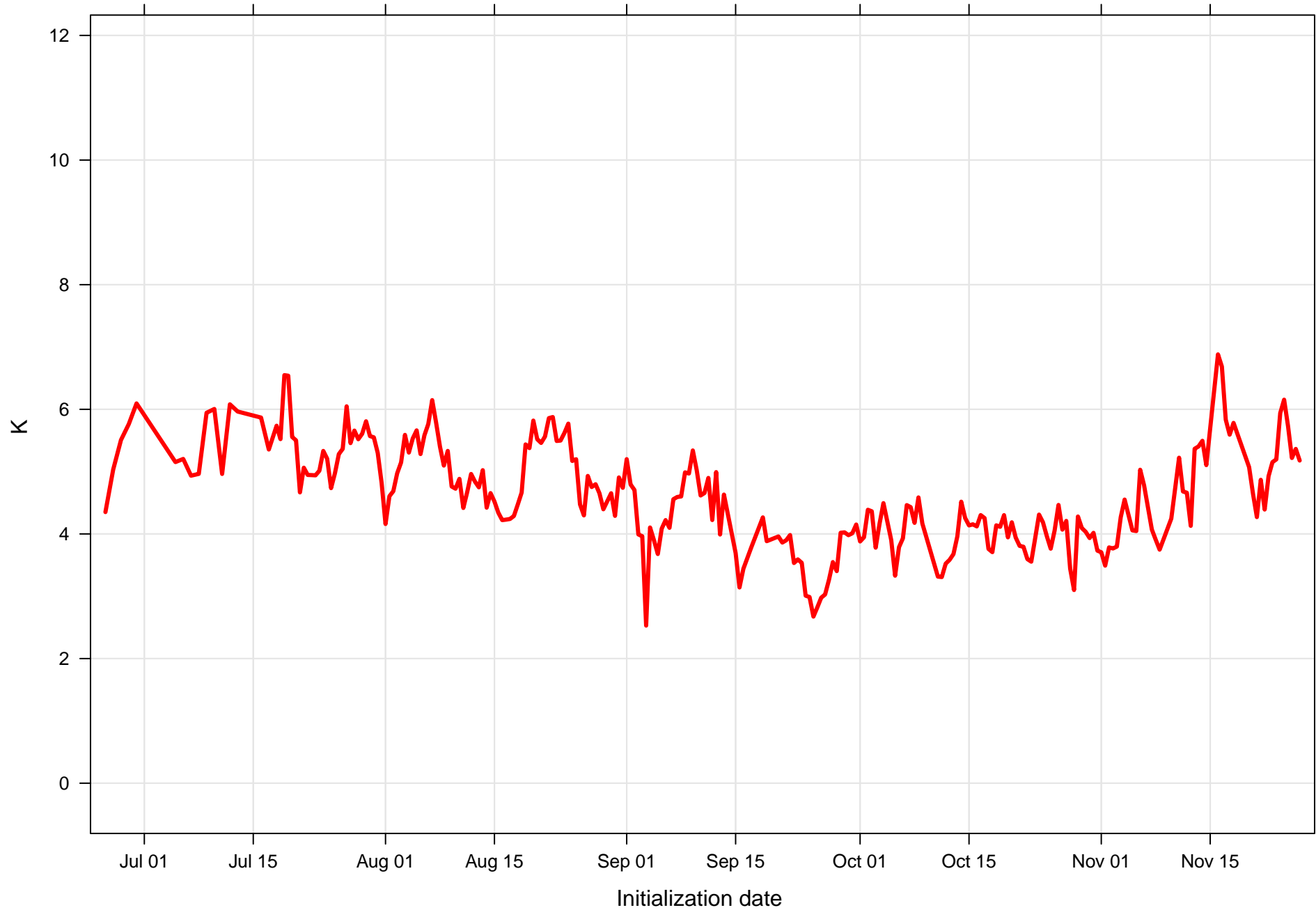
Surface dew point RMSE at KBQP all forecast hours and members
