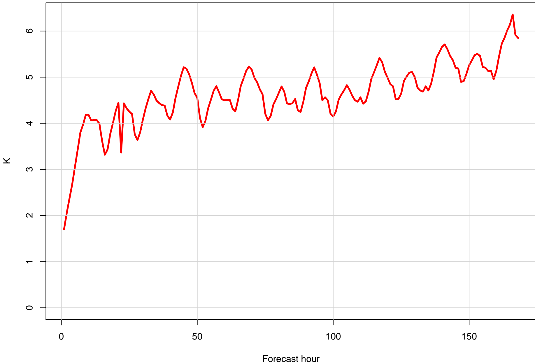
Surface temperature RMSE at KBQP by forecast hour
