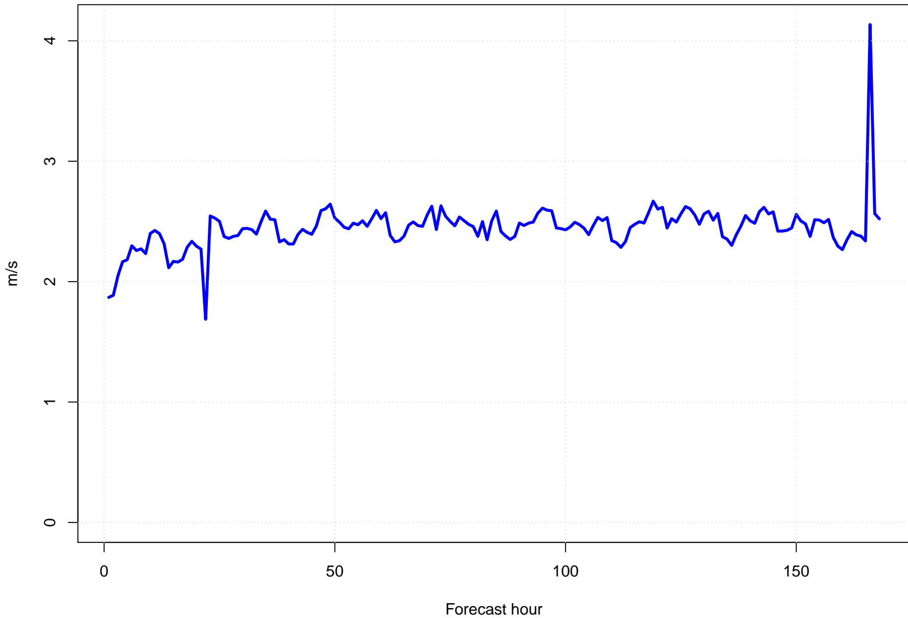
Surface wind speed bias at KBQP by forecast hour
