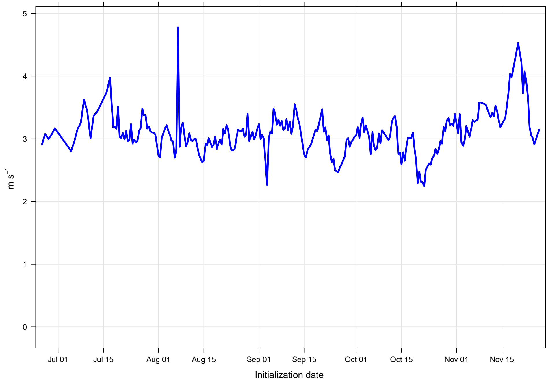
Surface vector wind mean error KBQP all forecast hours and members
