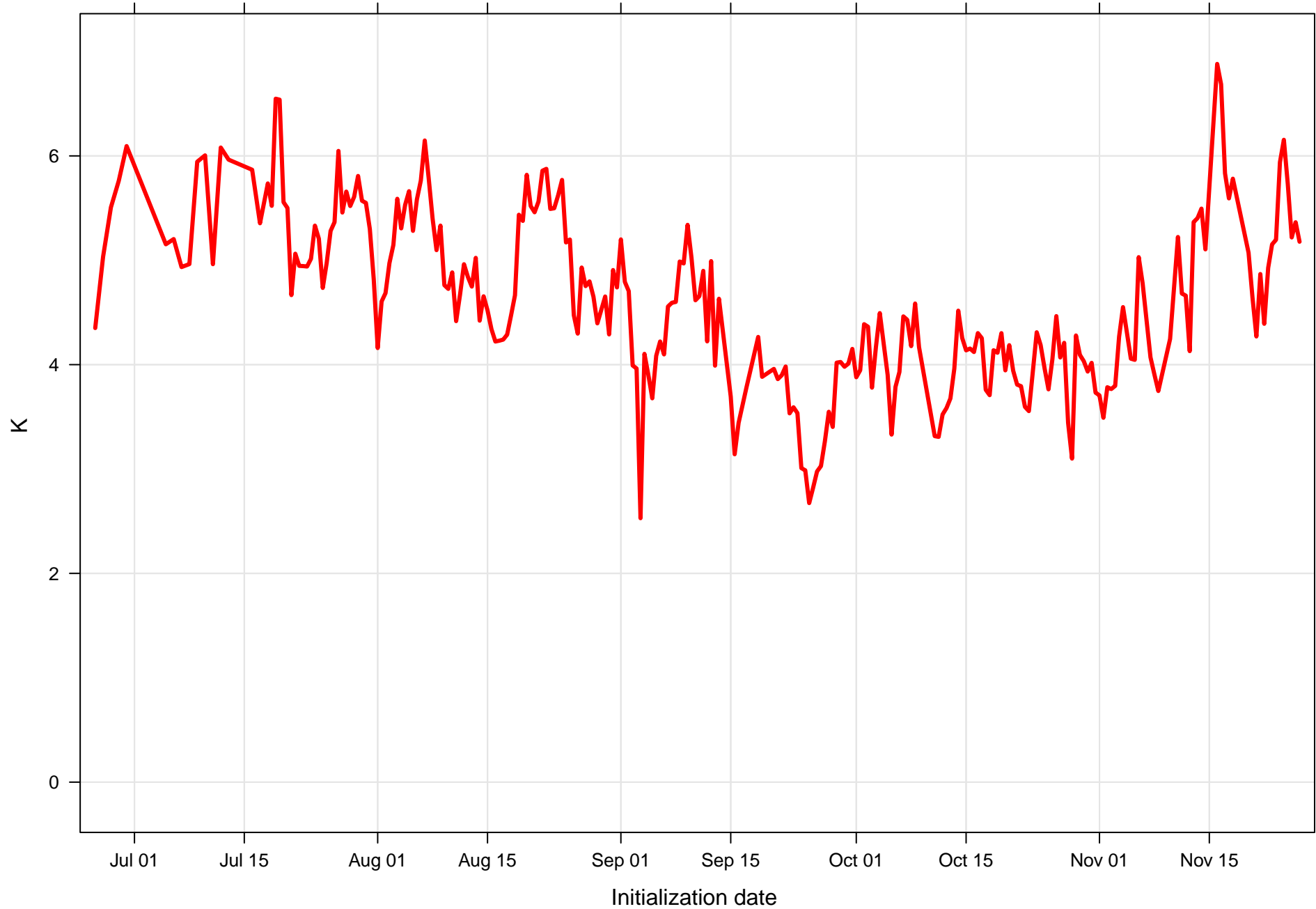
Surface temperature RMSE at KBQP all forecast hours and members
