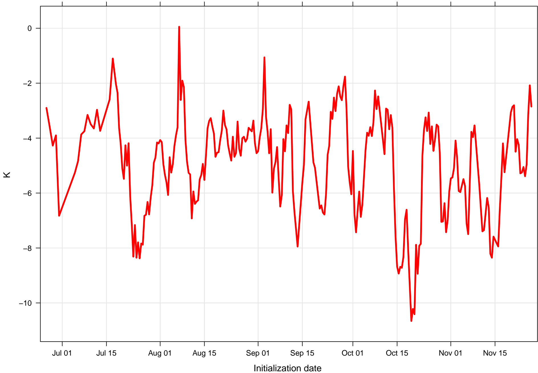
Surface dew point bias at KBQP all forecast hours and members
