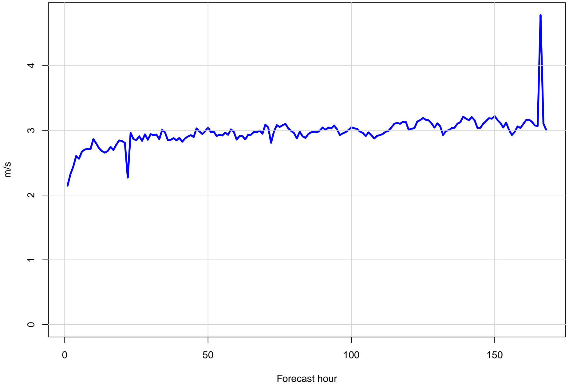
Surface wind speed RMSE at KBQP by forecast hour
