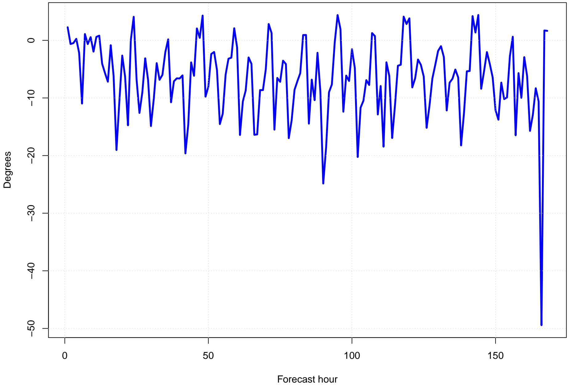
Surface wind direction bias at KEYW by forecast hour
