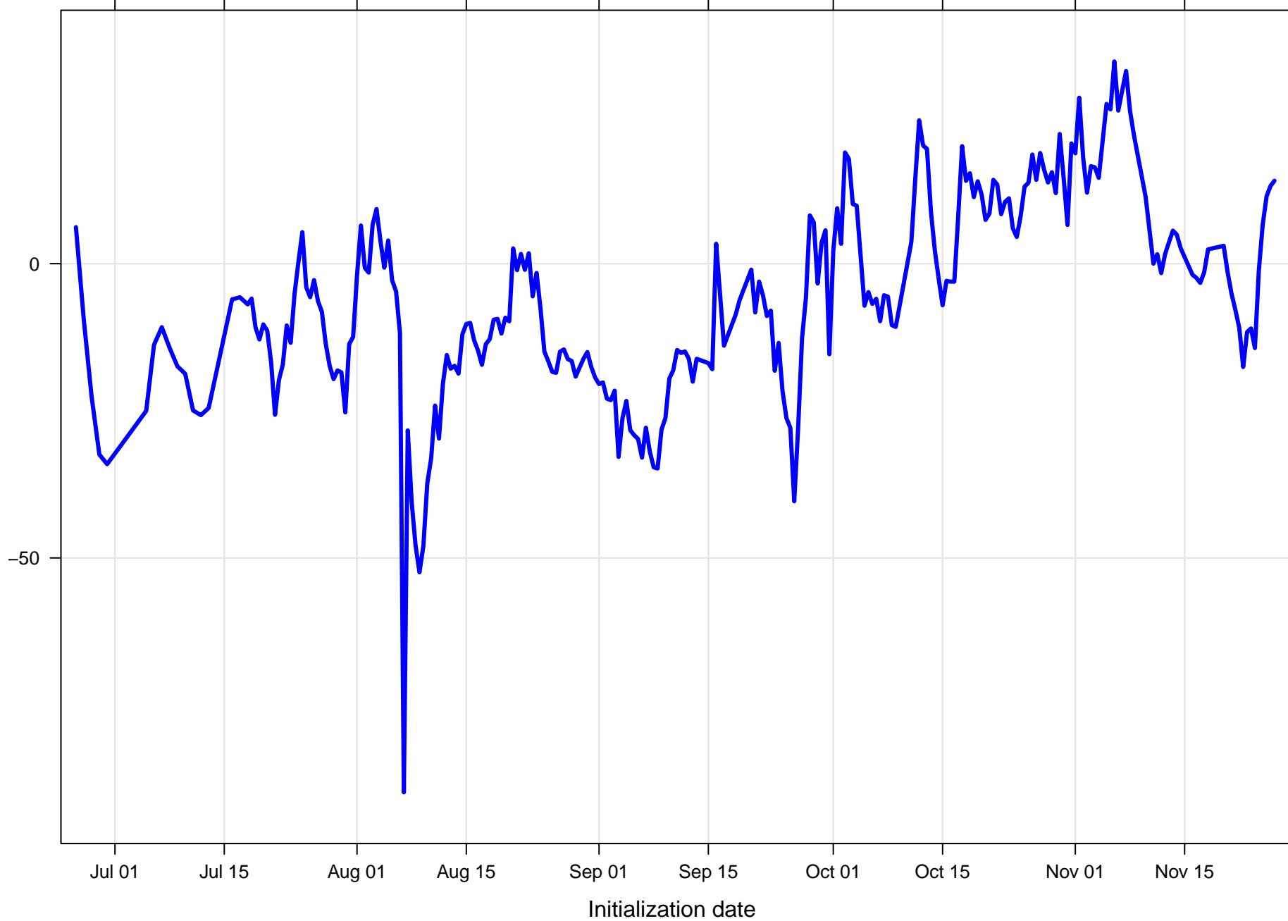
Surface wind direction bias at KEYW all forecast hours and members
