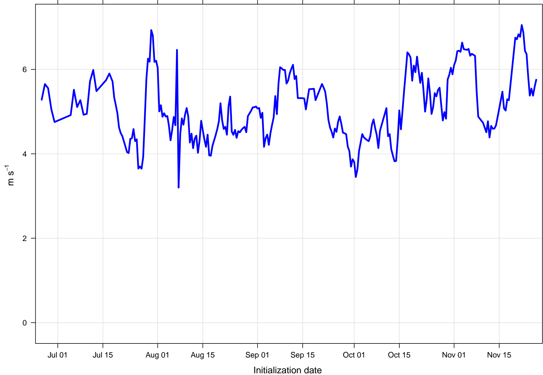
Surface vector wind RMSE at KEYW all forecast hours and members
