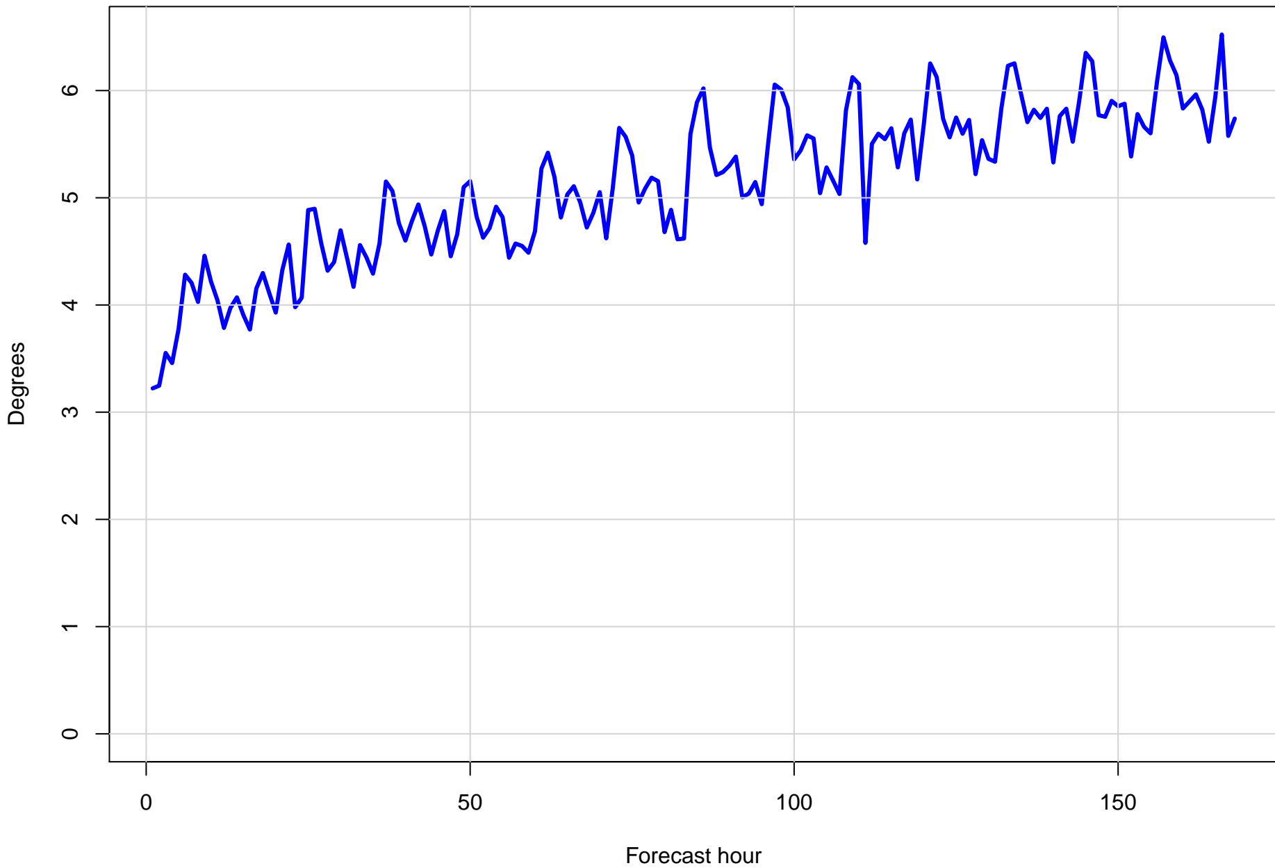
Surface vector wind RMSE at KEYW by forecast hour
