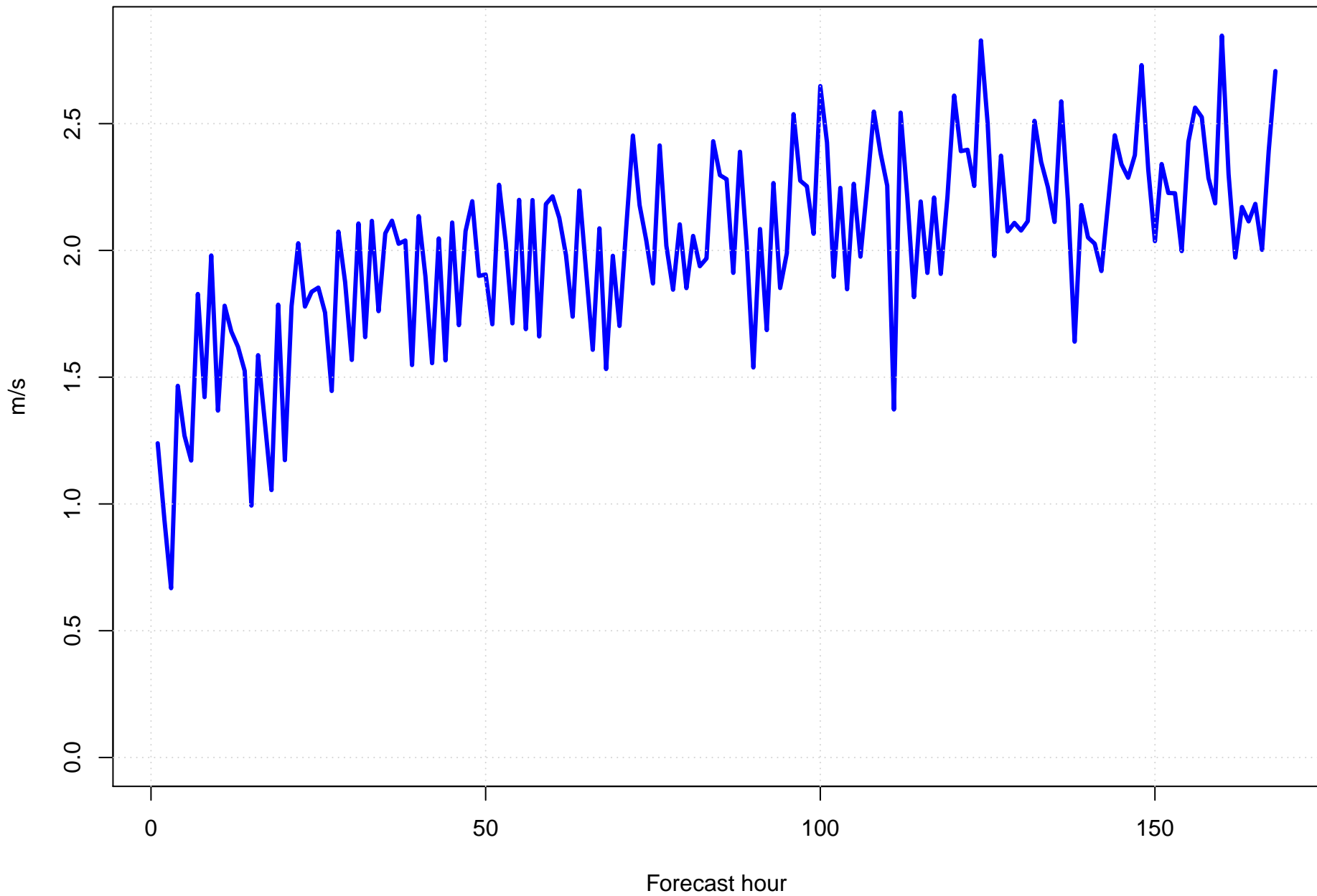
Surface wind speed bias at KEYW by forecast hour
