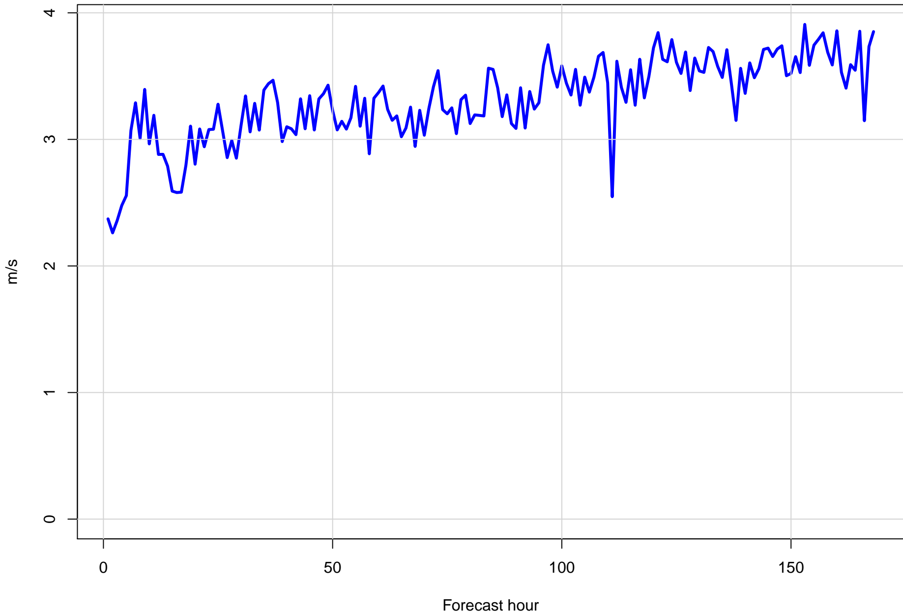
Surface wind speed RMSE at KEYW by forecast hour
