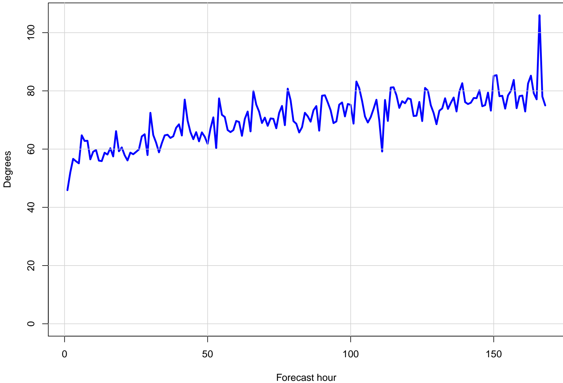
Surface wind direction RMSE at KEYW by forecast hour
