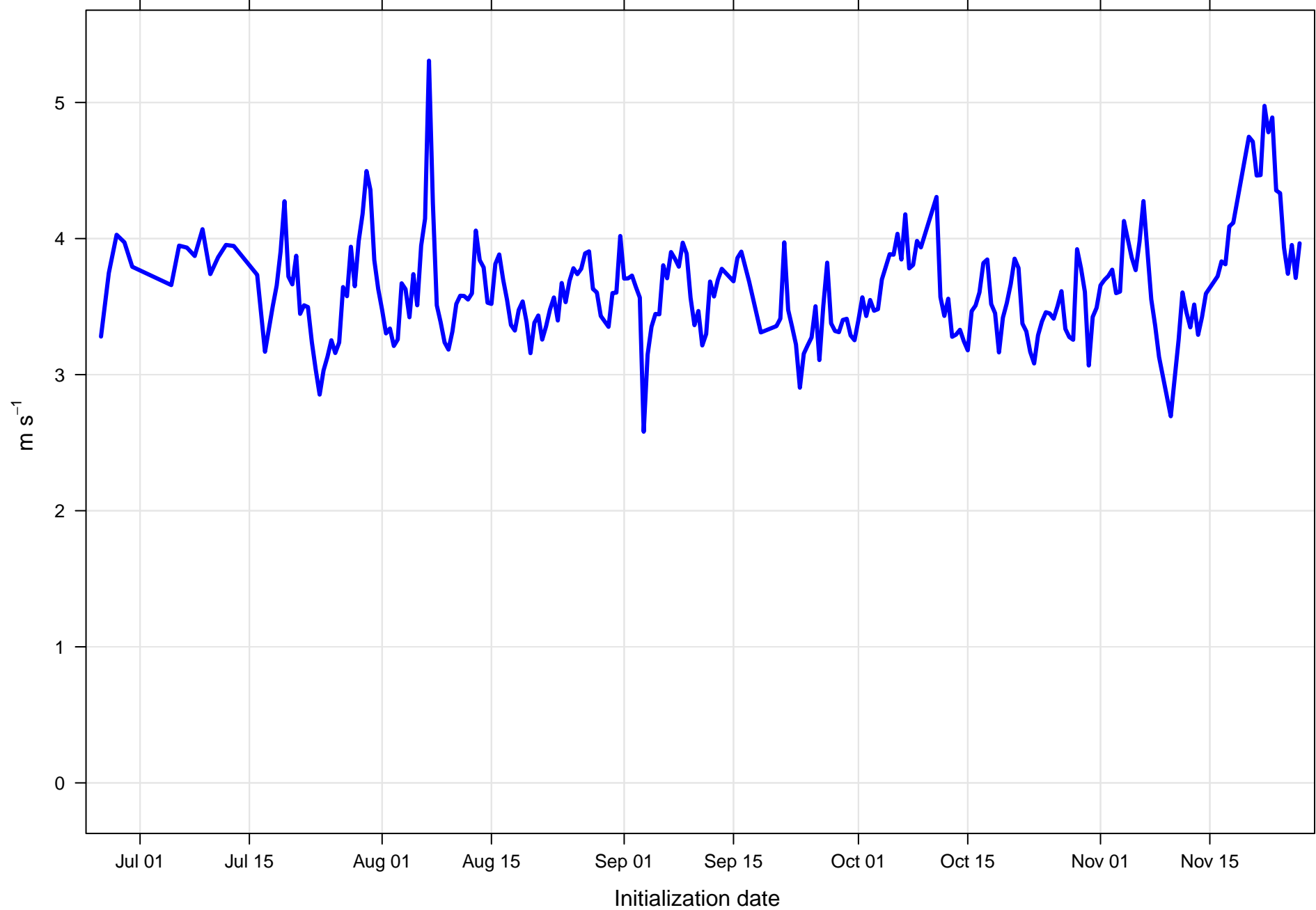
Surface vector wind RMSE at KIXA all forecast hours and members
