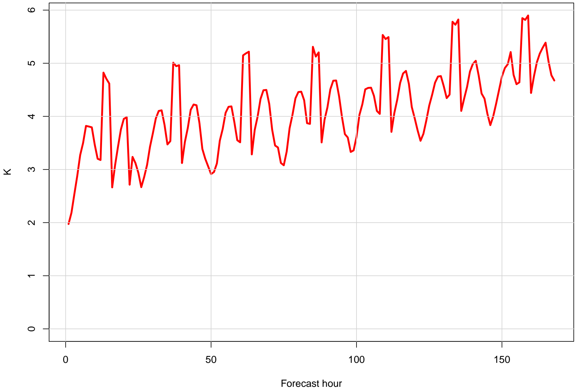
Surface temperature RMSE at KIXA by forecast hour
