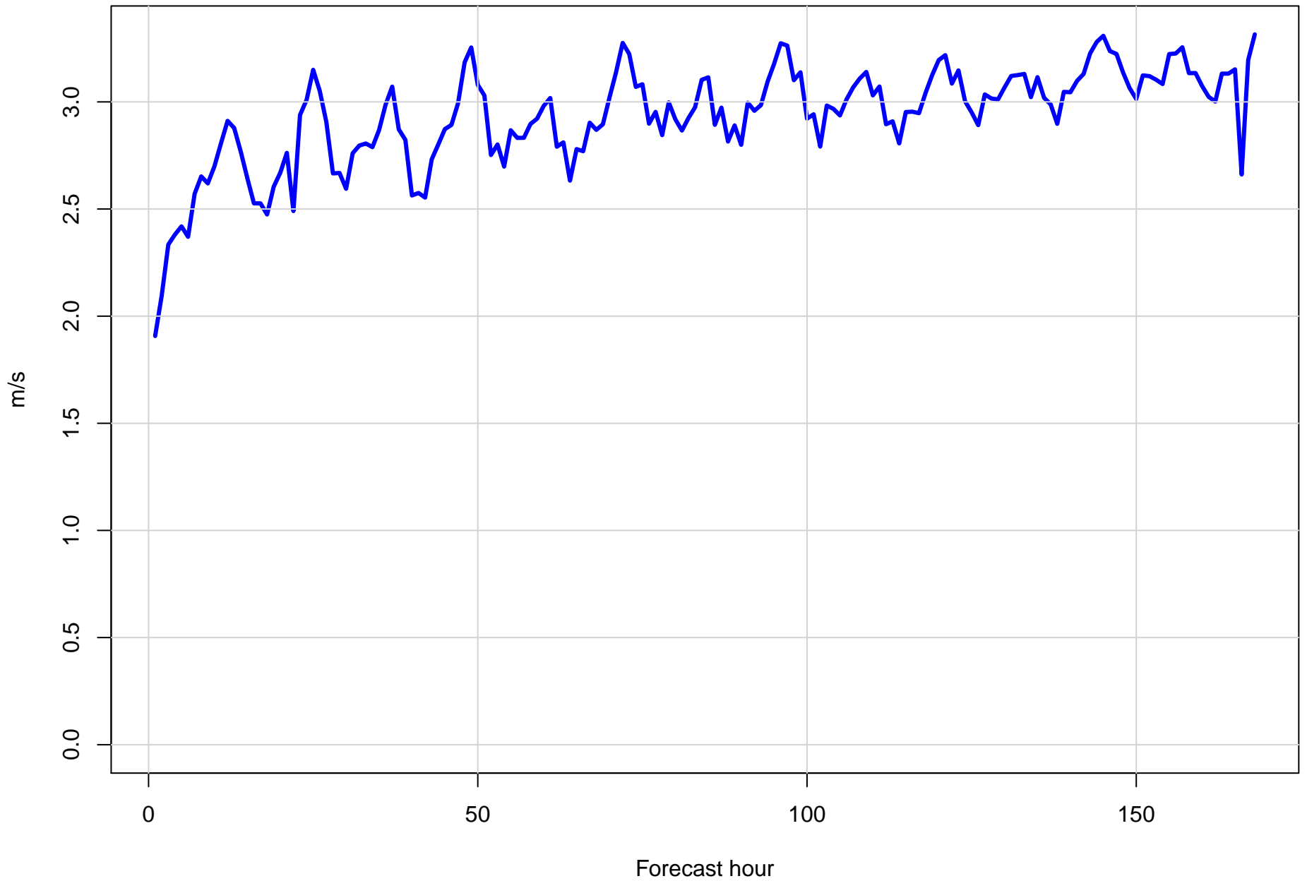
Surface wind speed RMSE at KIXA by forecast hour
