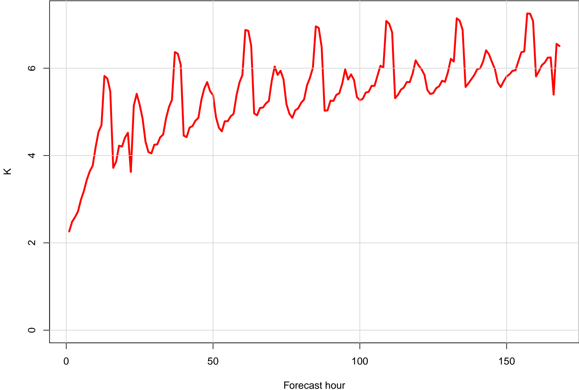
Surface dew point RMSE at KIXA by forecast hour
