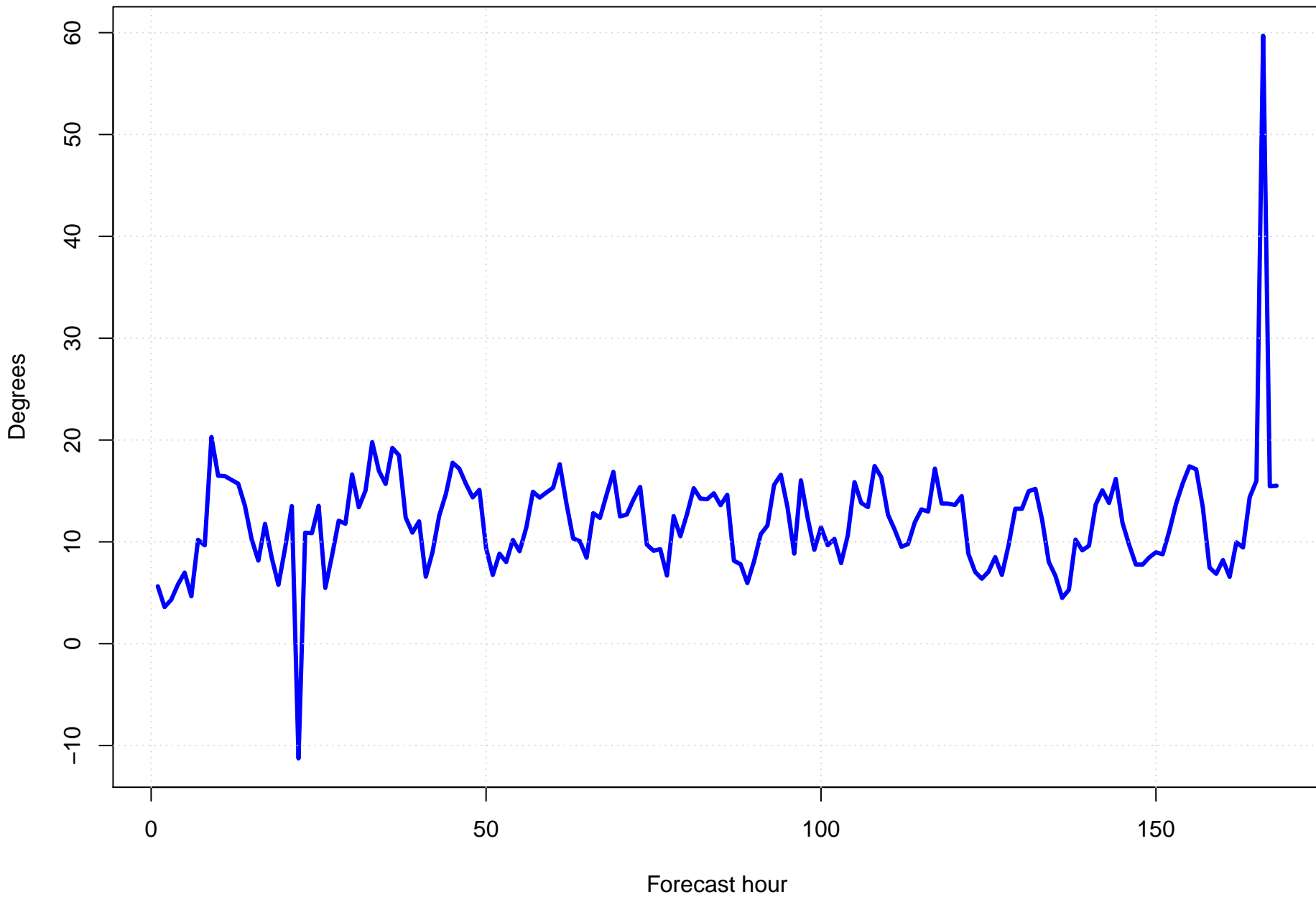
Surface wind direction bias at KIXA by forecast hour
