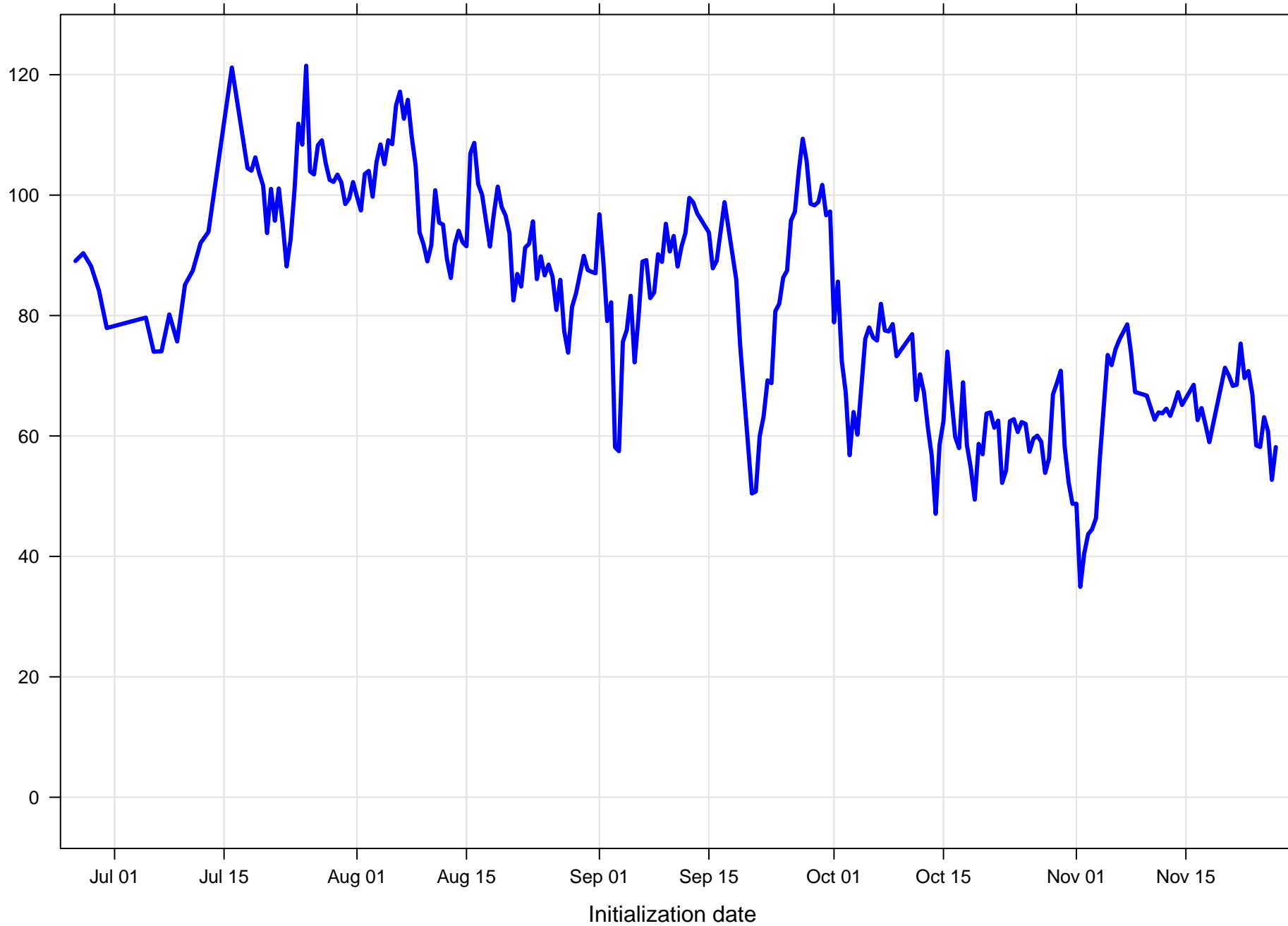
Surface wind direction RMSE at KIXA all forecast hours and members
