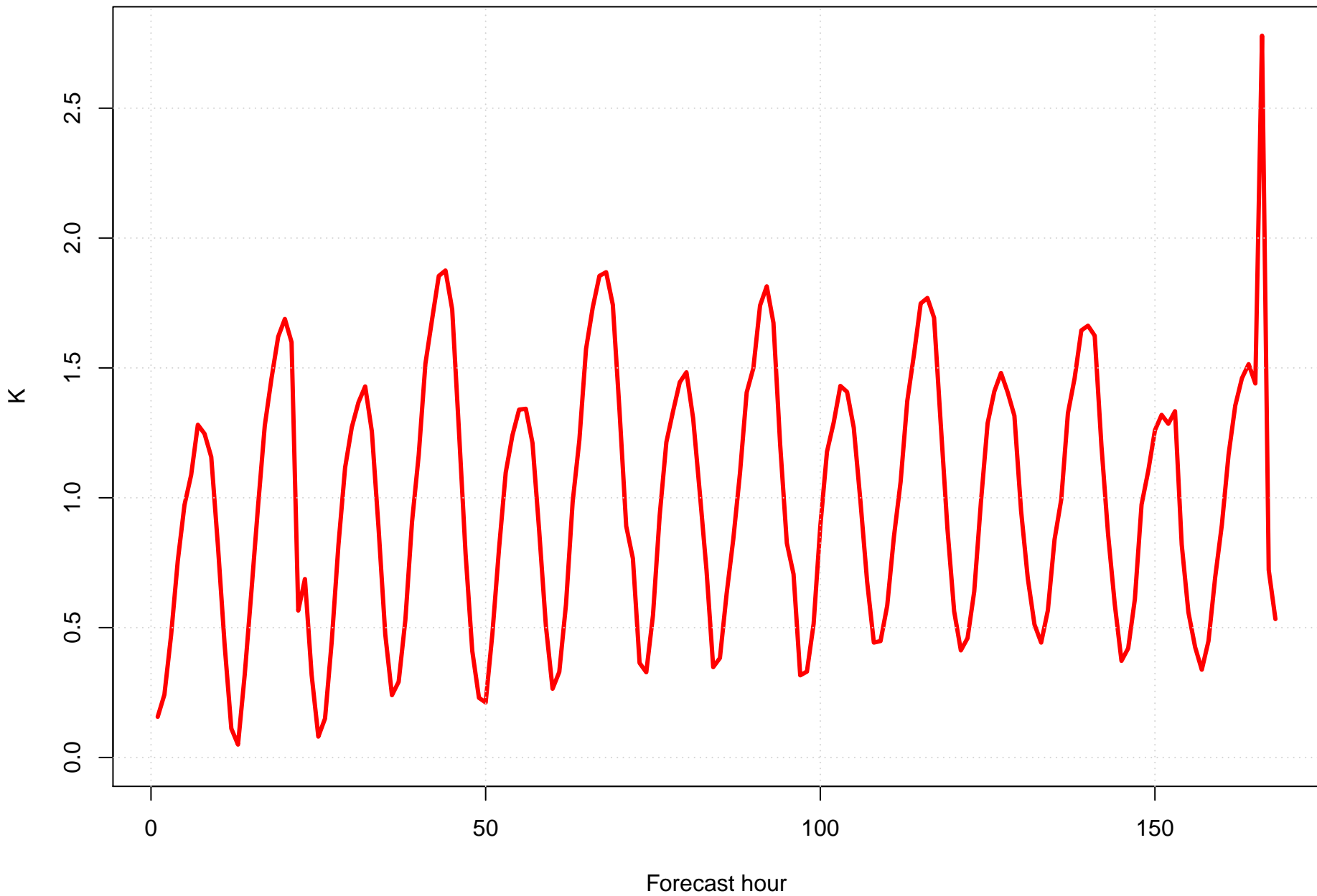
Surface temperature bias at KIXA by forecast hour
