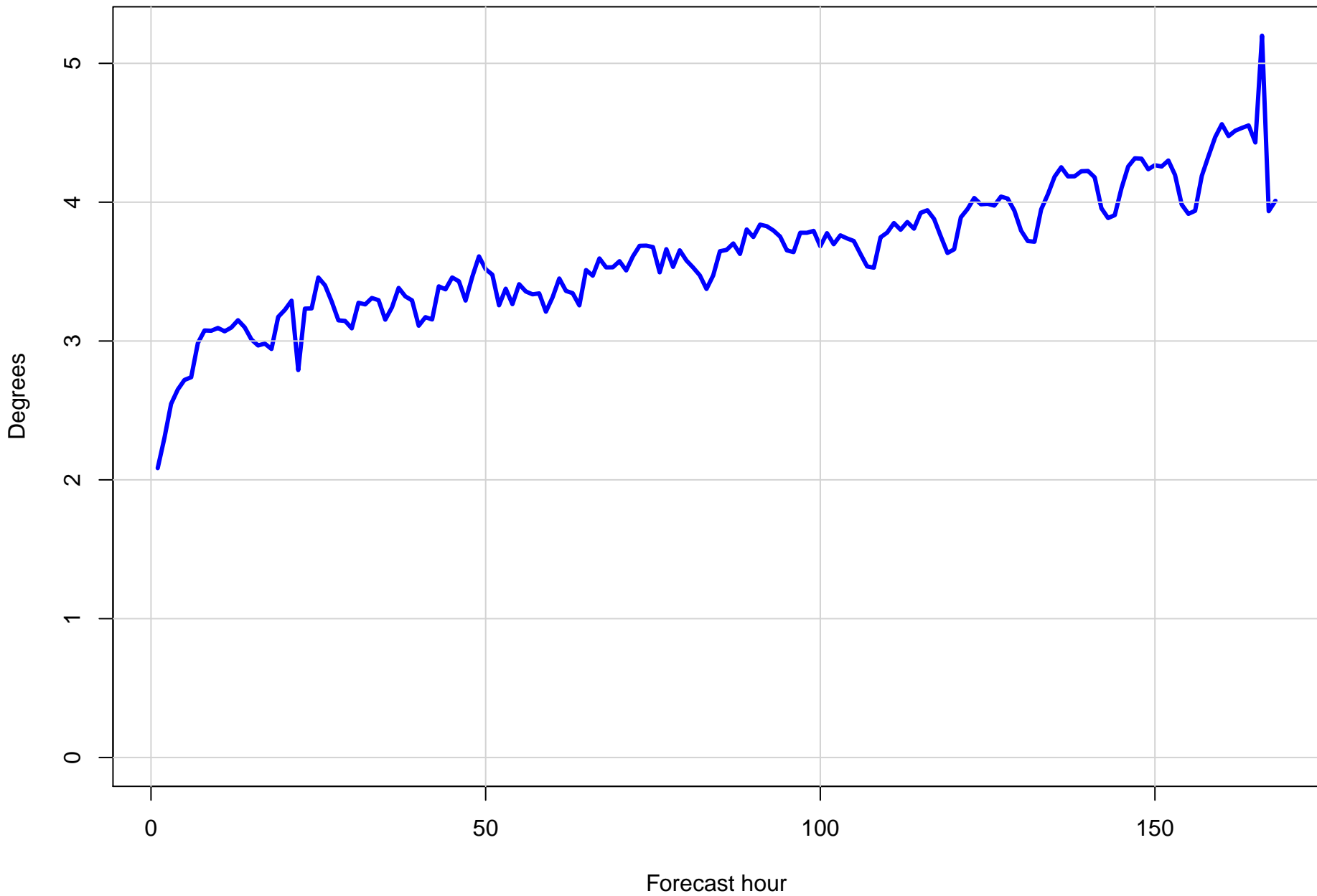
Surface vector wind RMSE at KIXA by forecast hour
