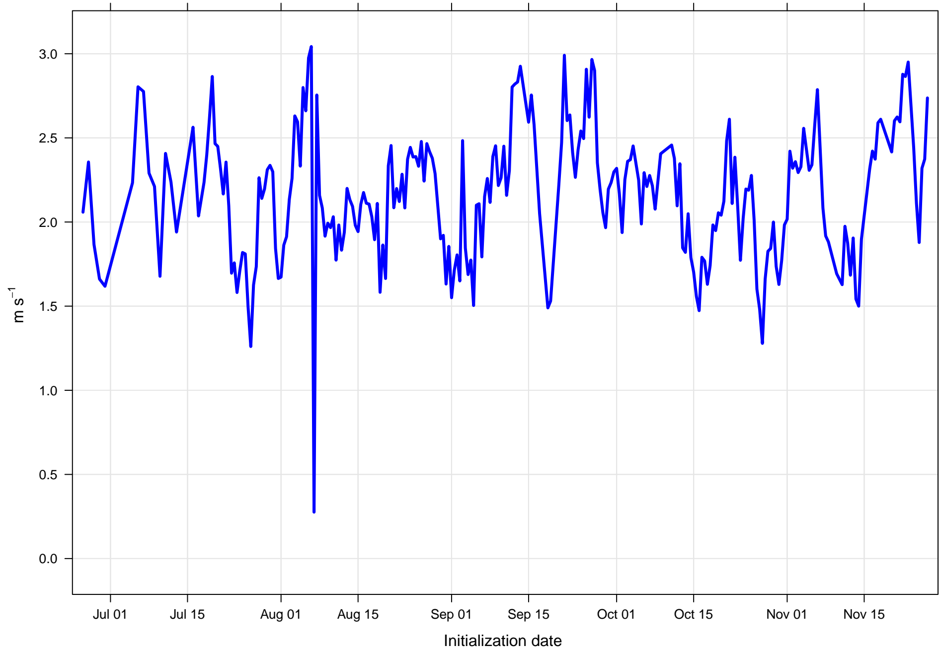
Surface wind speed bias at KIXA all forecast hours and members
