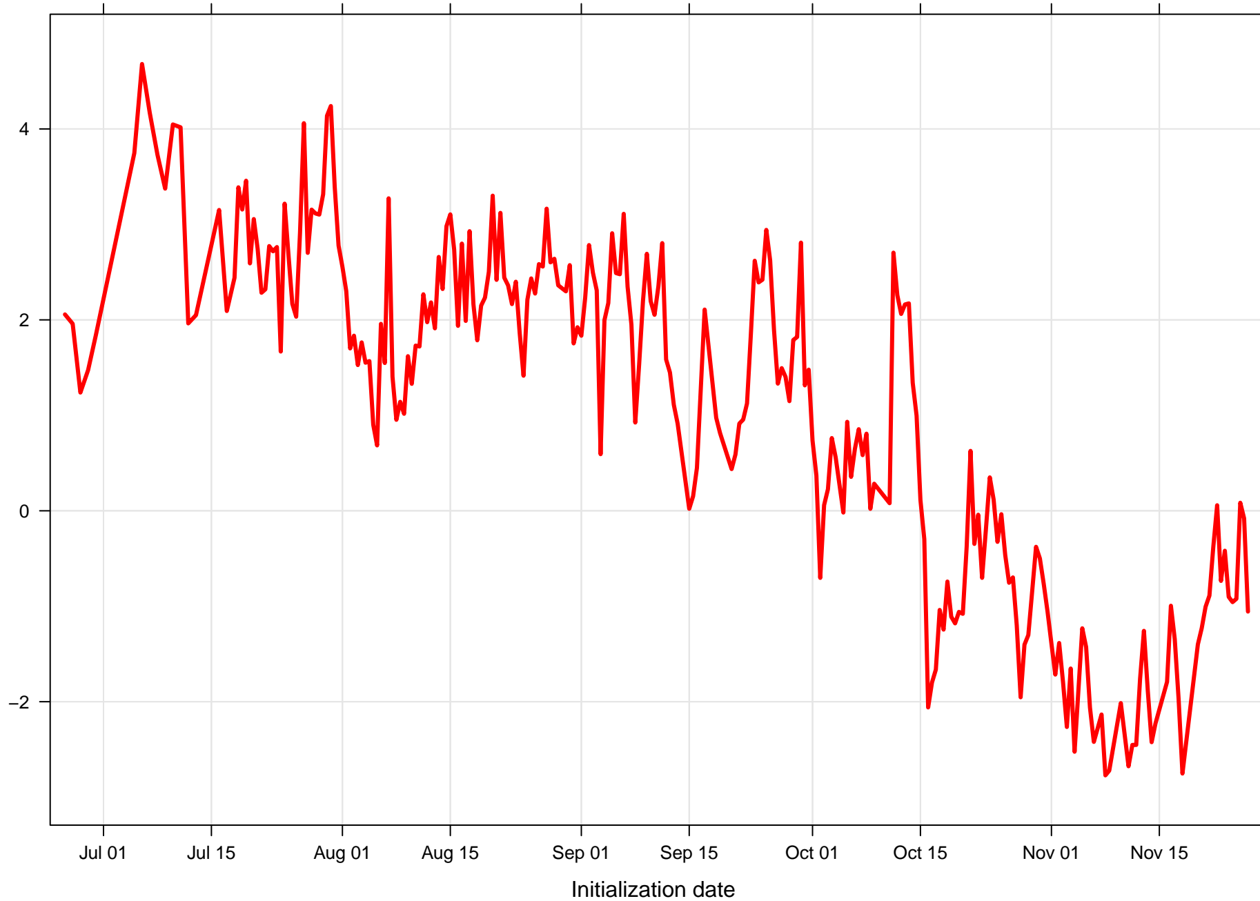
Surface temperature bias at KIXA all forecast hours and members
