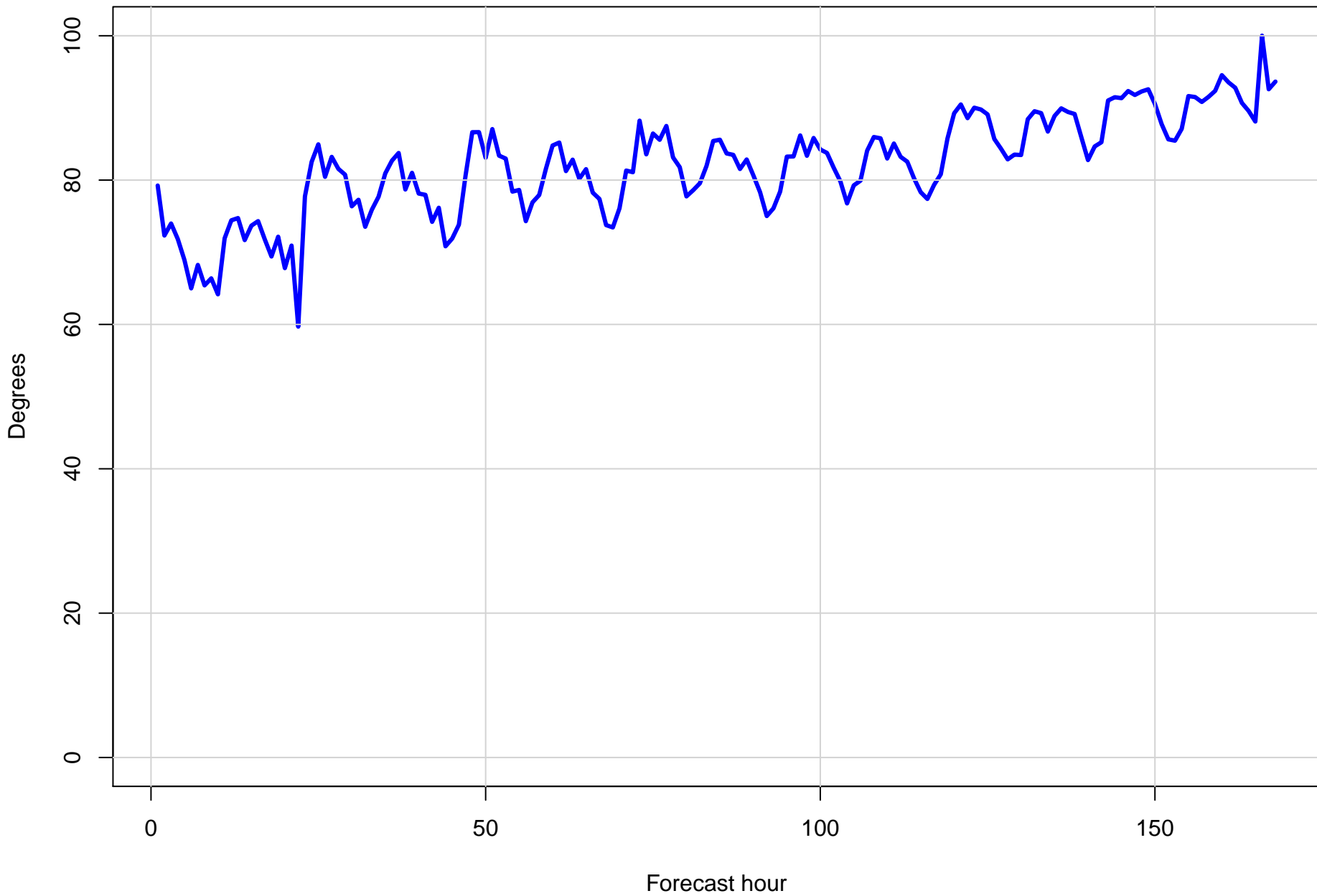
Surface wind direction RMSE at KIXA by forecast hour
