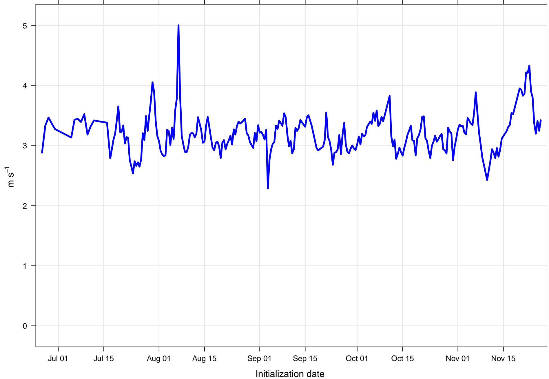
Surface vector wind mean error KIXA all forecast hours and members
