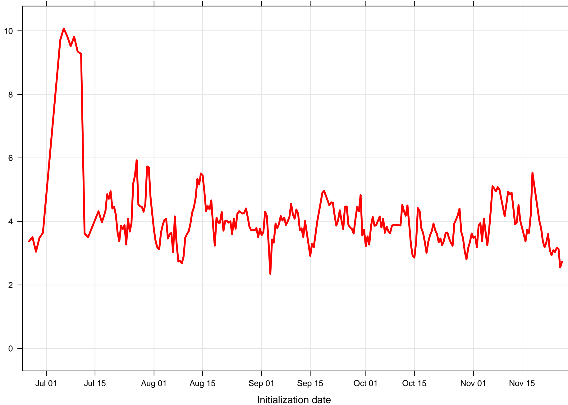
Surface temperature RMSE at KIXA all forecast hours and members
