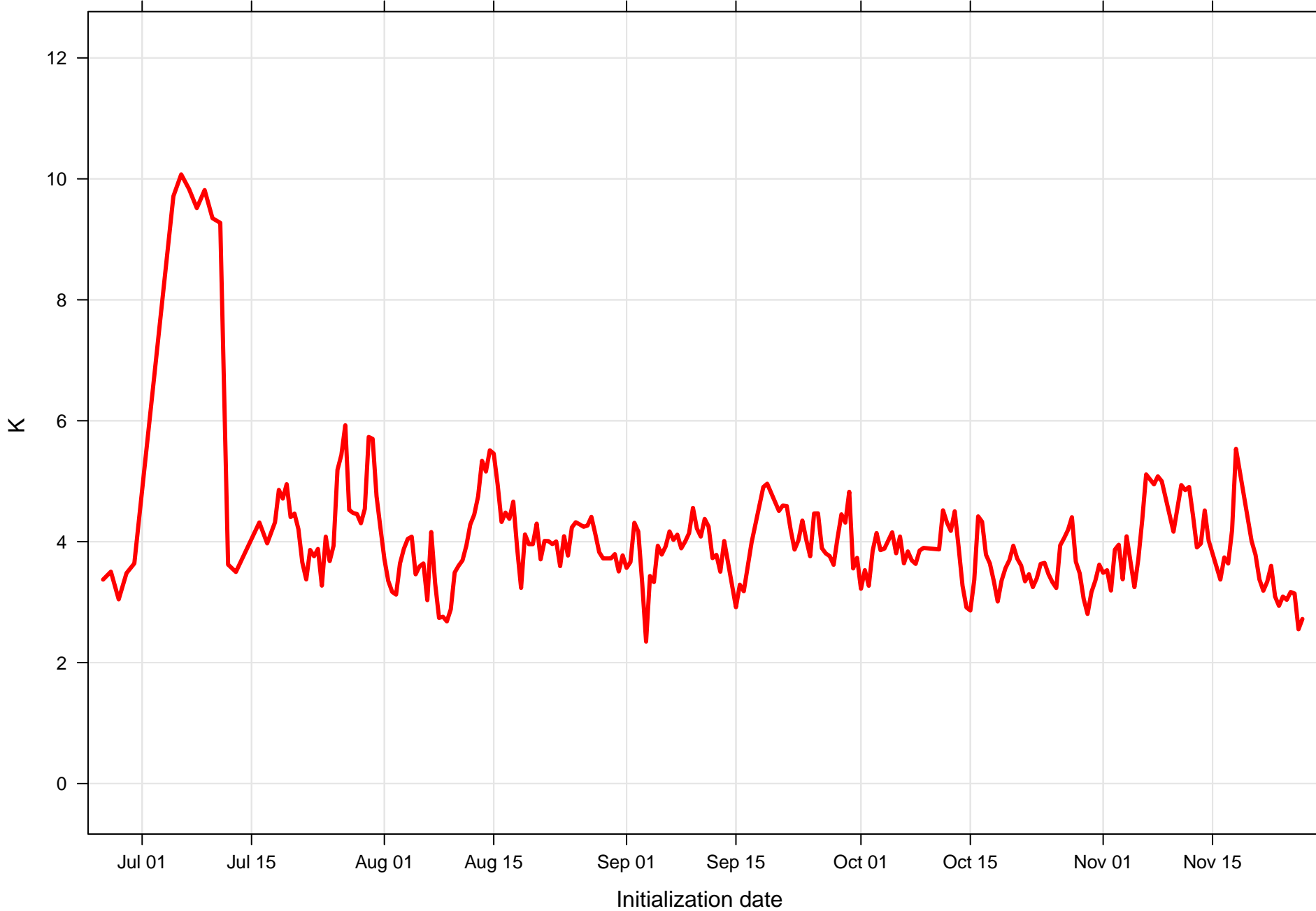
Surface dew point RMSE at KIXA all forecast hours and members
