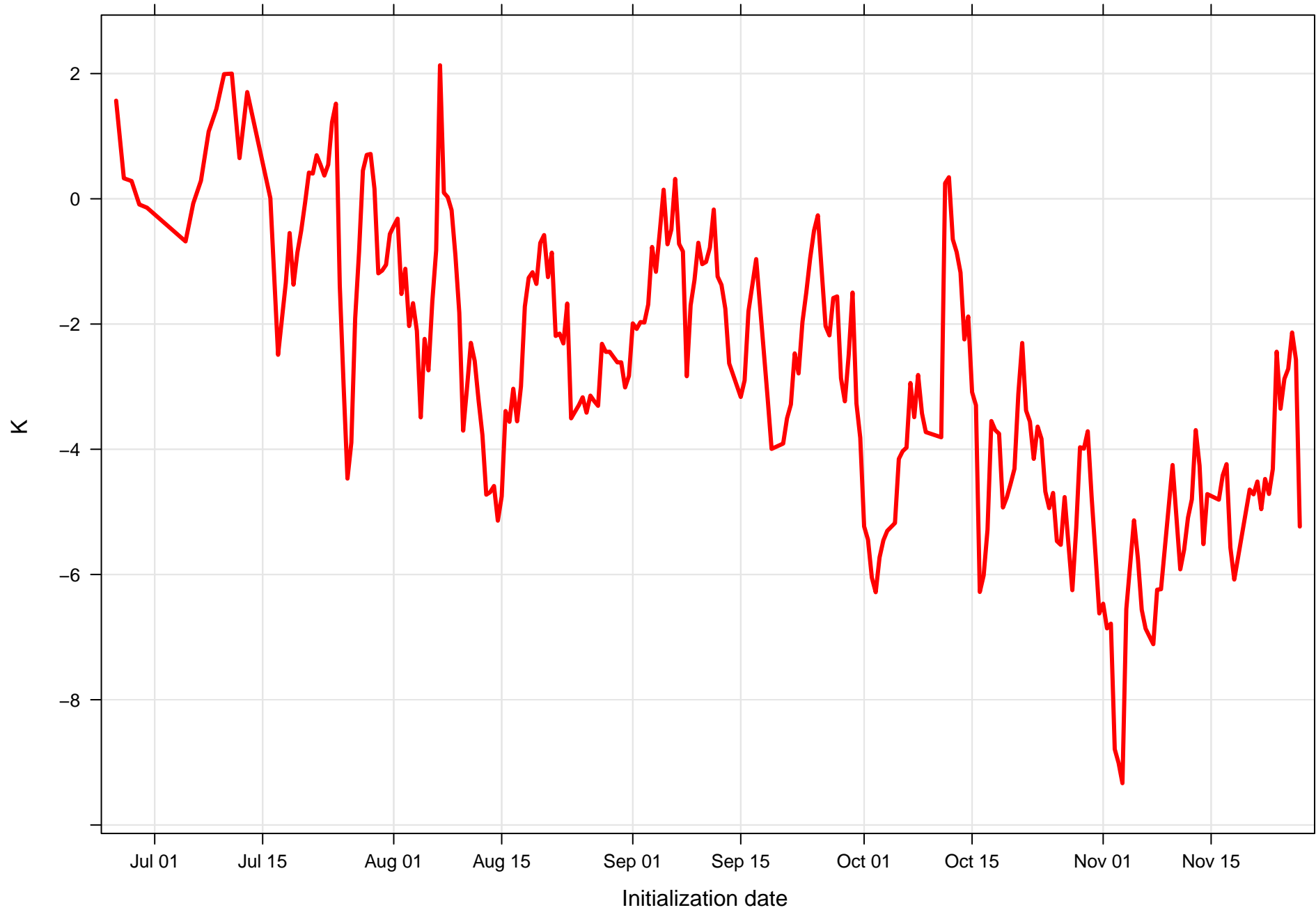
Surface dew point bias at KIXA all forecast hours and members
