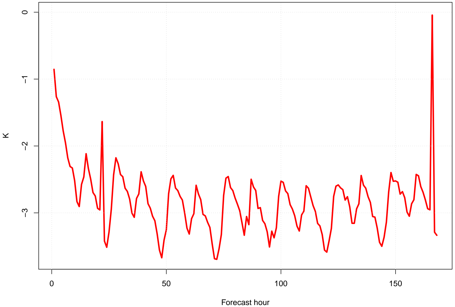
Surface dew point bias at KIXA by forecast hour
