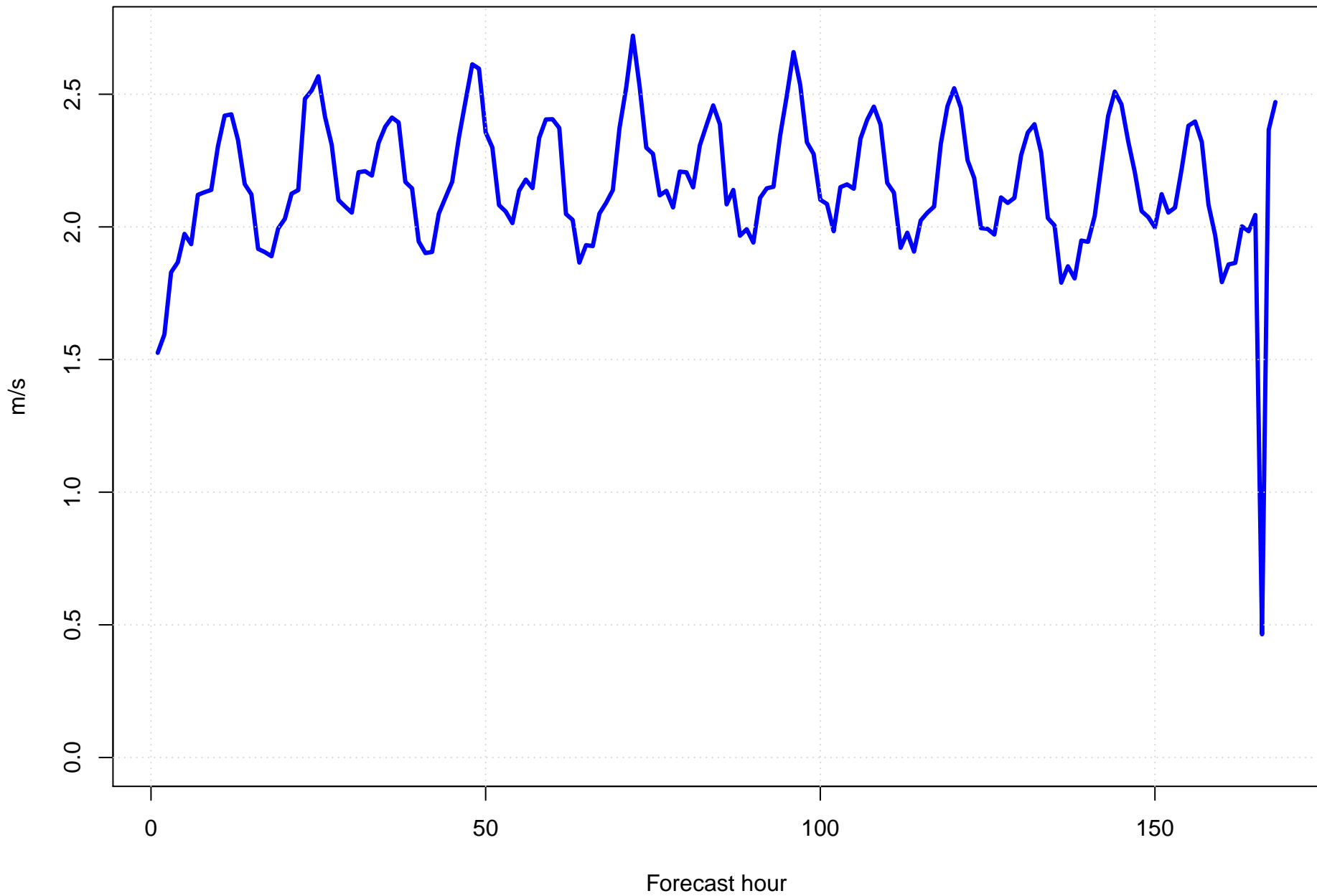
Surface wind speed bias at KIXA by forecast hour
