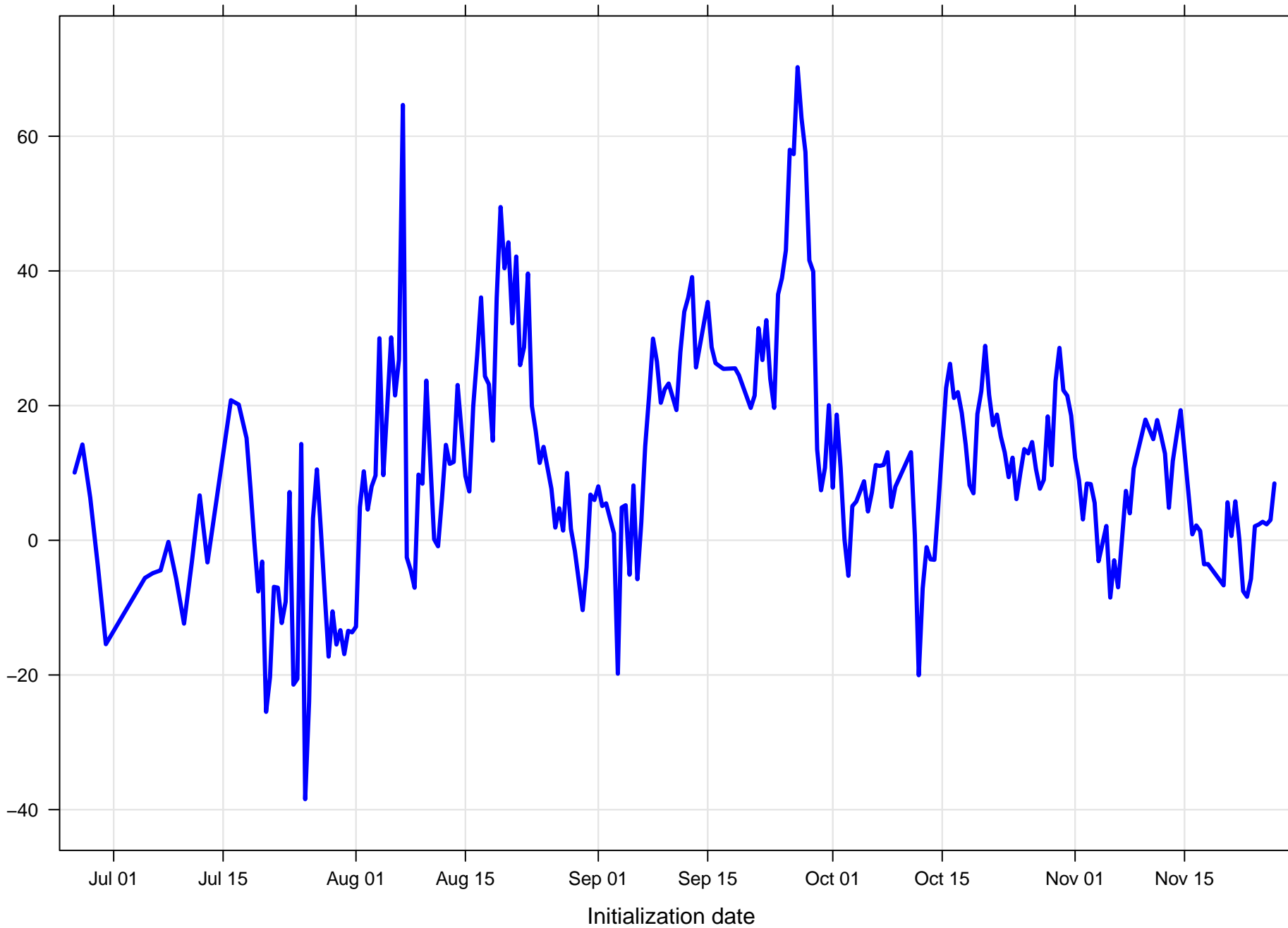
Surface wind direction bias at KIXA all forecast hours and members
