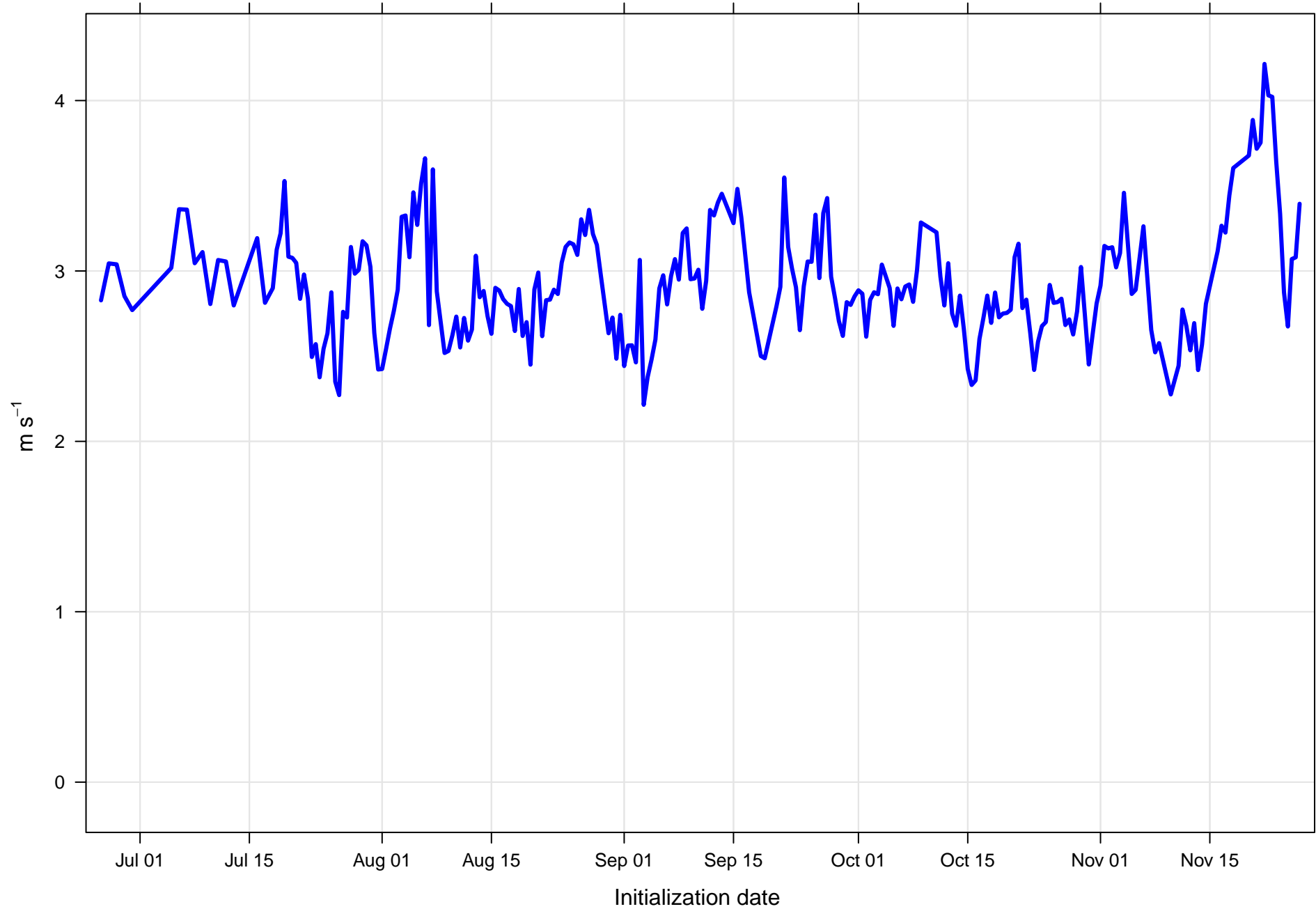
Surface wind speed RMSE at KIXA all forecast hours and members
