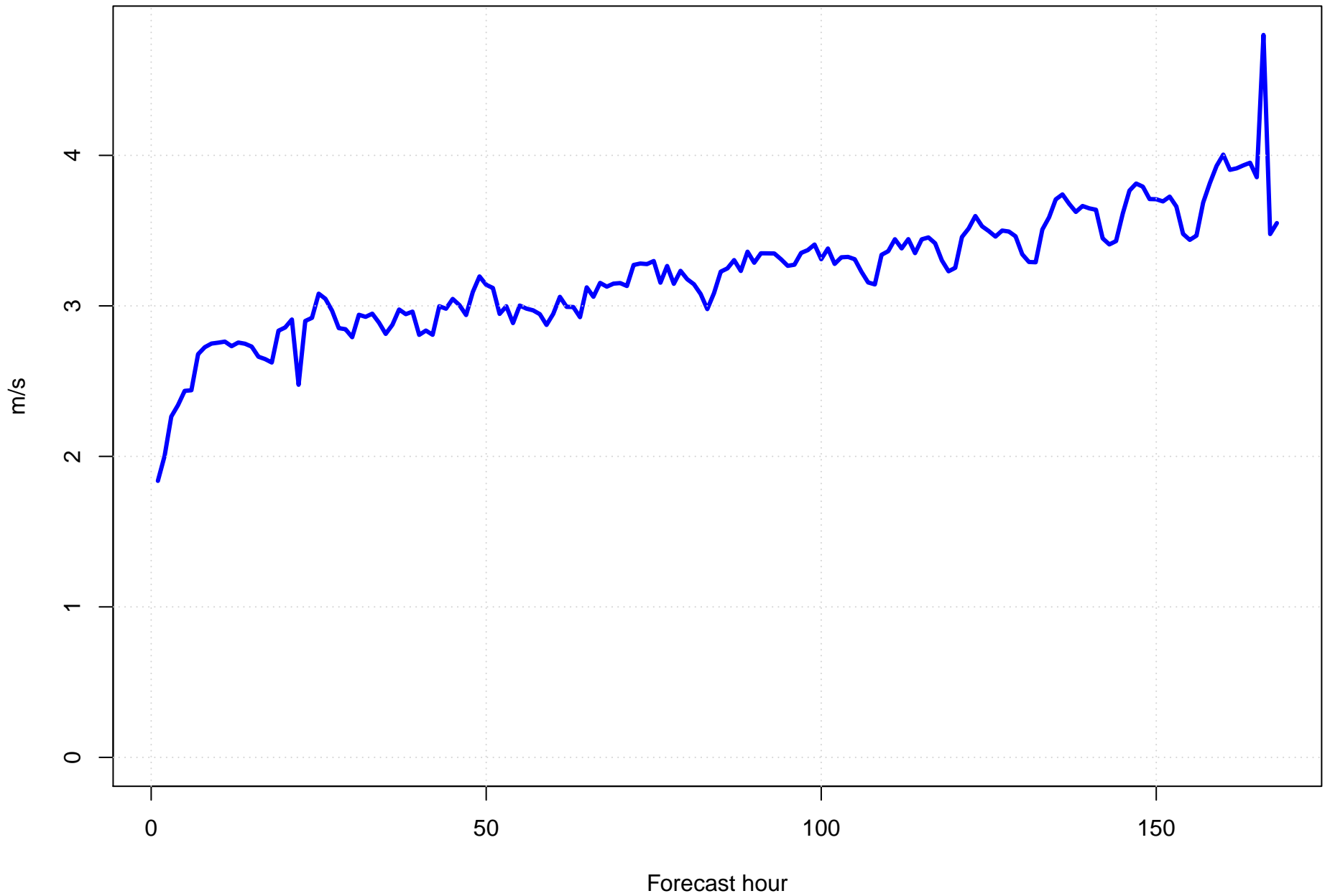
Surface vector wind error at KIXA by forecast hour
