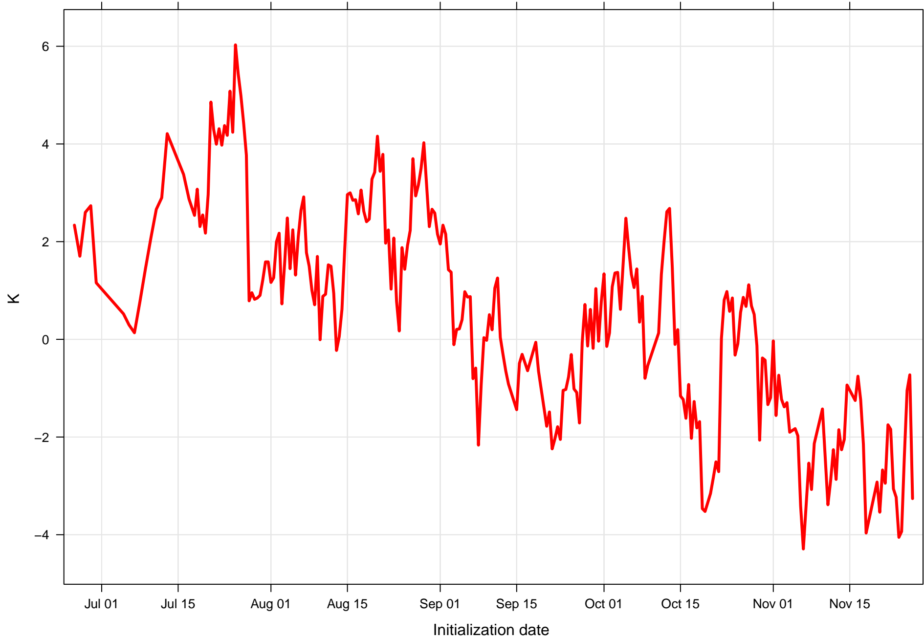
Surface temperature bias at KJKL all forecast hours and members
