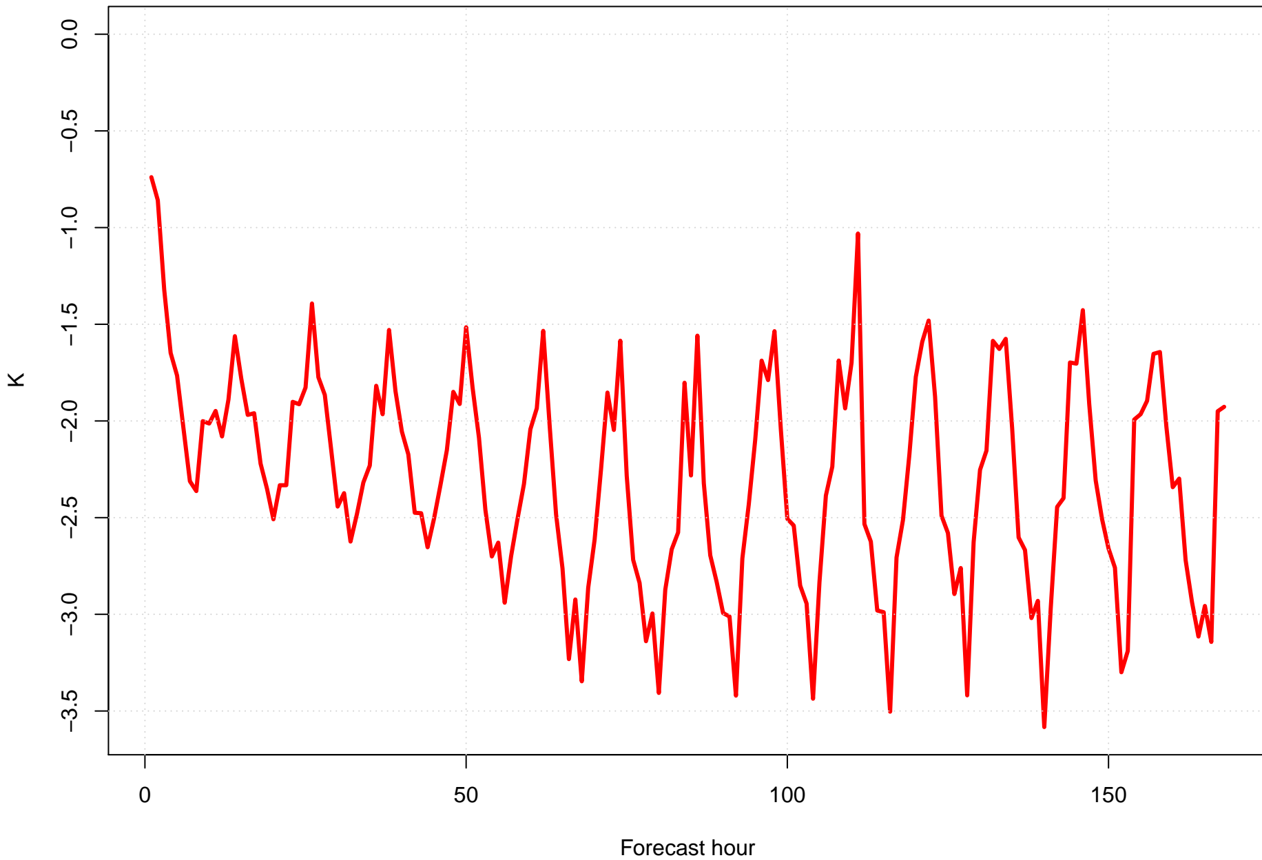
Surface dew point bias at KMCO by forecast hour
