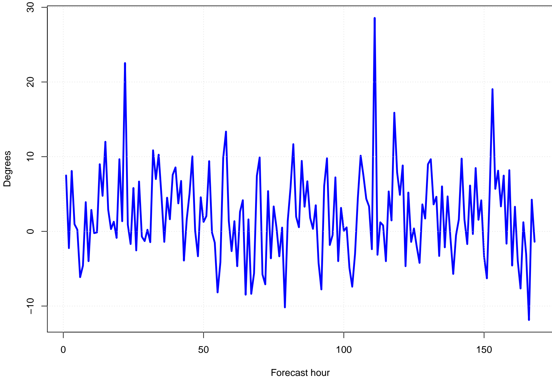
Surface wind direction bias at KMCO by forecast hour
