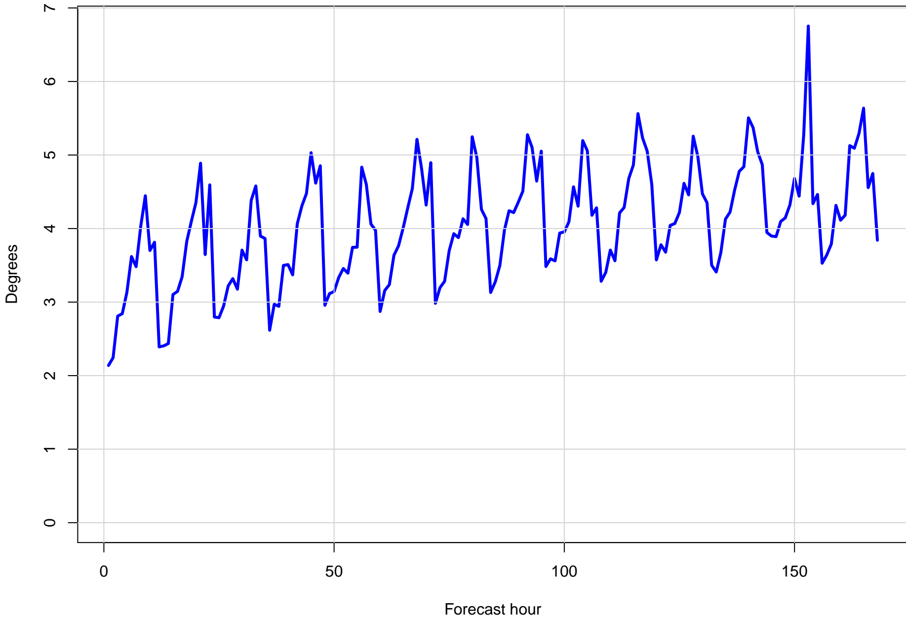
Surface vector wind RMSE at KMCO by forecast hour
