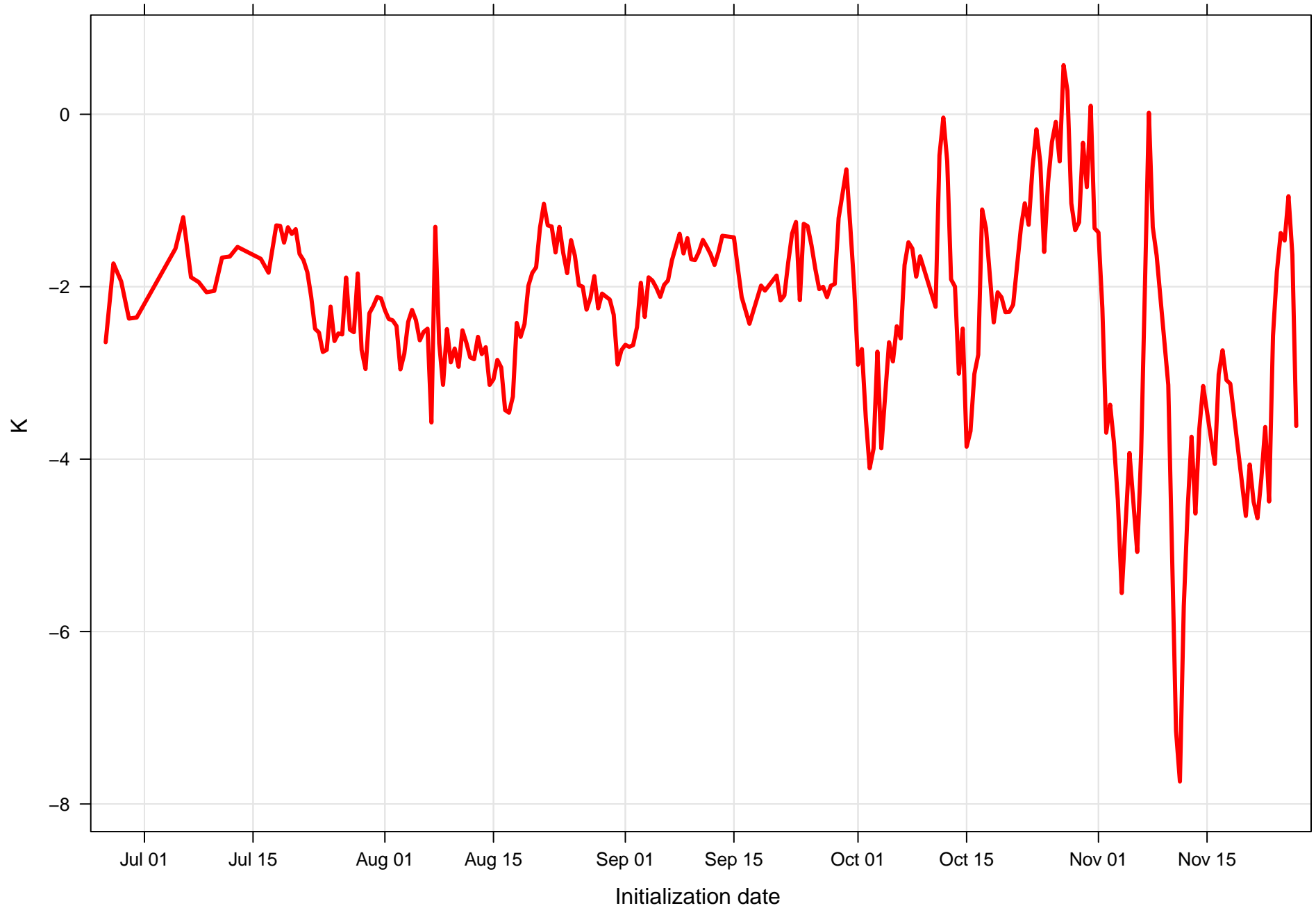
Surface dew point bias at KMCO all forecast hours and members
