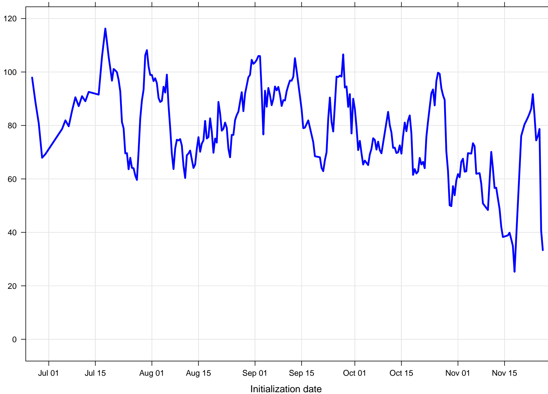
Surface wind direction RMSE at KMCO all forecast hours and members
