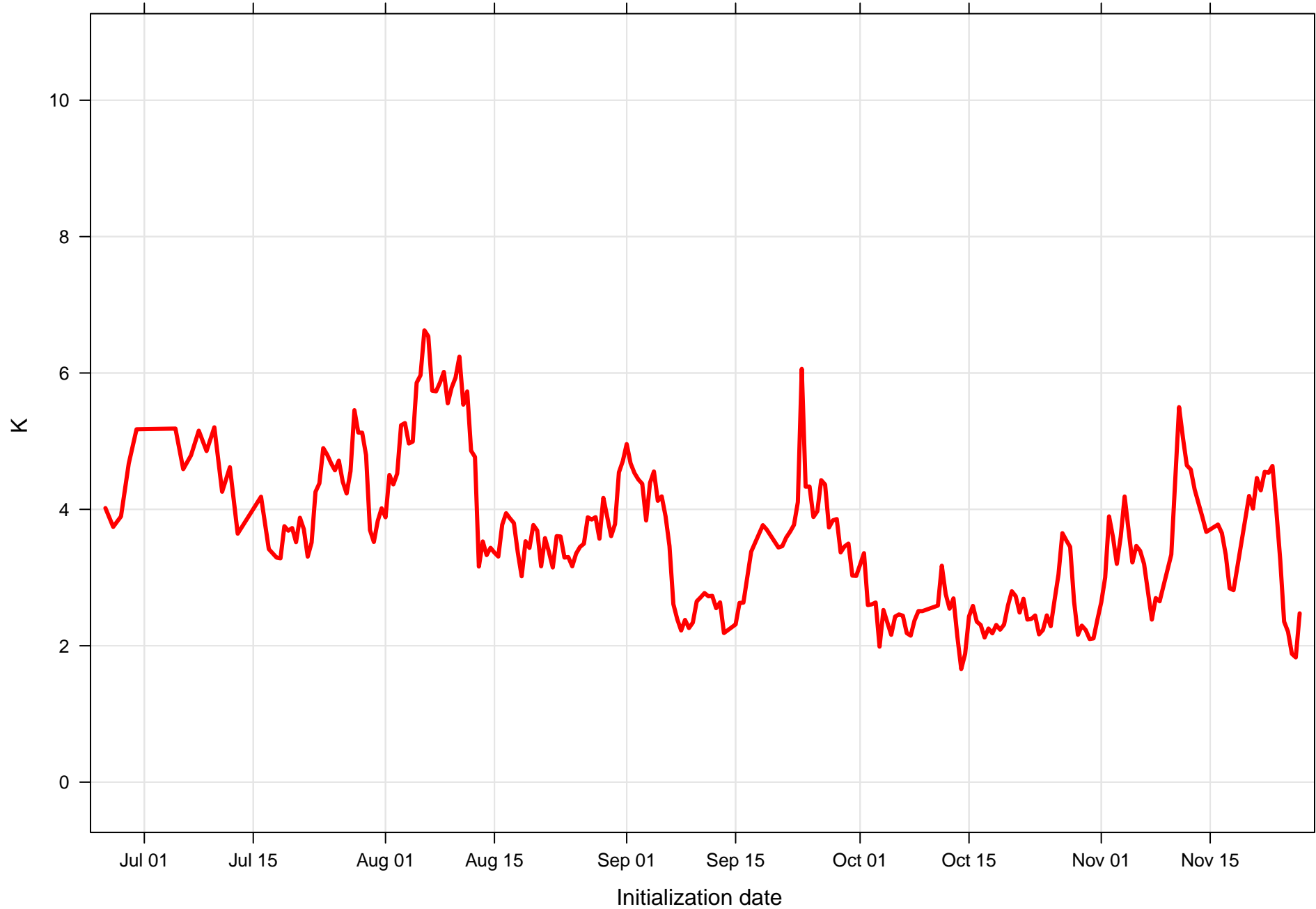
Surface dew point RMSE at KMCO all forecast hours and members
