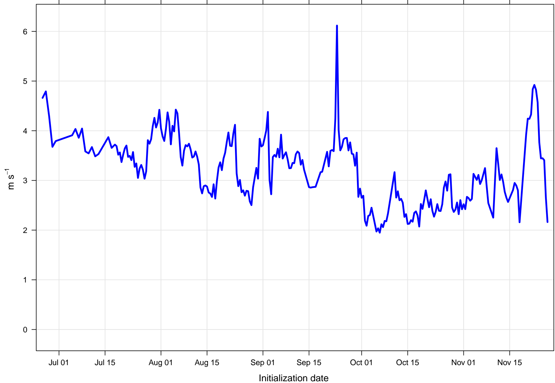
Surface vector wind mean error KMCO all forecast hours and members
