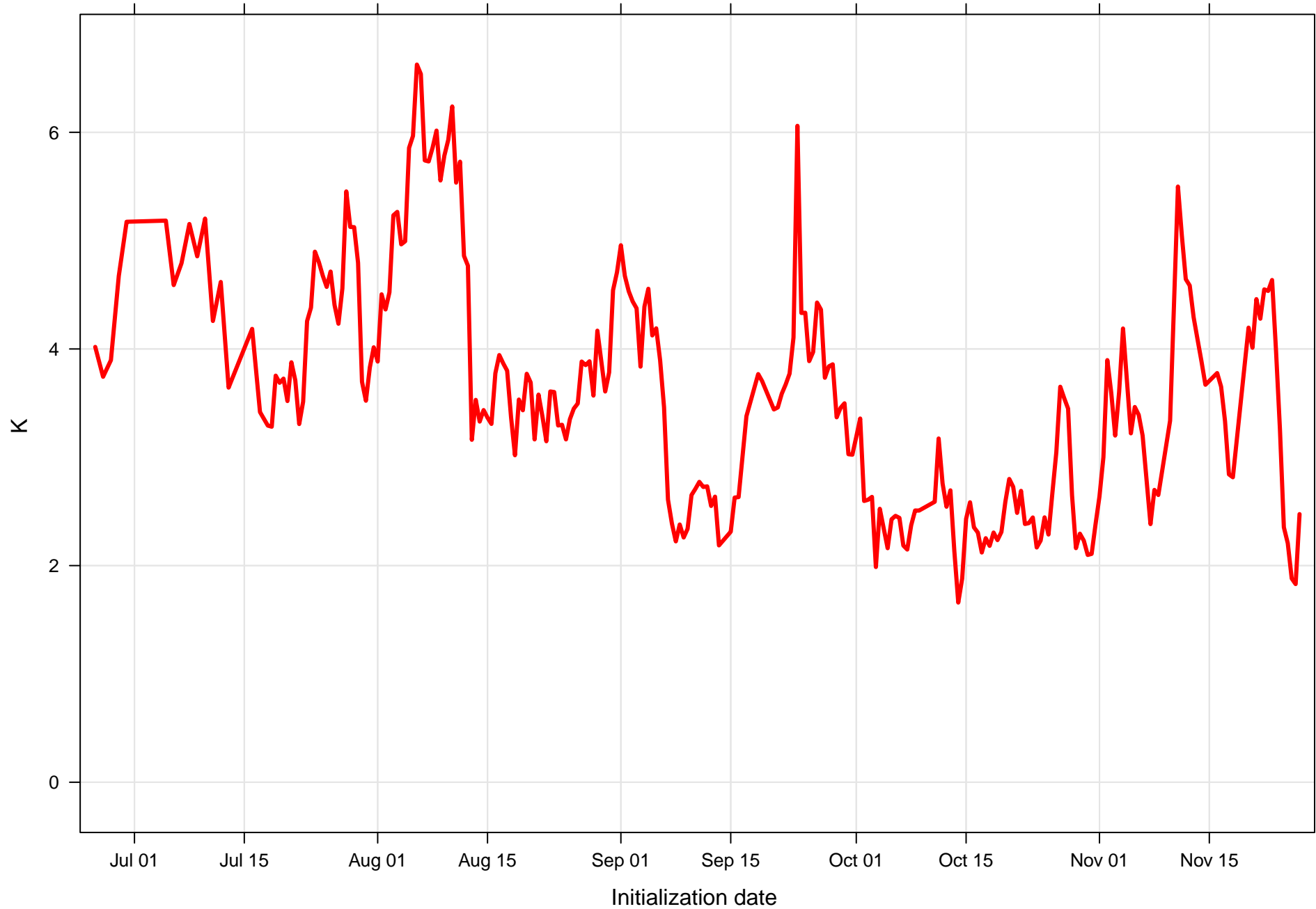
Surface temperature RMSE at KMCO all forecast hours and members
