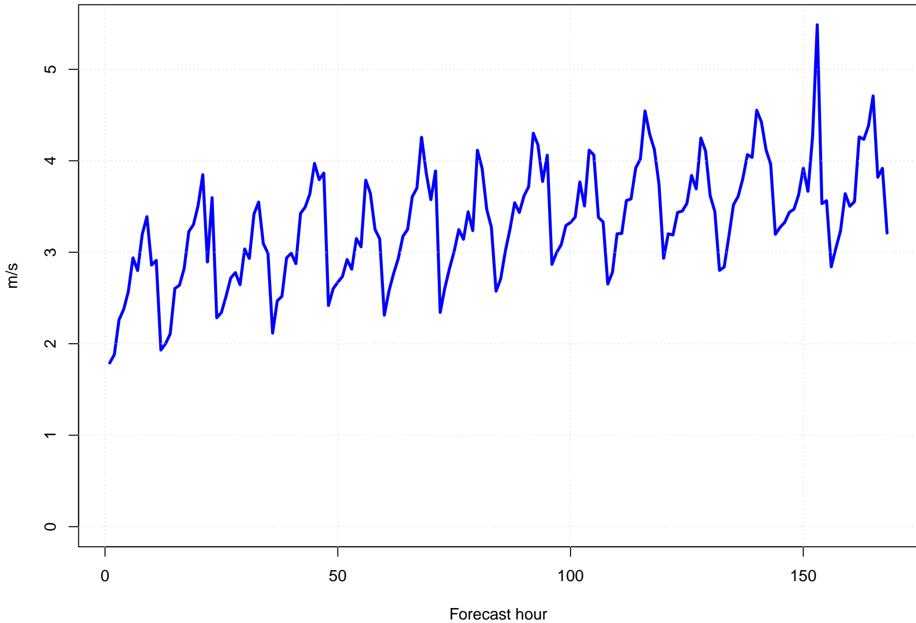
Surface vector wind error at KMCO by forecast hour
