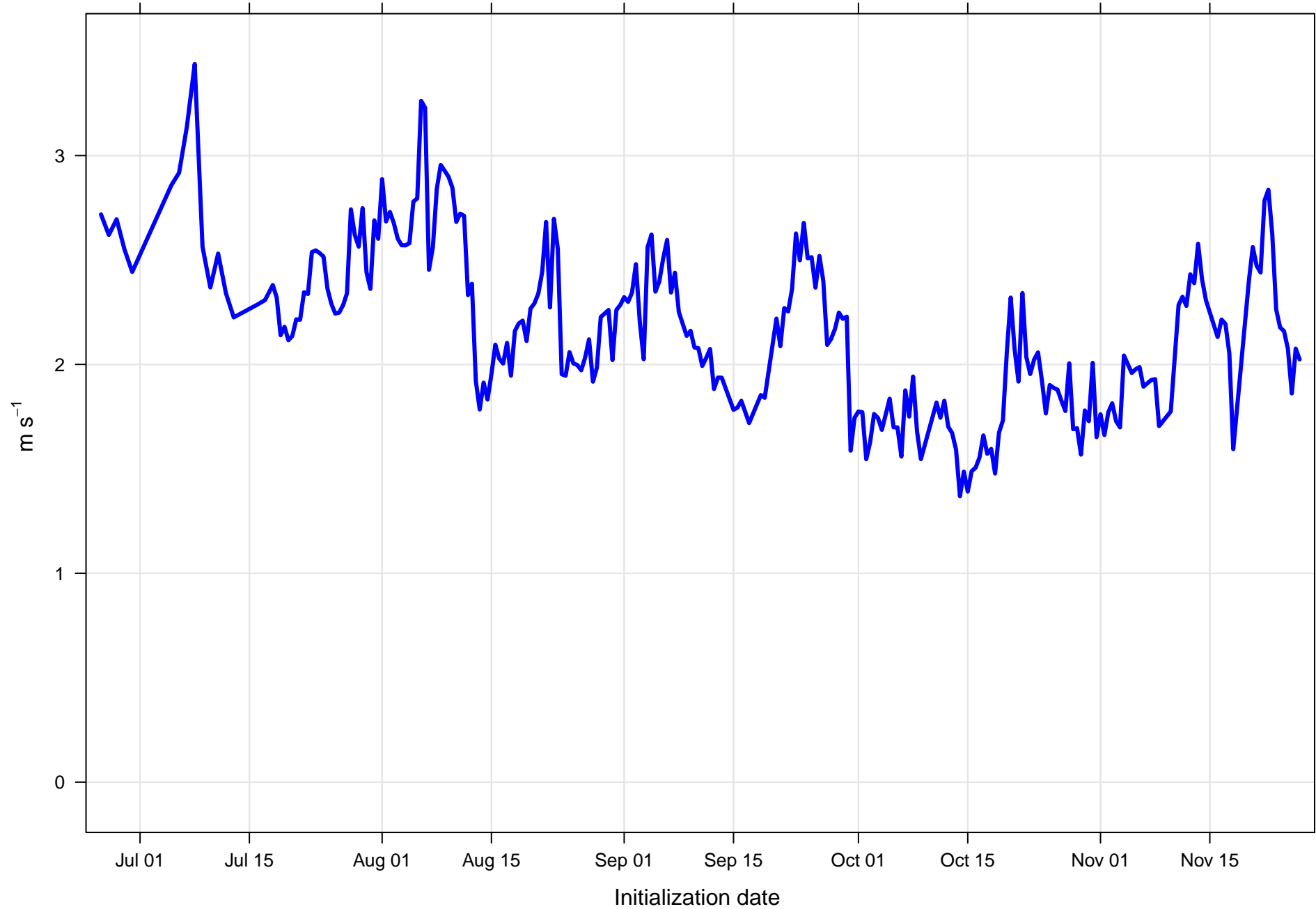
Surface wind speed RMSE at KMCO all forecast hours and members
