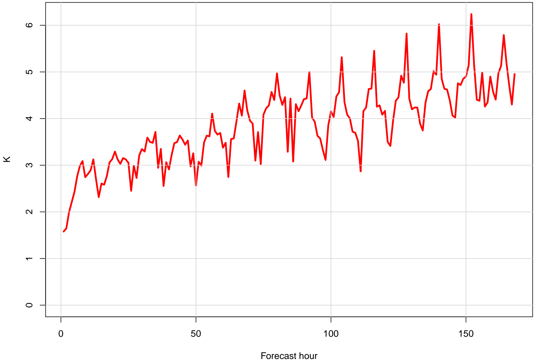
Surface dew point RMSE at KMCO by forecast hour
