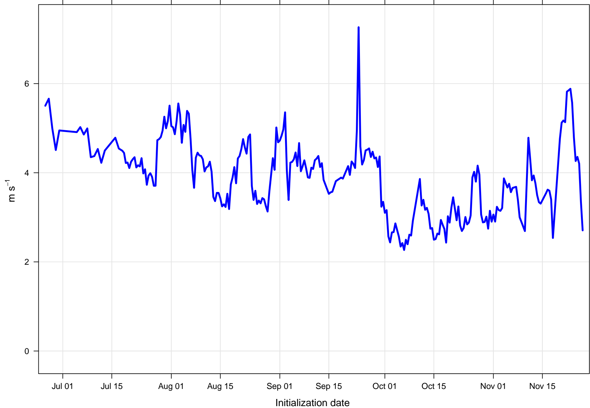
Surface vector wind RMSE at KMCO all forecast hours and members
