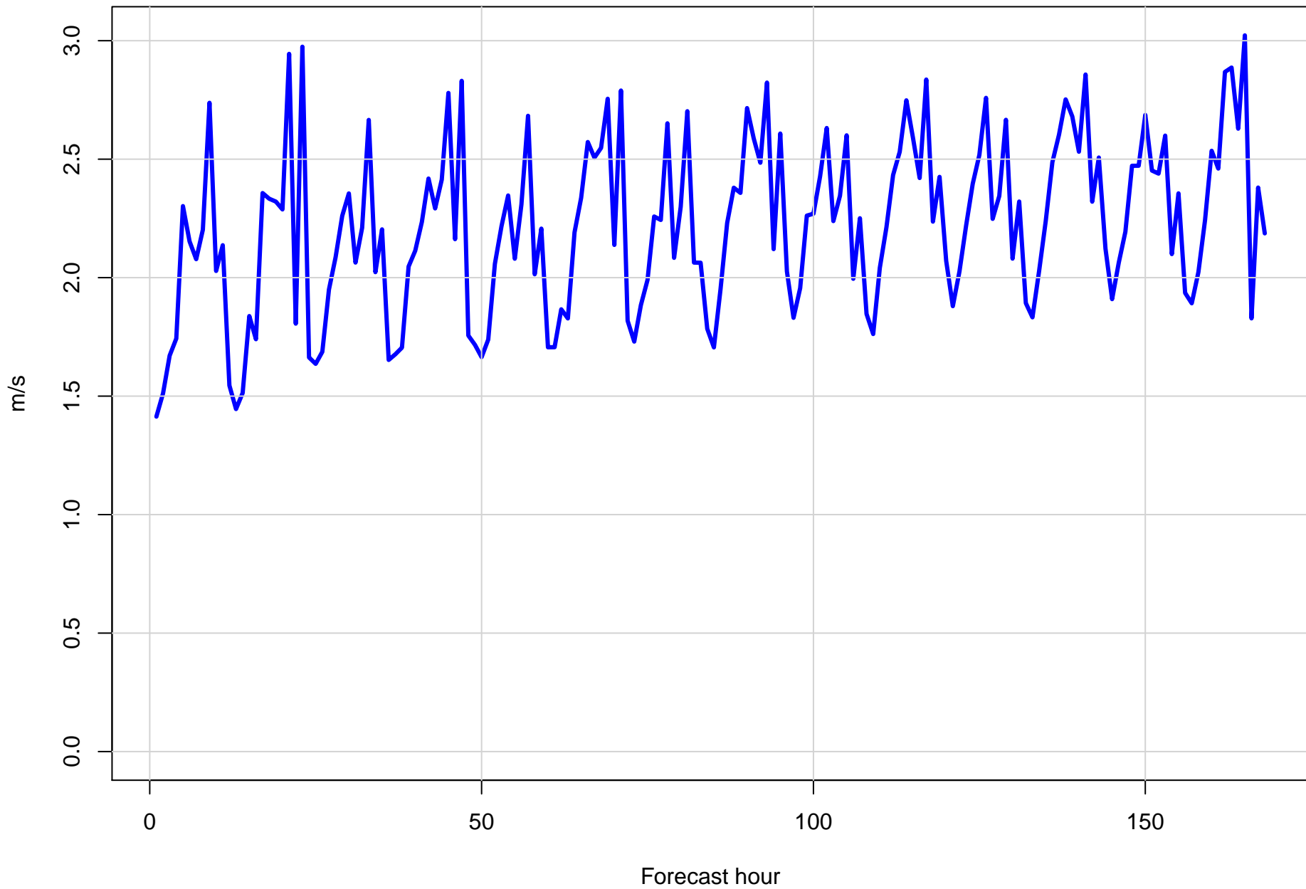
Surface wind speed RMSE at KMCO by forecast hour
