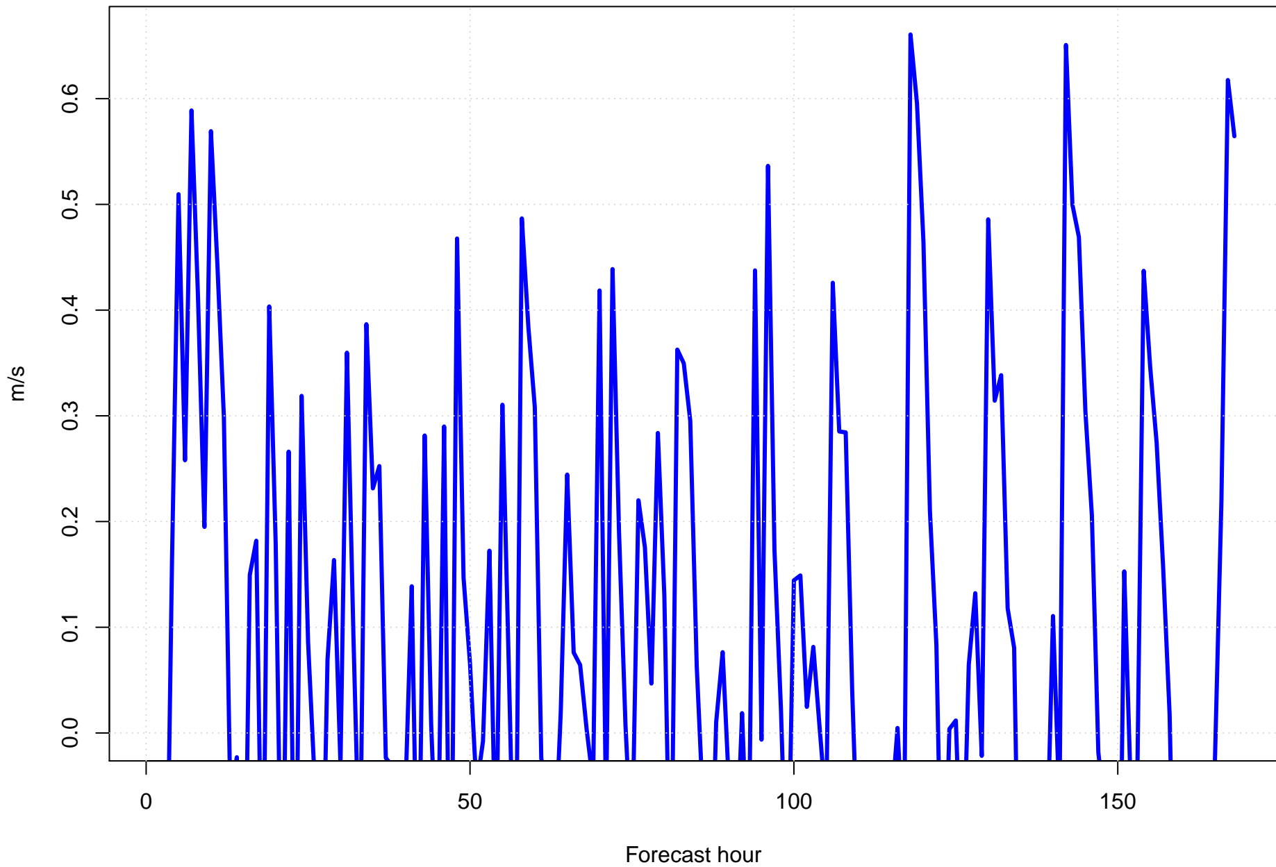
Surface wind speed bias at KMCO by forecast hour
