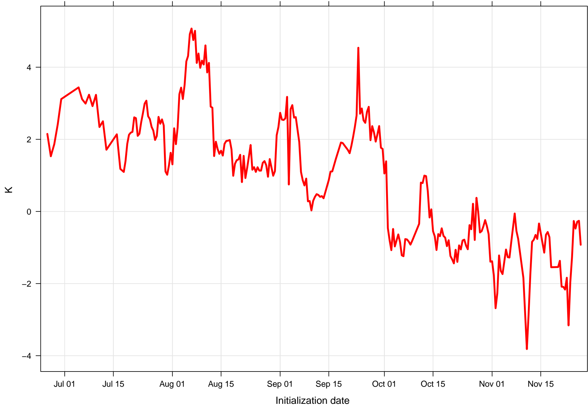
Surface temperature bias at KMCO all forecast hours and members
