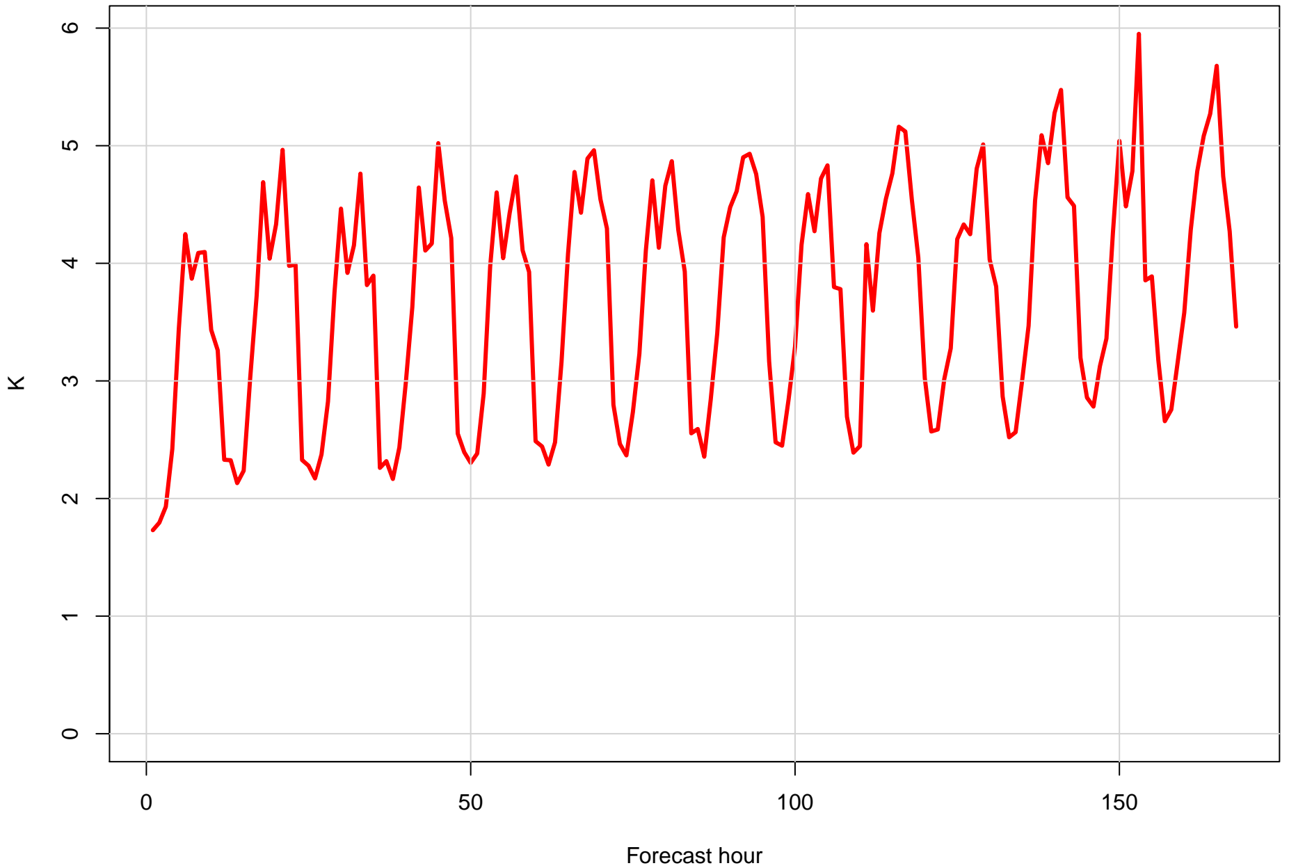
Surface temperature RMSE at KMCO by forecast hour
