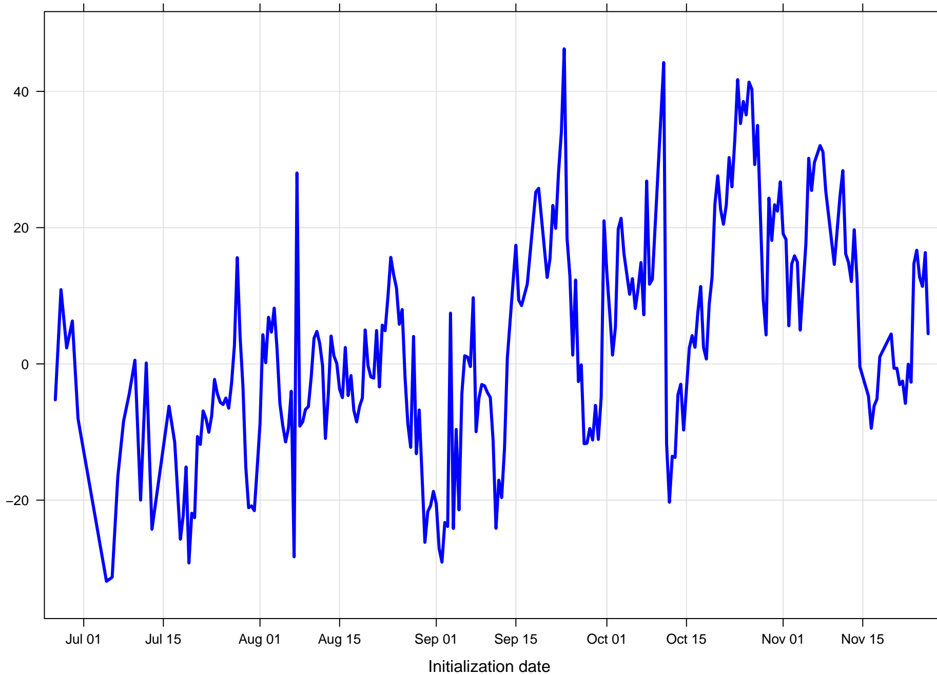
Surface wind direction bias at KMCO all forecast hours and members
