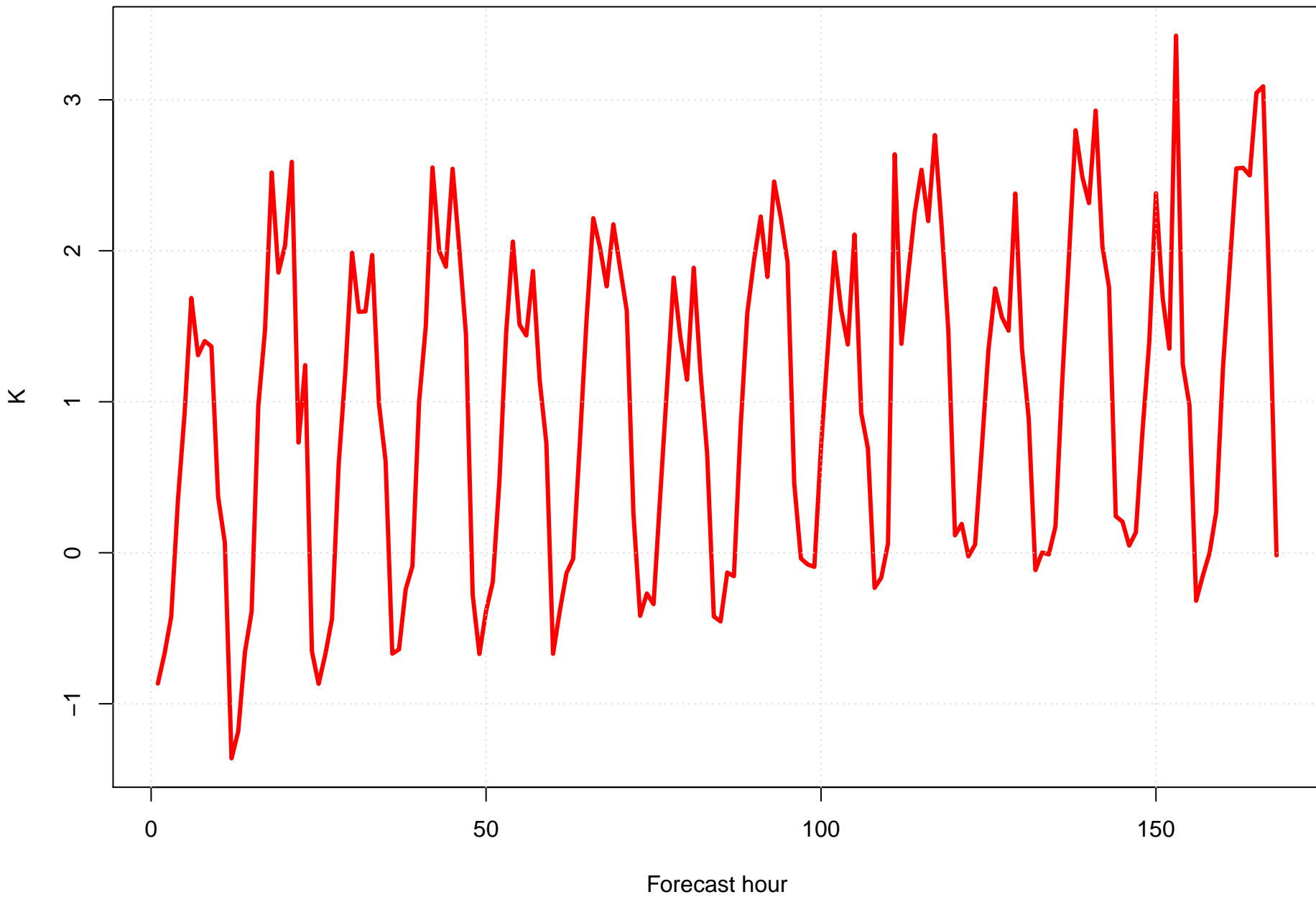
Surface temperature bias at KMCO by forecast hour
