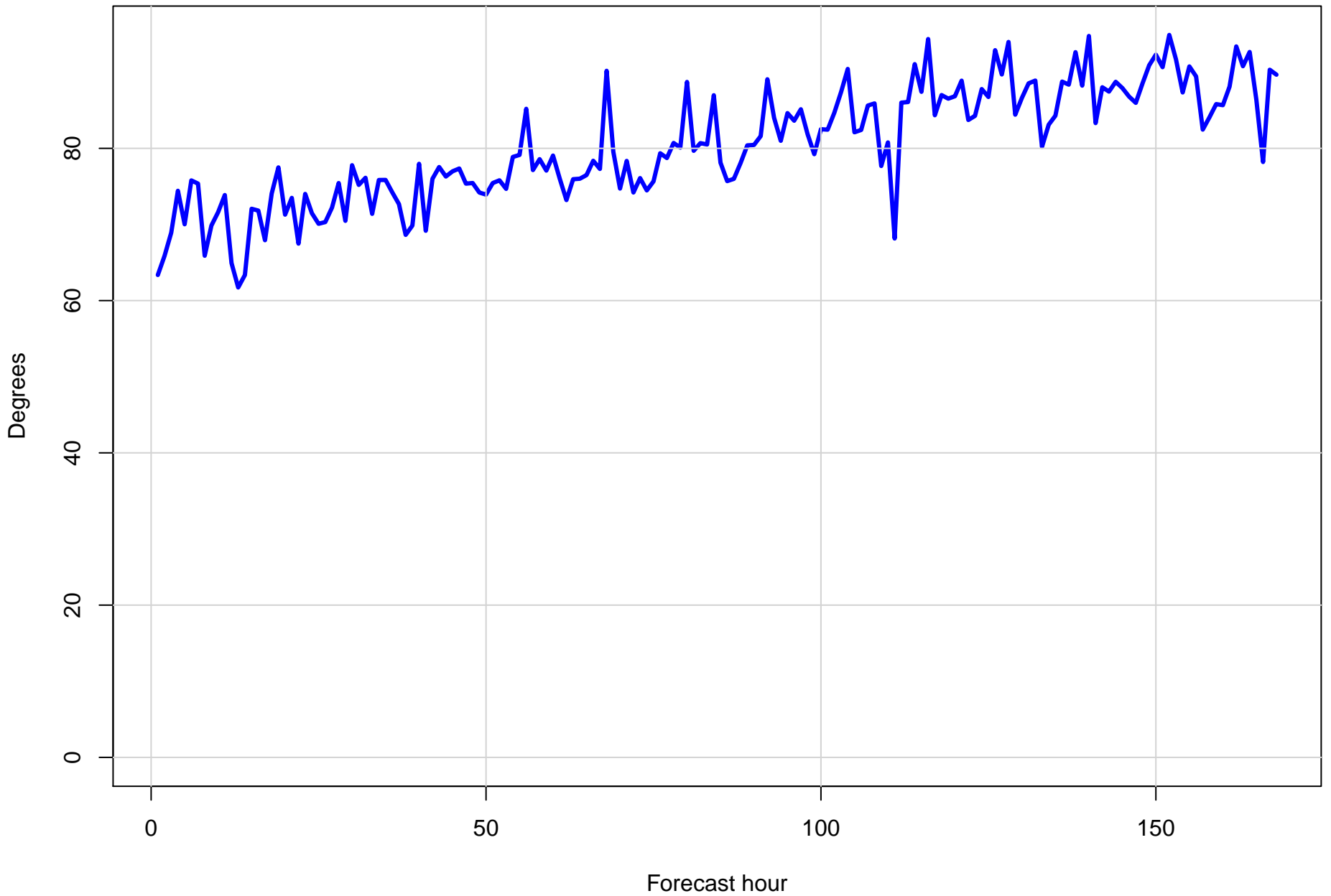
Surface wind direction RMSE at KMCO by forecast hour
