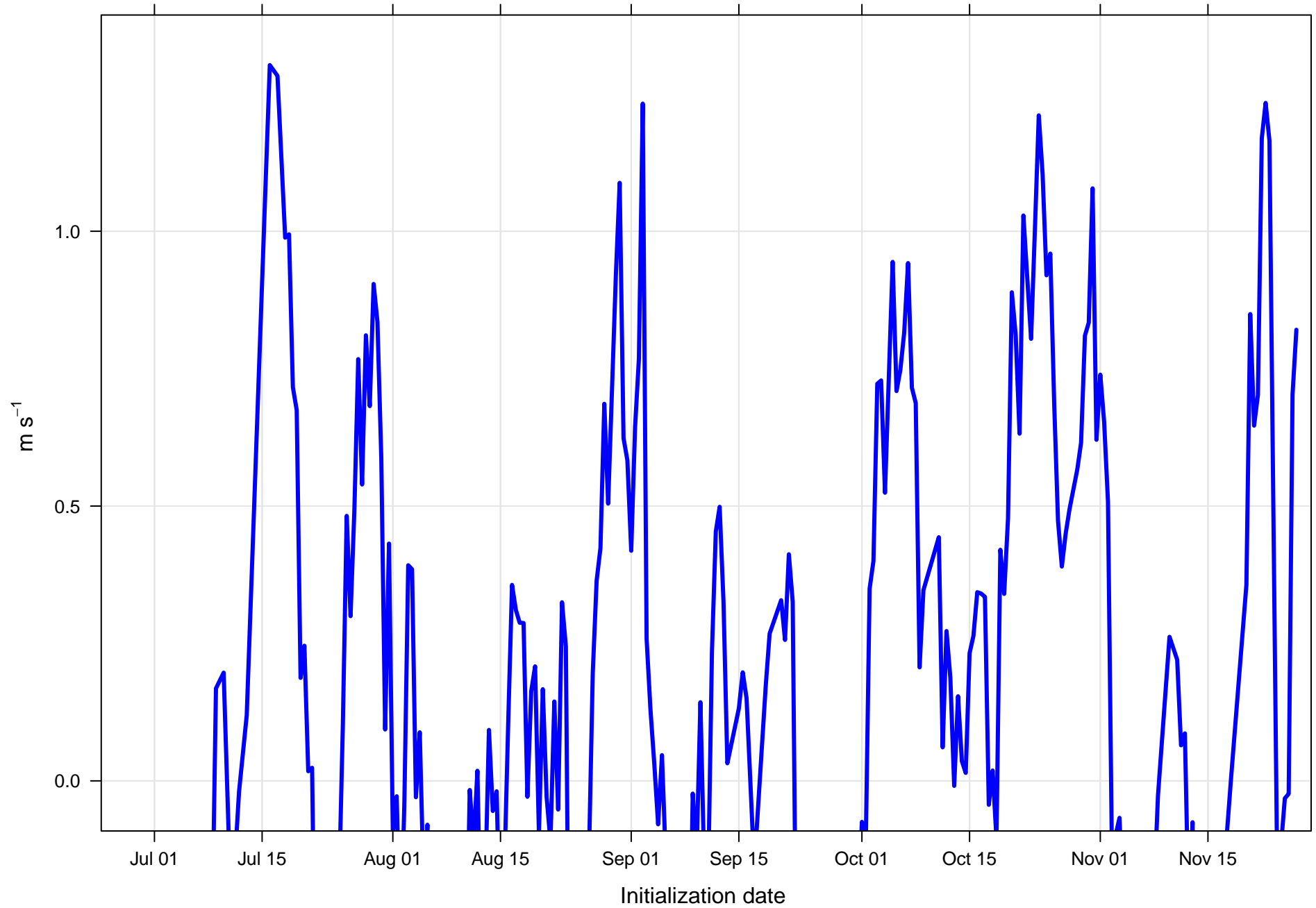
Surface wind speed bias at KMCO all forecast hours and members
