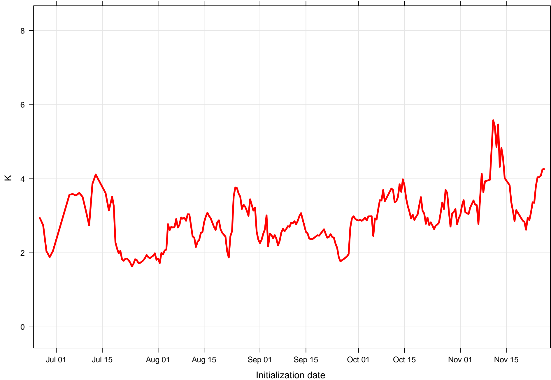
Surface dew point RMSE at KMSY all forecast hours and members
