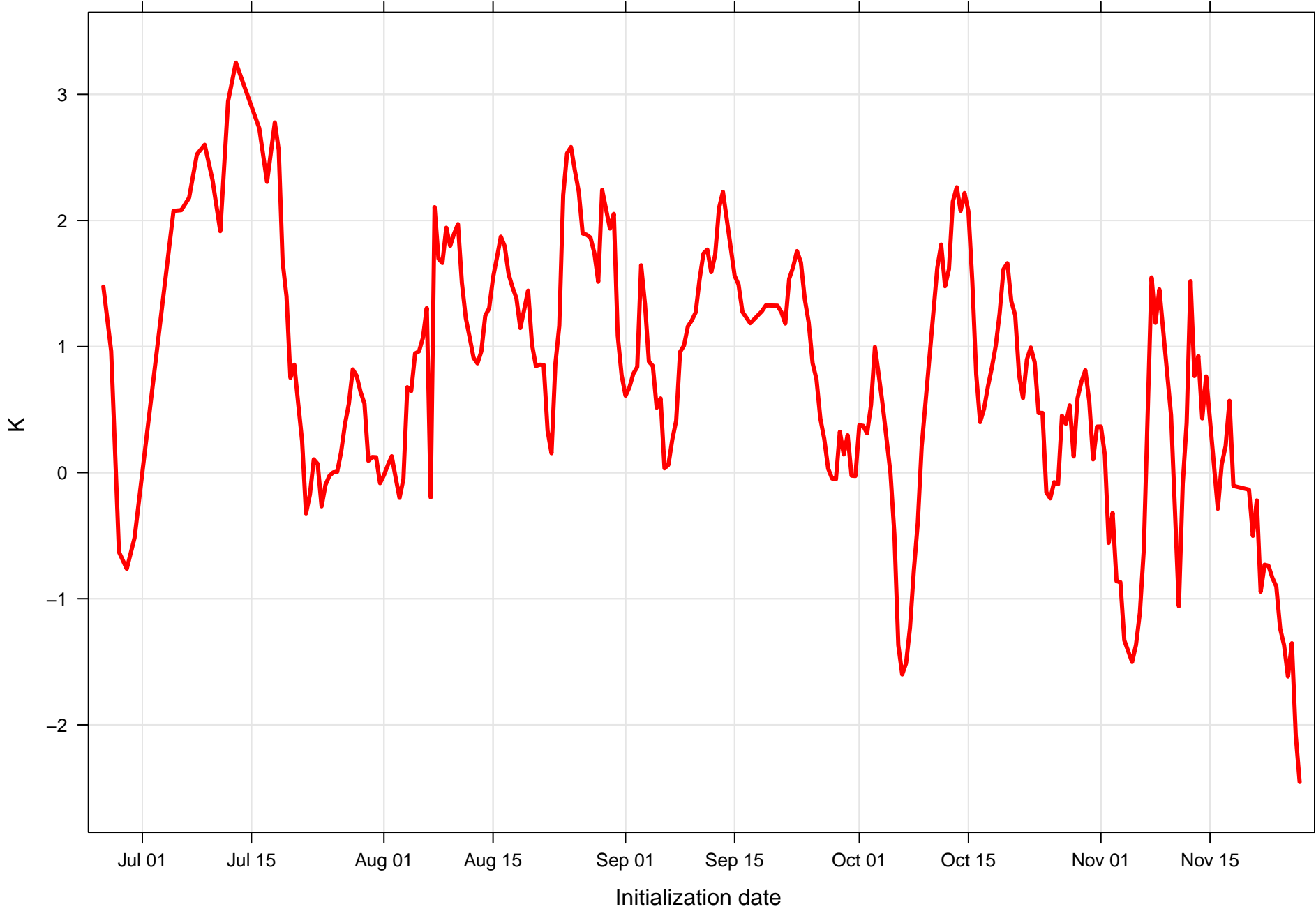
Surface temperature bias at KMSY all forecast hours and members
