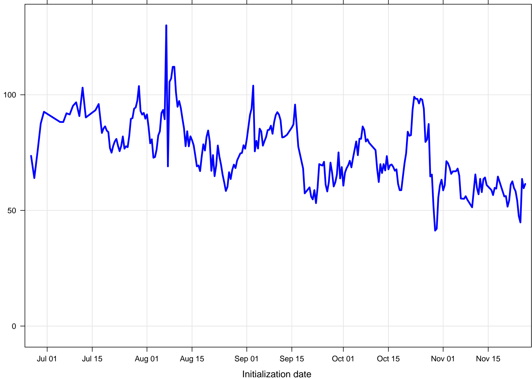
Surface wind direction RMSE at KMSY all forecast hours and members
