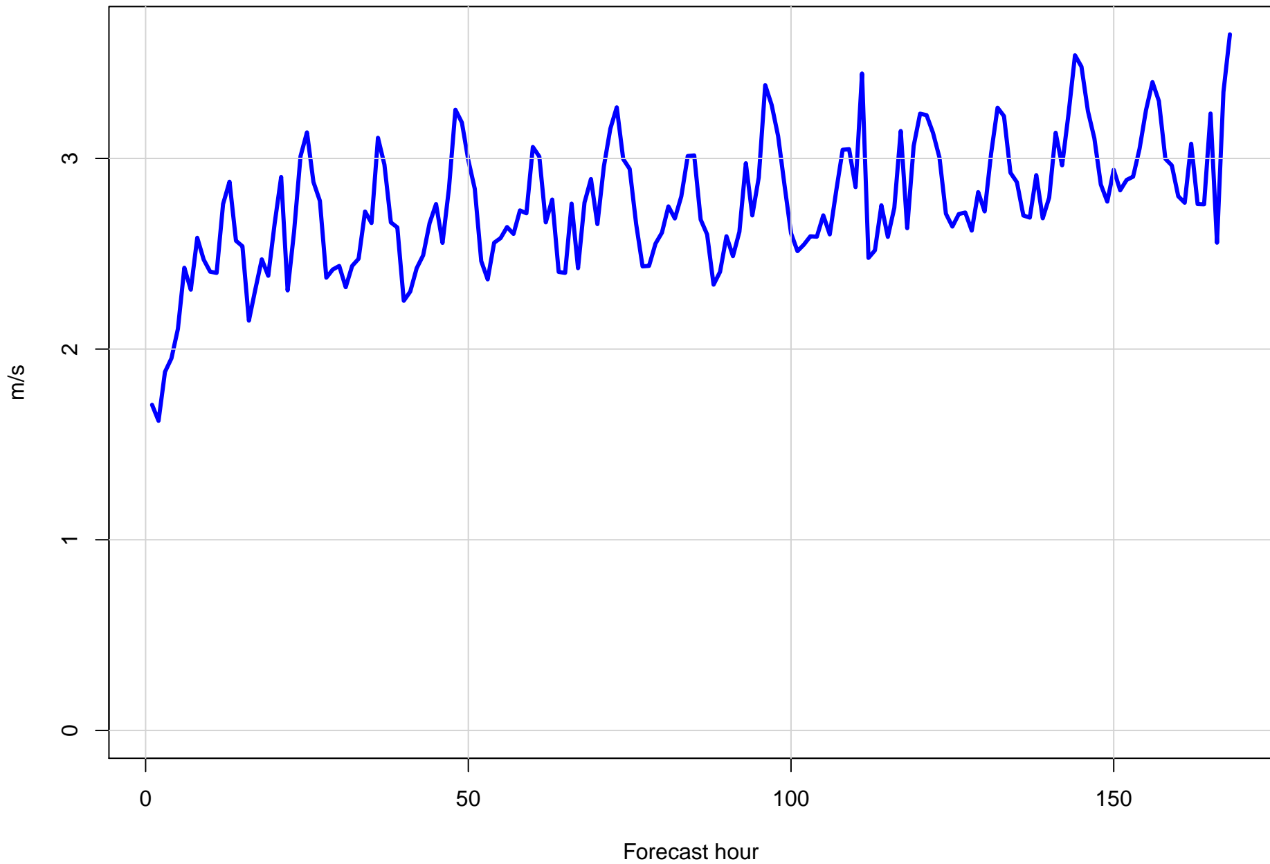
Surface wind speed RMSE at KMSY by forecast hour
