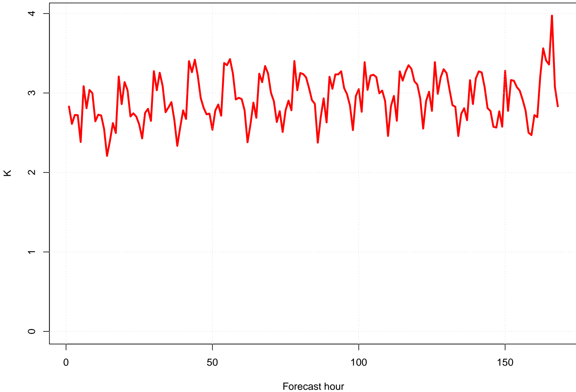
Surface dew point bias at KMSY by forecast hour
