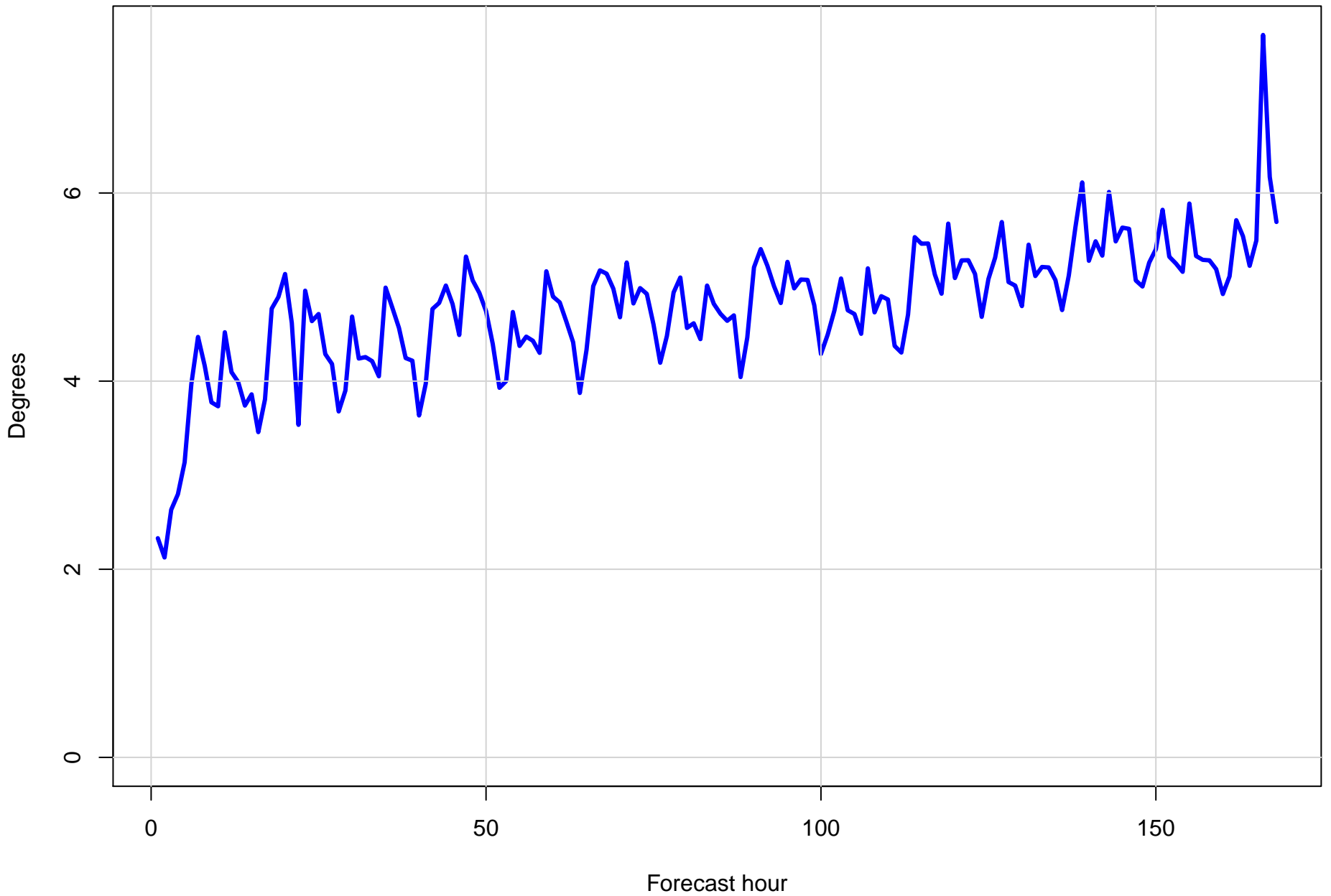
Surface vector wind RMSE at KMSY by forecast hour
