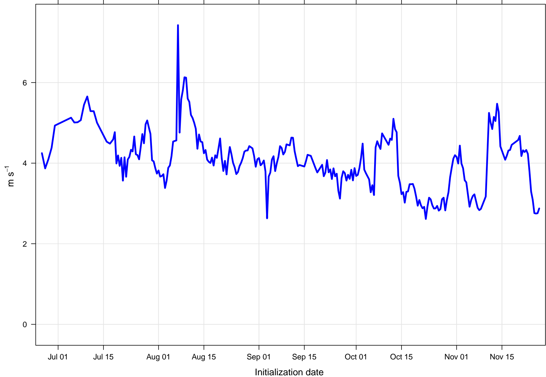
Surface vector wind mean error KMSY all forecast hours and members
