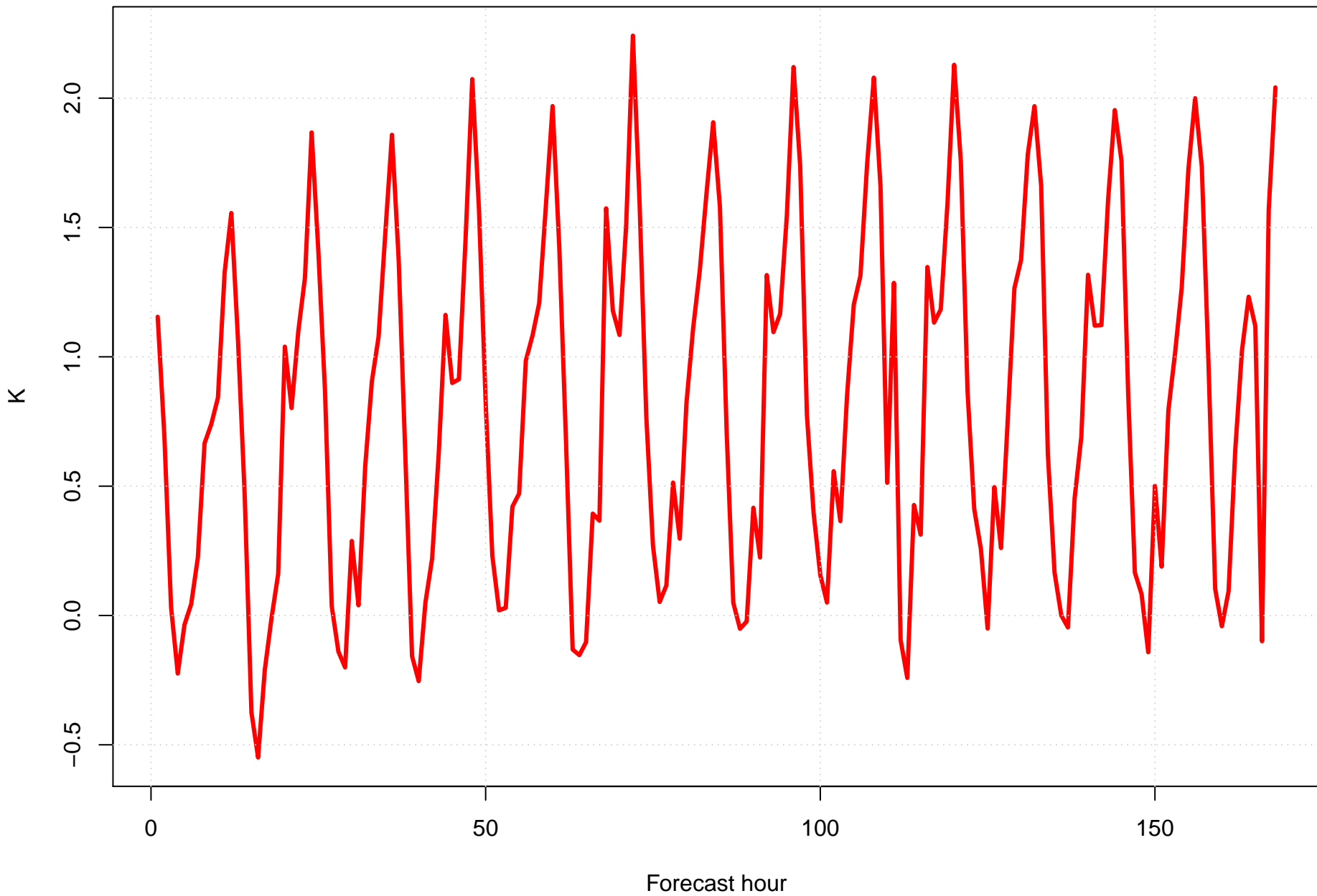
Surface temperature bias at KMSY by forecast hour
