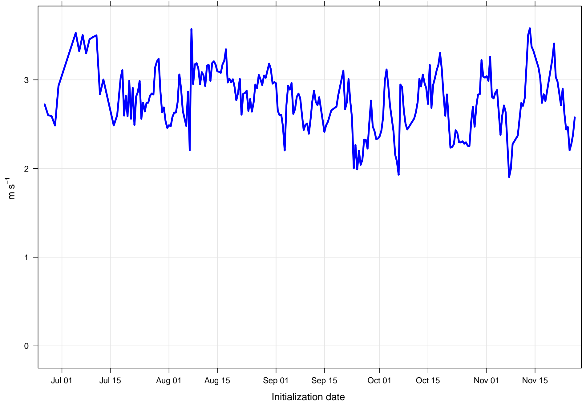
Surface wind speed RMSE at KMSY all forecast hours and members
