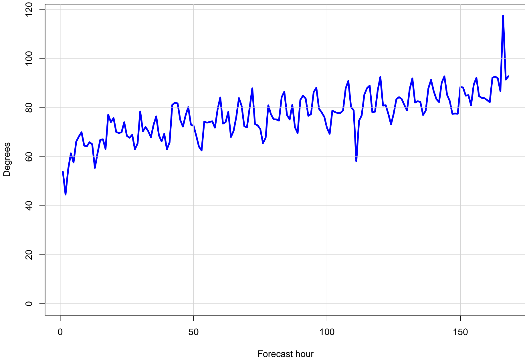
Surface wind direction RMSE at KMSY by forecast hour
