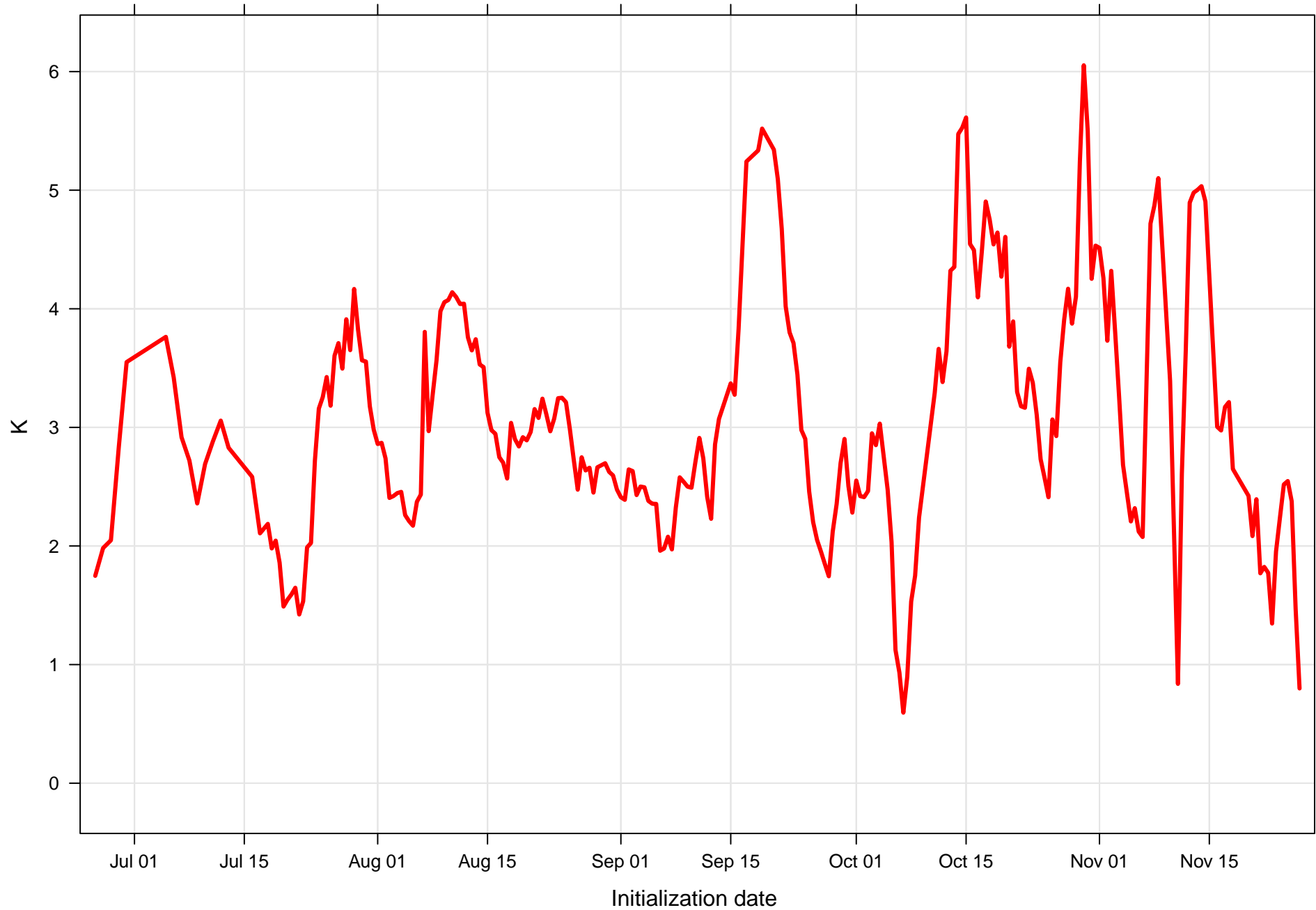
Surface dew point bias at KMSY all forecast hours and members
