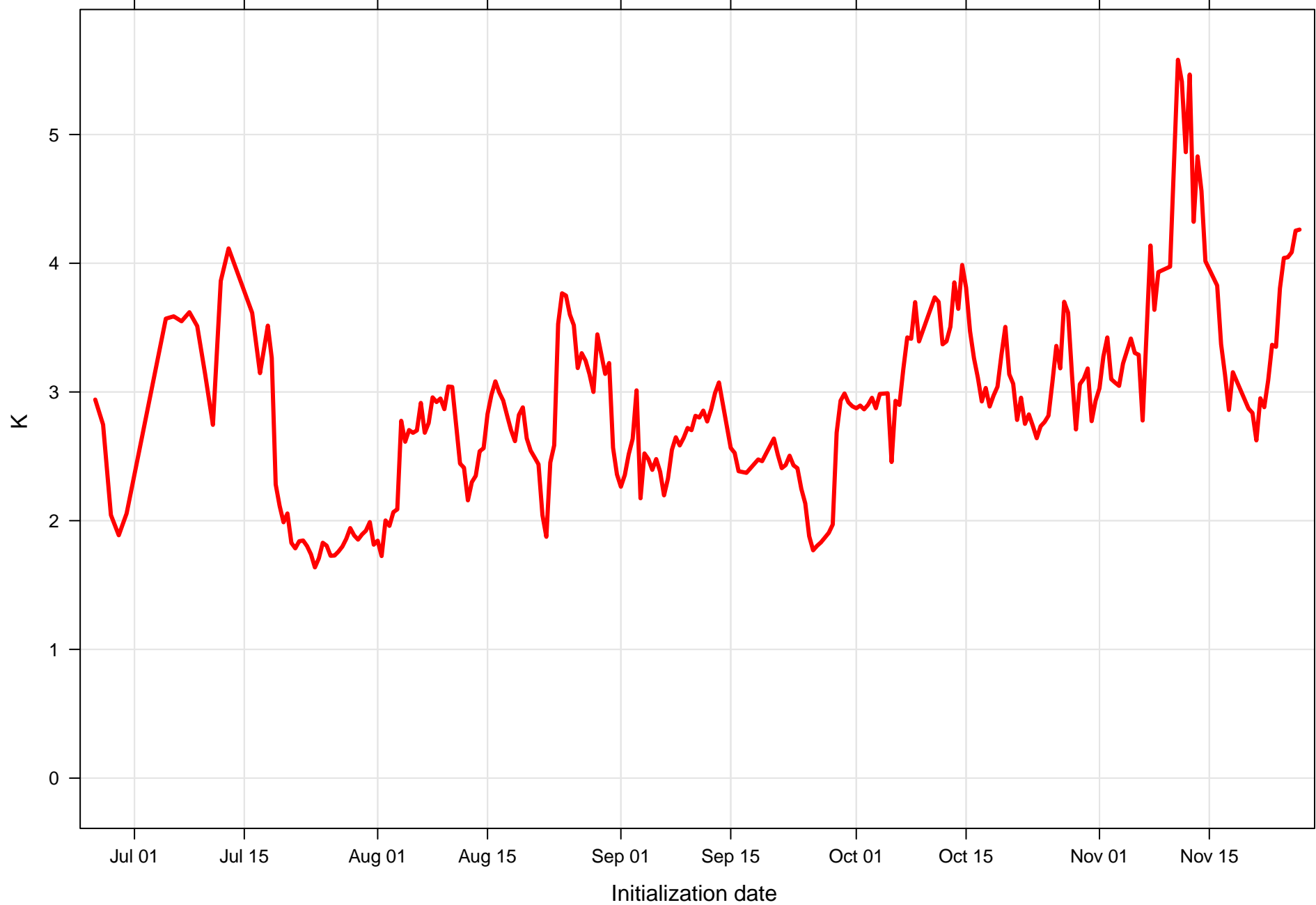
Surface temperature RMSE at KMSY all forecast hours and members
