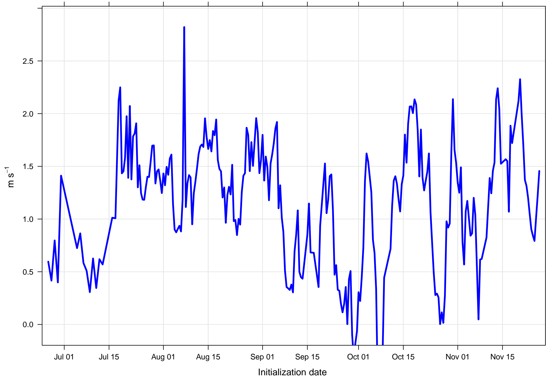
Surface wind speed bias at KMSY all forecast hours and members
