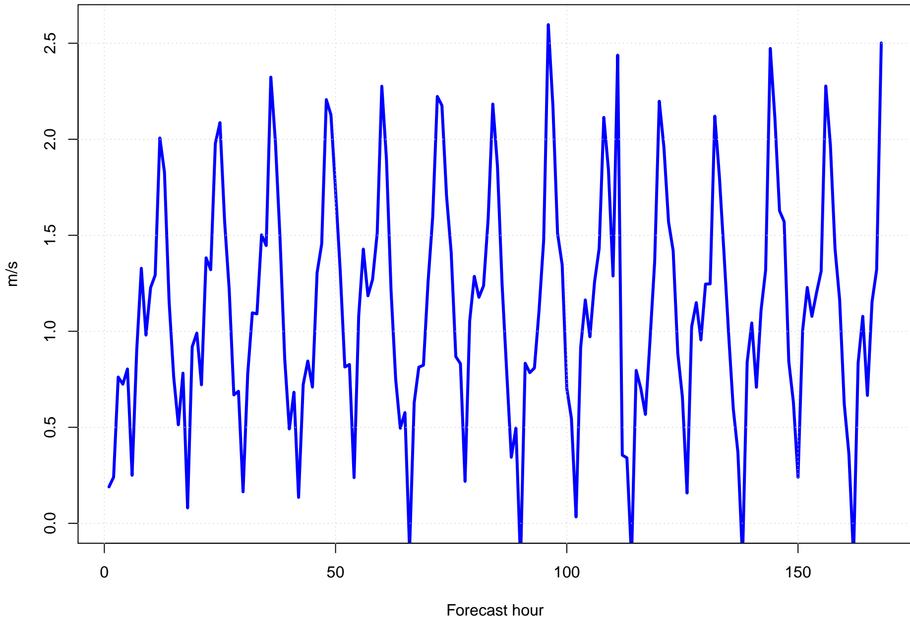
Surface wind speed bias at KMSY by forecast hour
