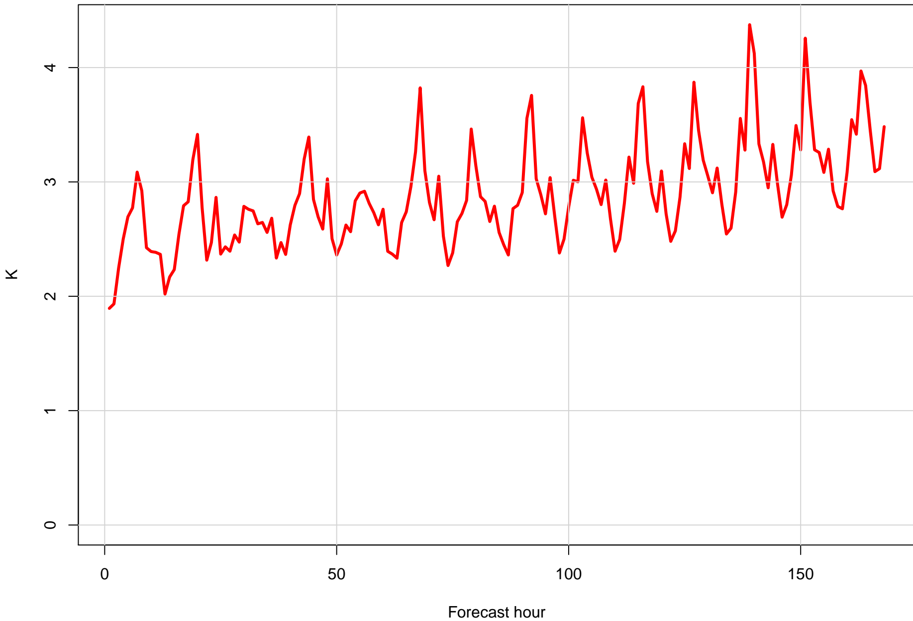
Surface temperature RMSE at KMSY by forecast hour
