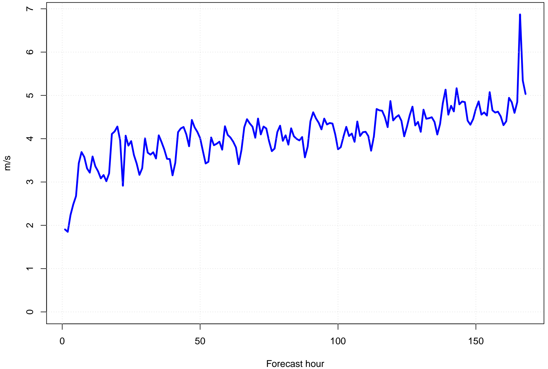
Surface vector wind error at KMSY by forecast hour
