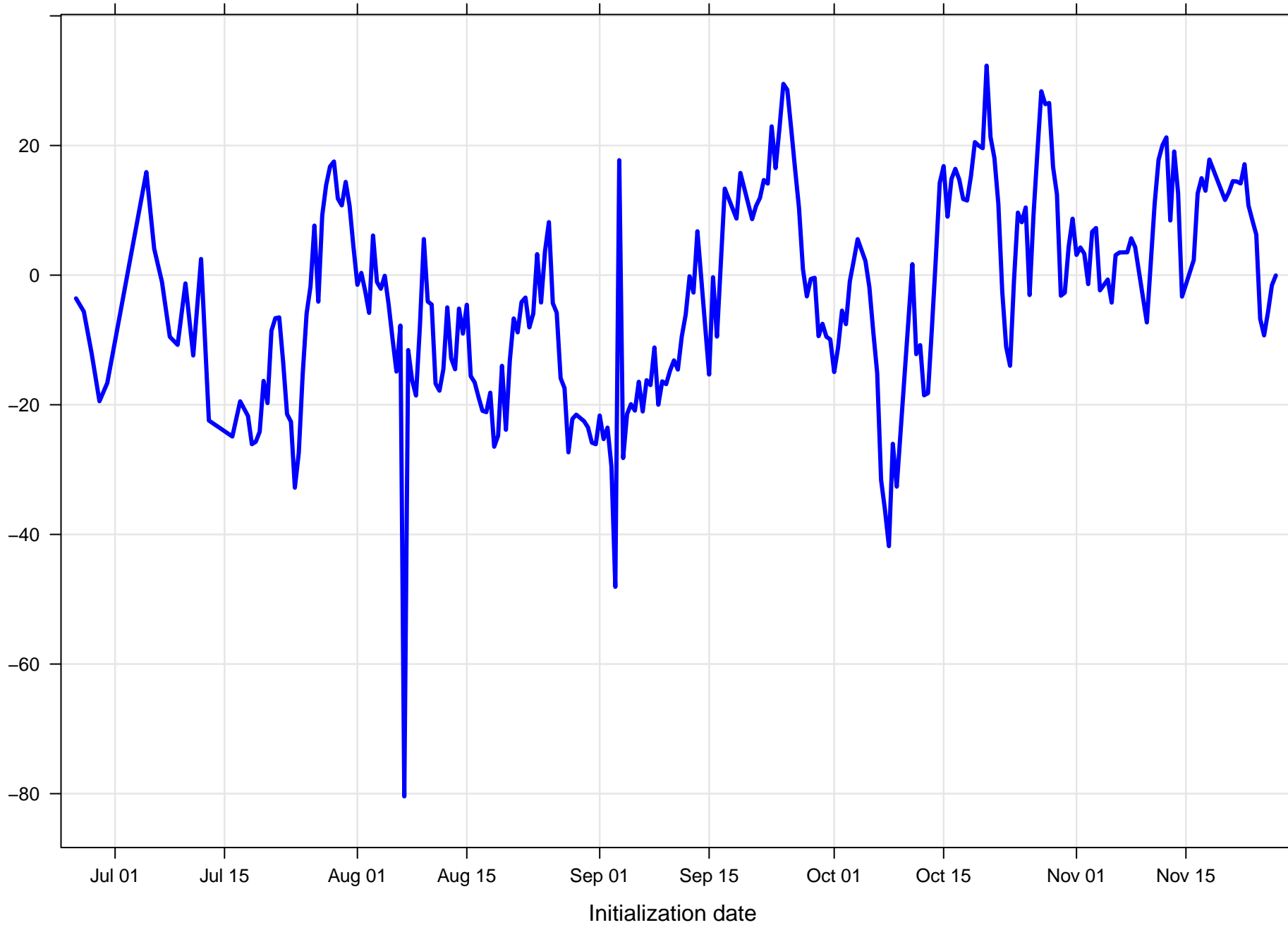
Surface wind direction bias at KMSY all forecast hours and members
