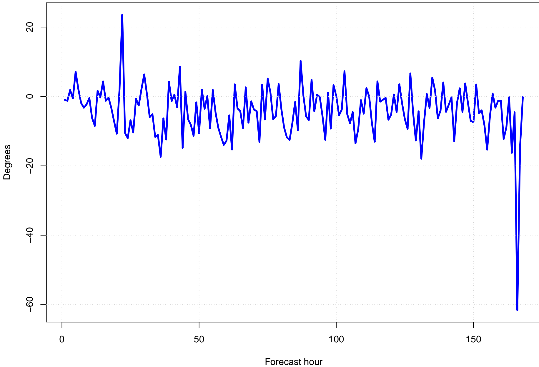
Surface wind direction bias at KMSY by forecast hour
