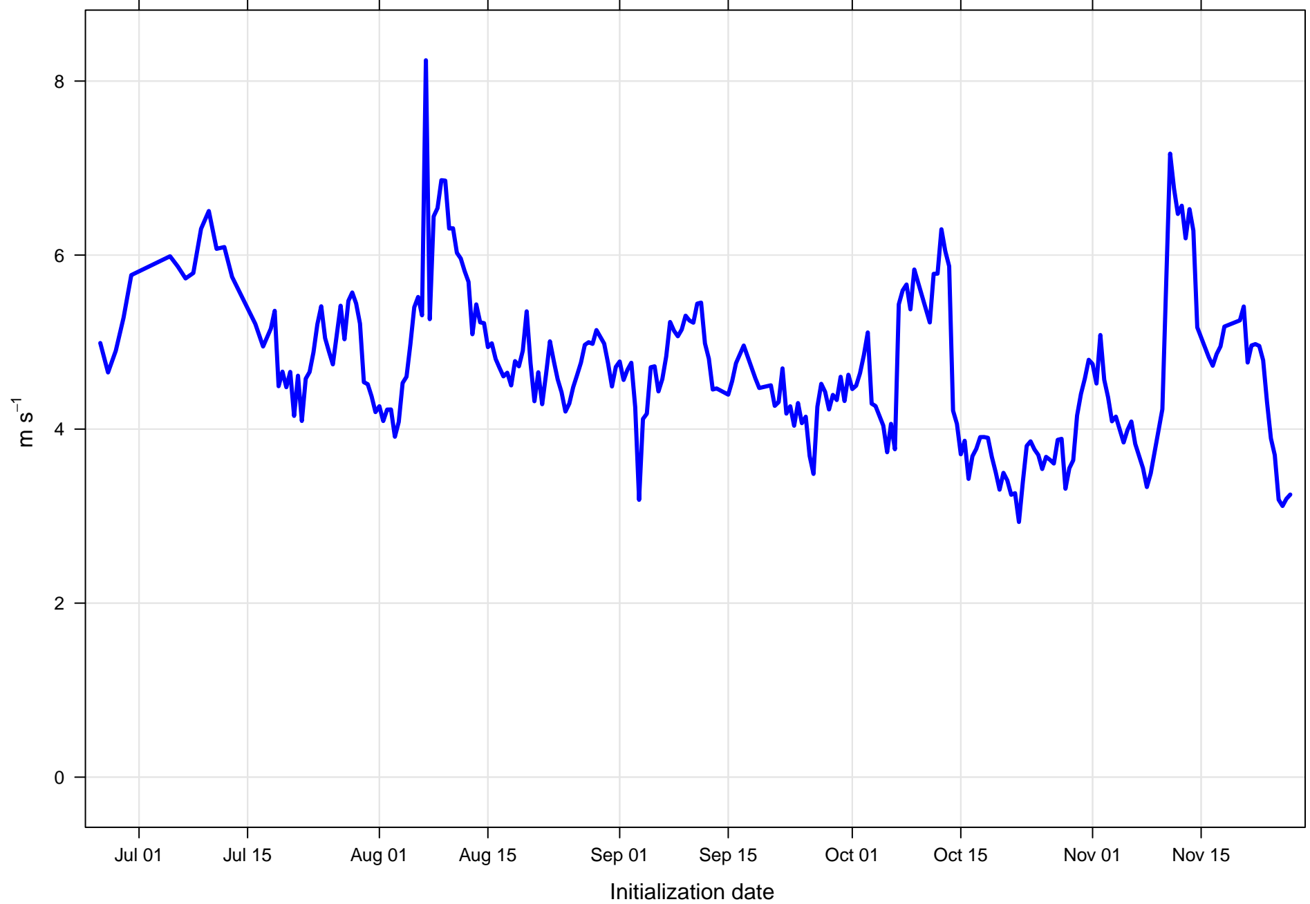
Surface vector wind RMSE at KMSY all forecast hours and members
