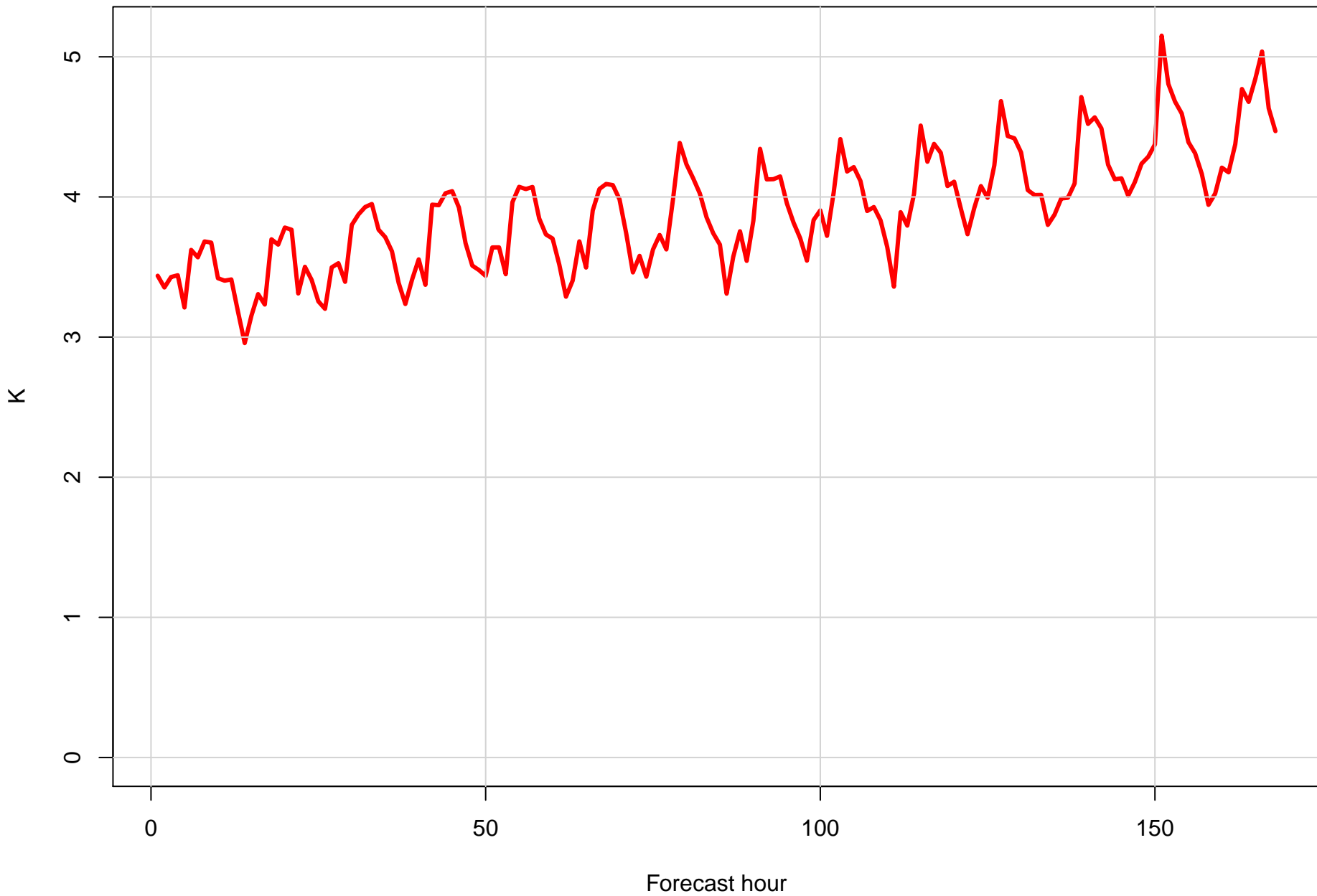
Surface dew point RMSE at KMSY by forecast hour
