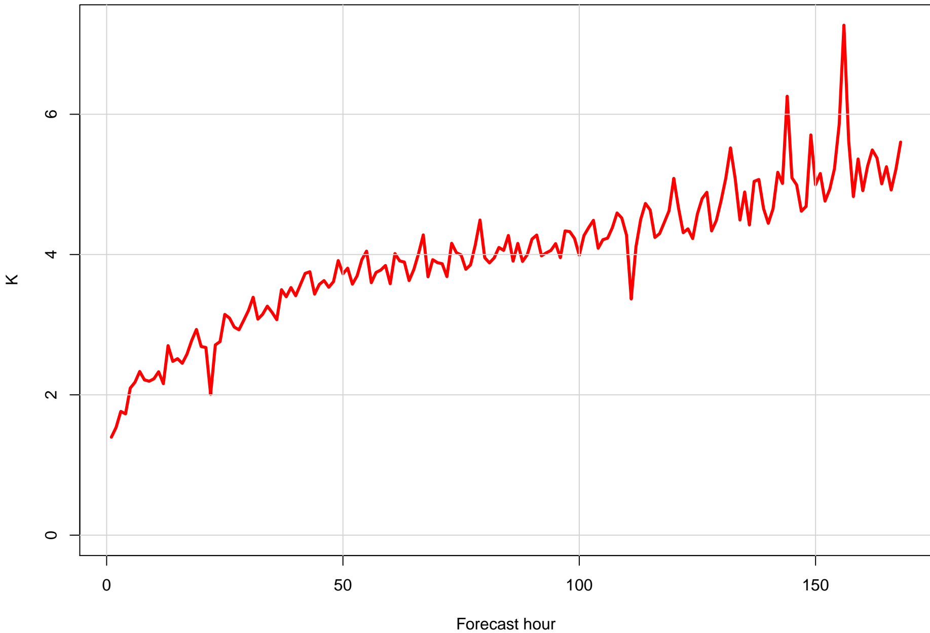
Surface dew point RMSE at KPNS by forecast hour
