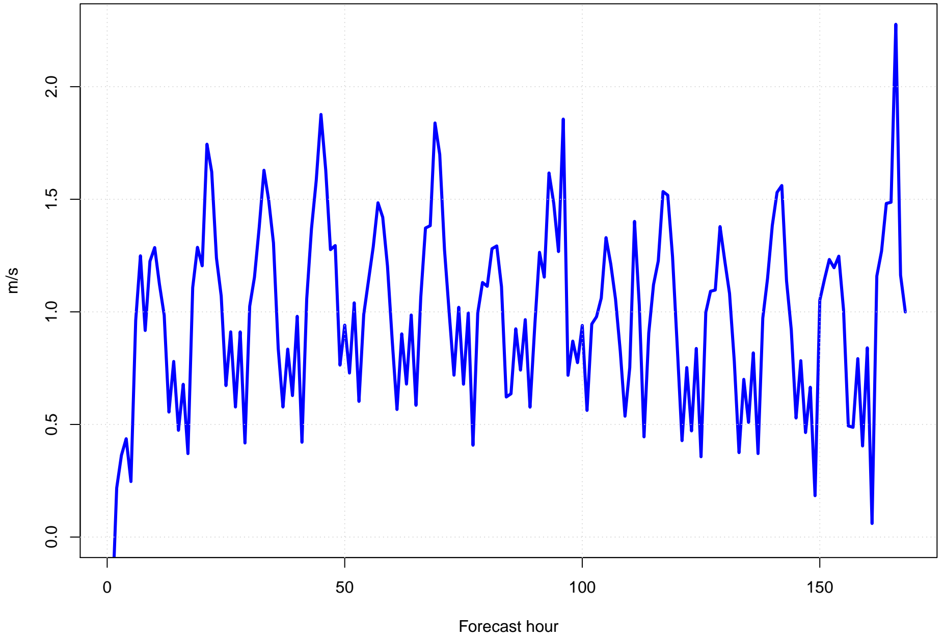
Surface wind speed bias at KPNS by forecast hour
