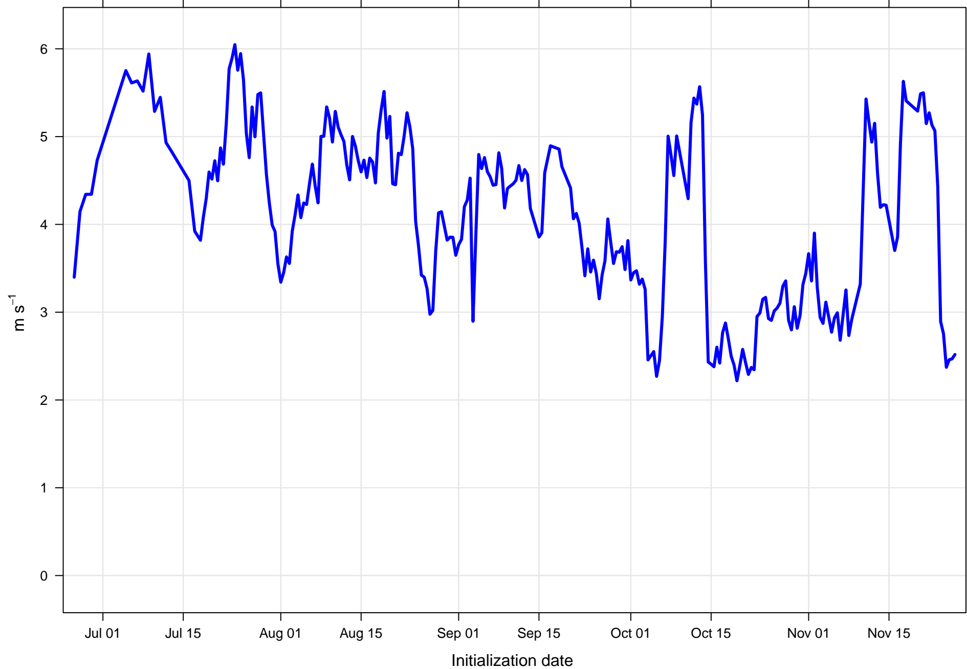
Surface vector wind RMSE at KPNS all forecast hours and members
