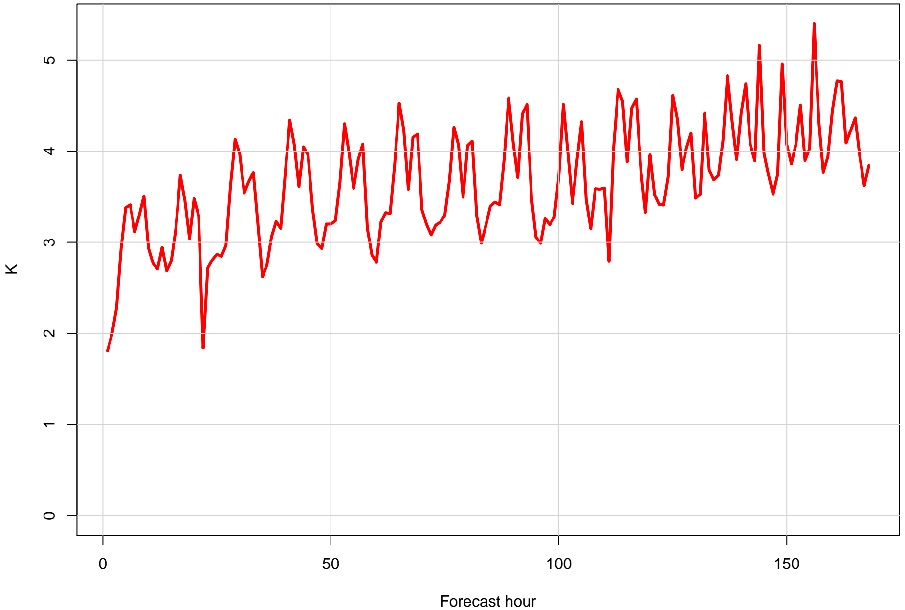
Surface temperature RMSE at KPNS by forecast hour
