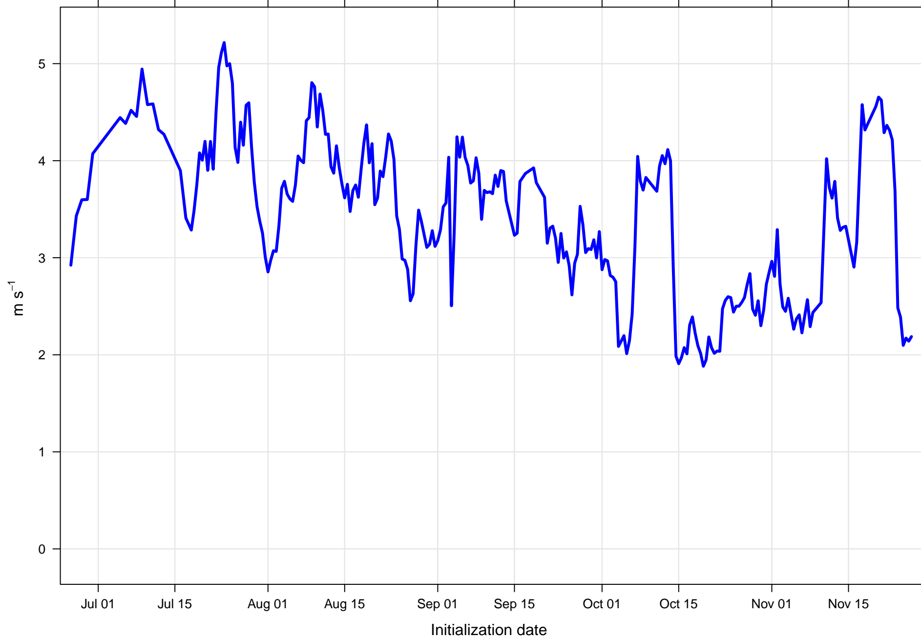
Surface vector wind mean error KPNS all forecast hours and members
