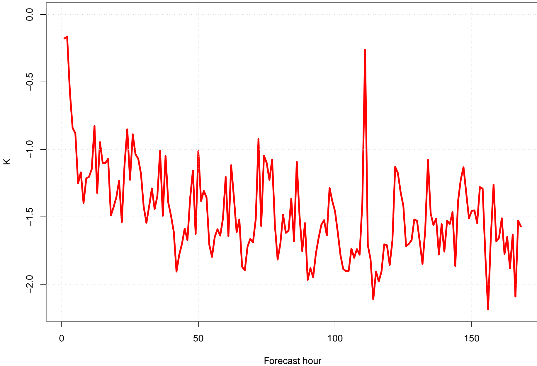
Surface dew point bias at KPNS by forecast hour
