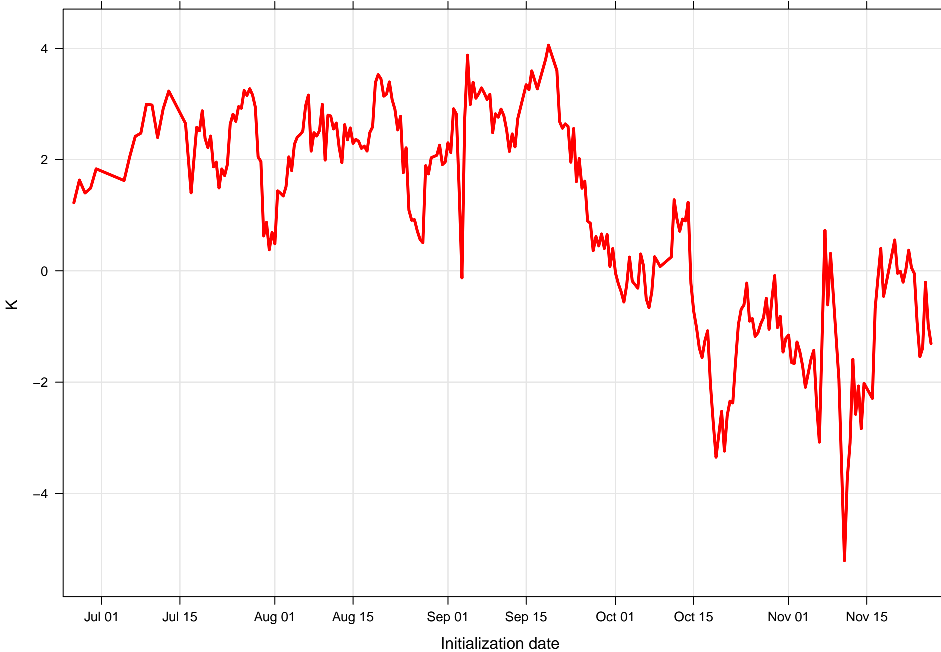
Surface temperature bias at KPNS all forecast hours and members
