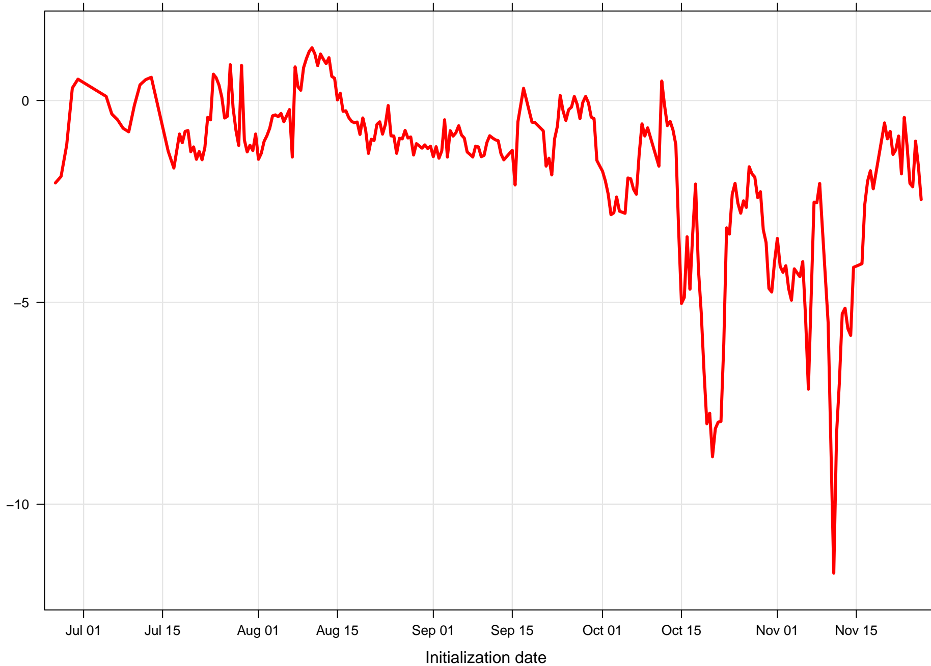
Surface dew point bias at KPNS all forecast hours and members
