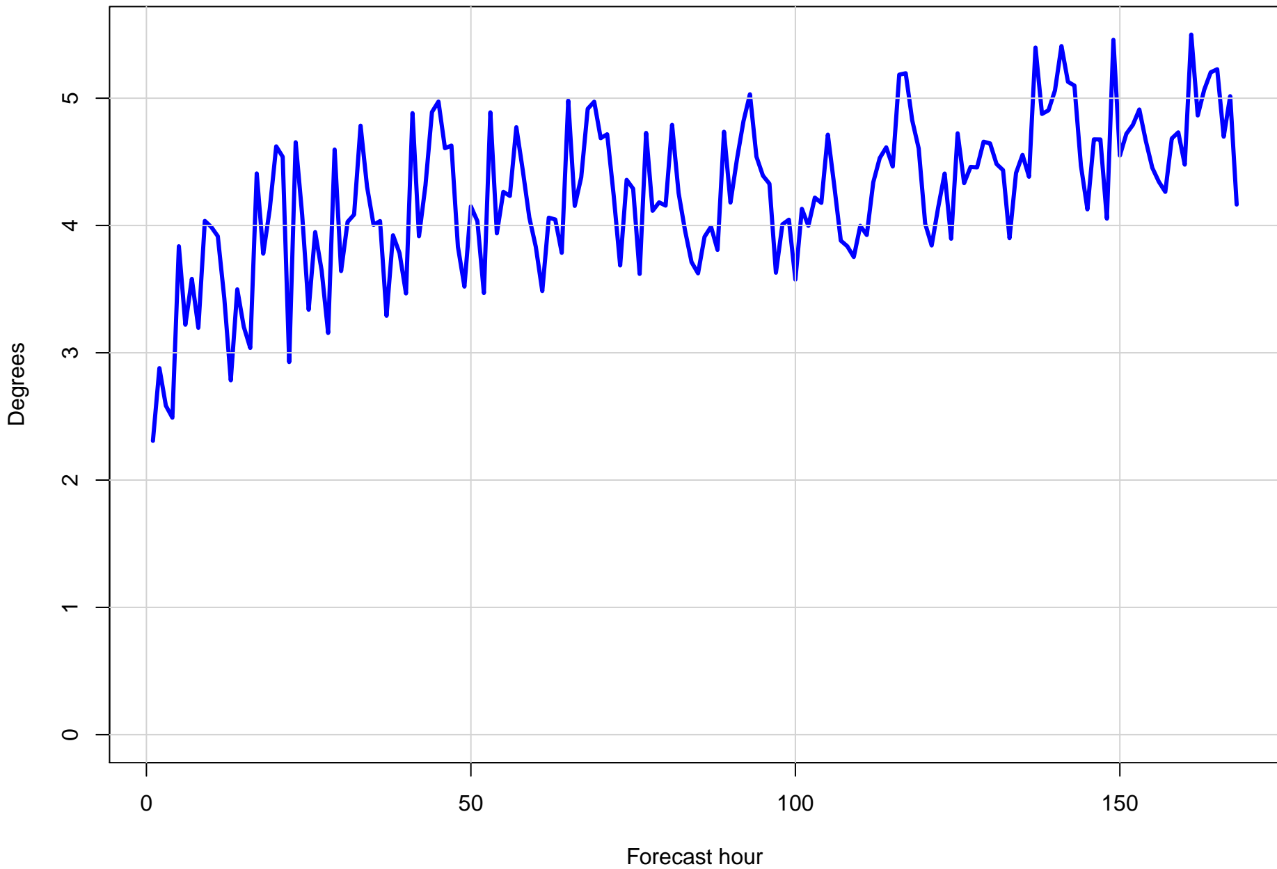
Surface vector wind RMSE at KPNS by forecast hour
