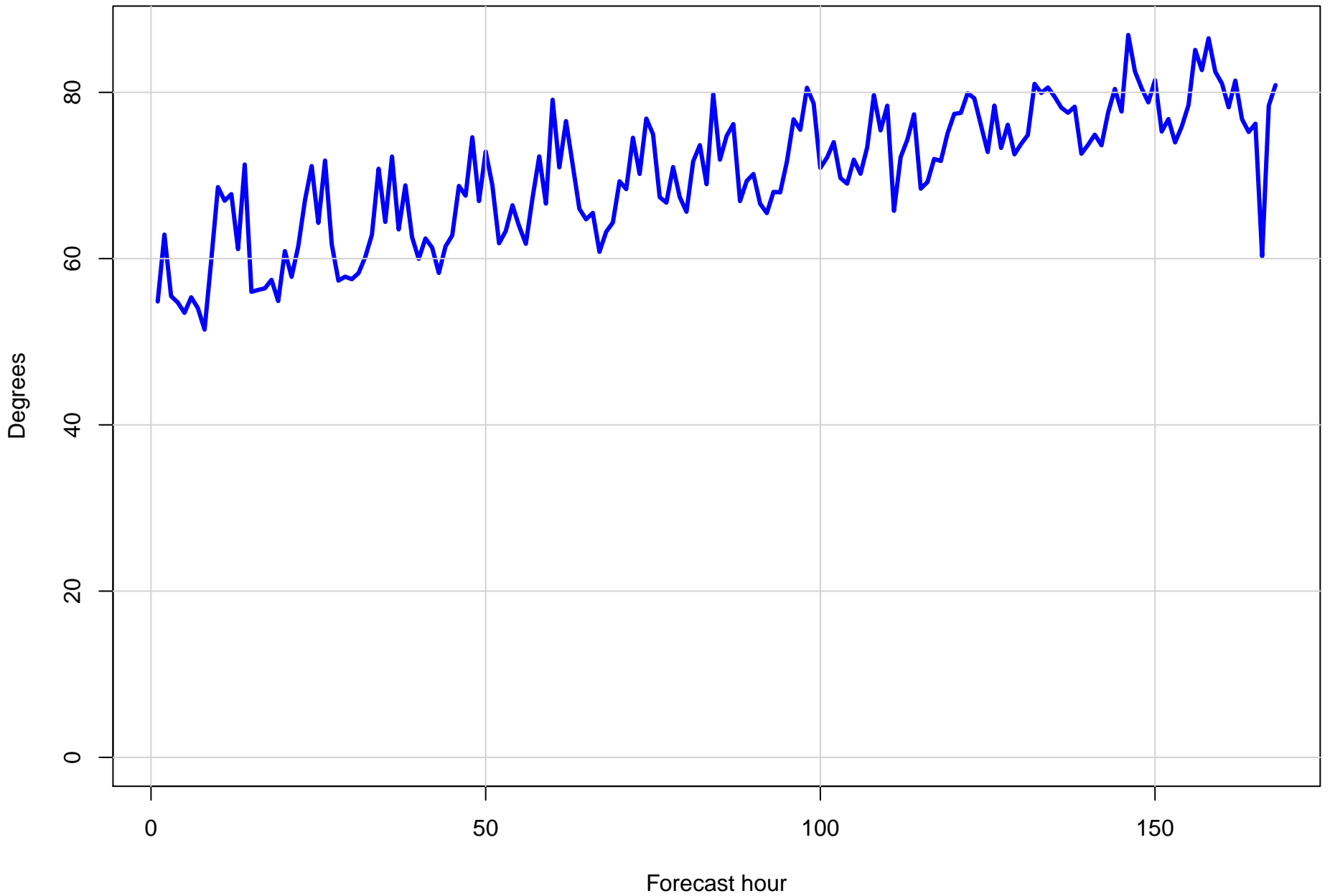
Surface wind direction RMSE at KPNS by forecast hour
