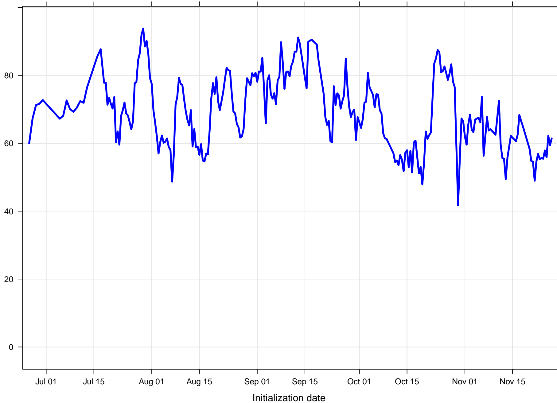
Surface wind direction RMSE at KPNS all forecast hours and members
