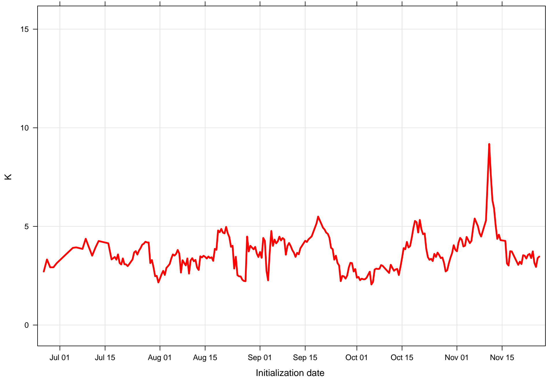
Surface dew point RMSE at KPNS all forecast hours and members
