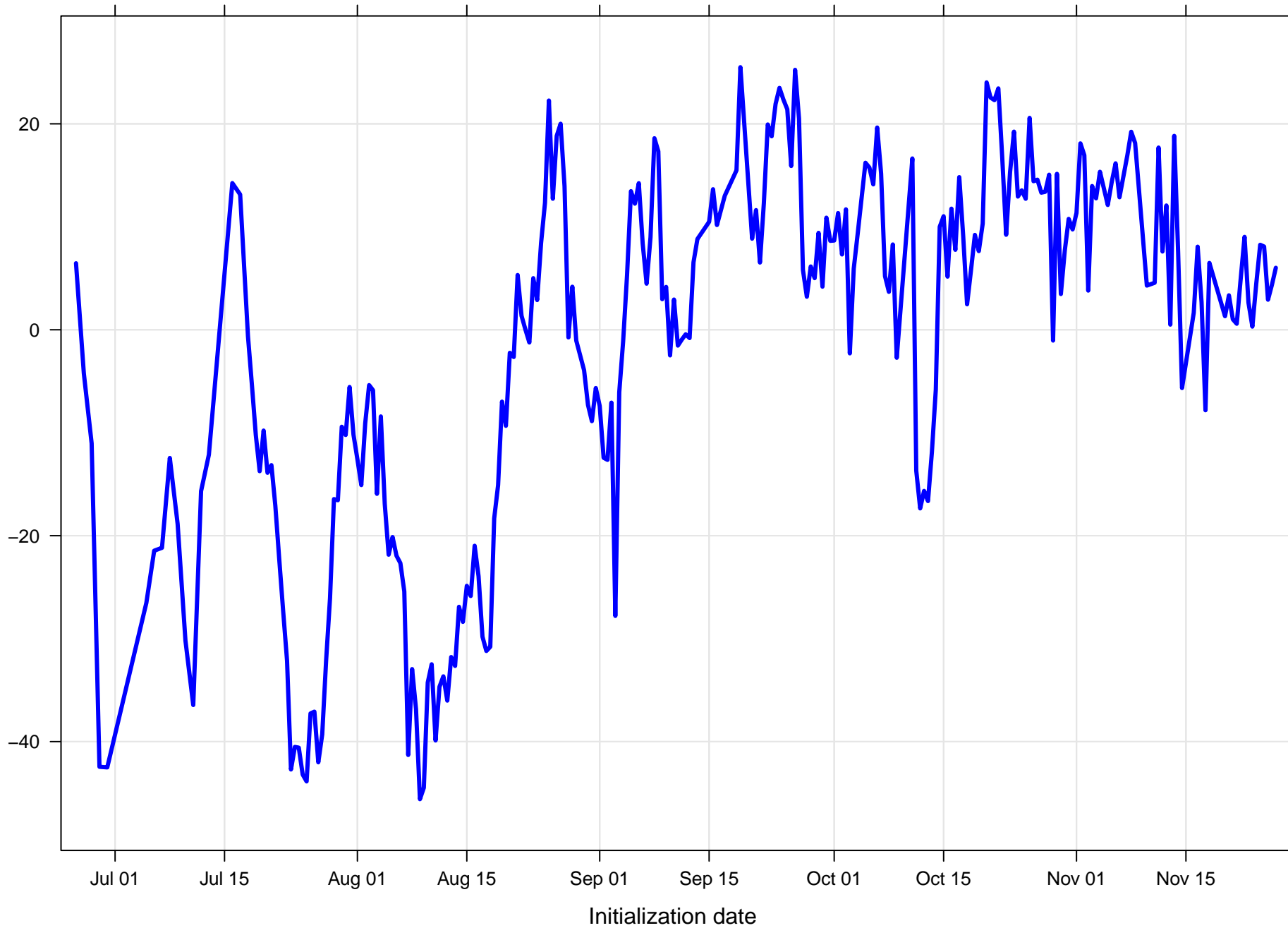
Surface wind direction bias at KPNS all forecast hours and members
