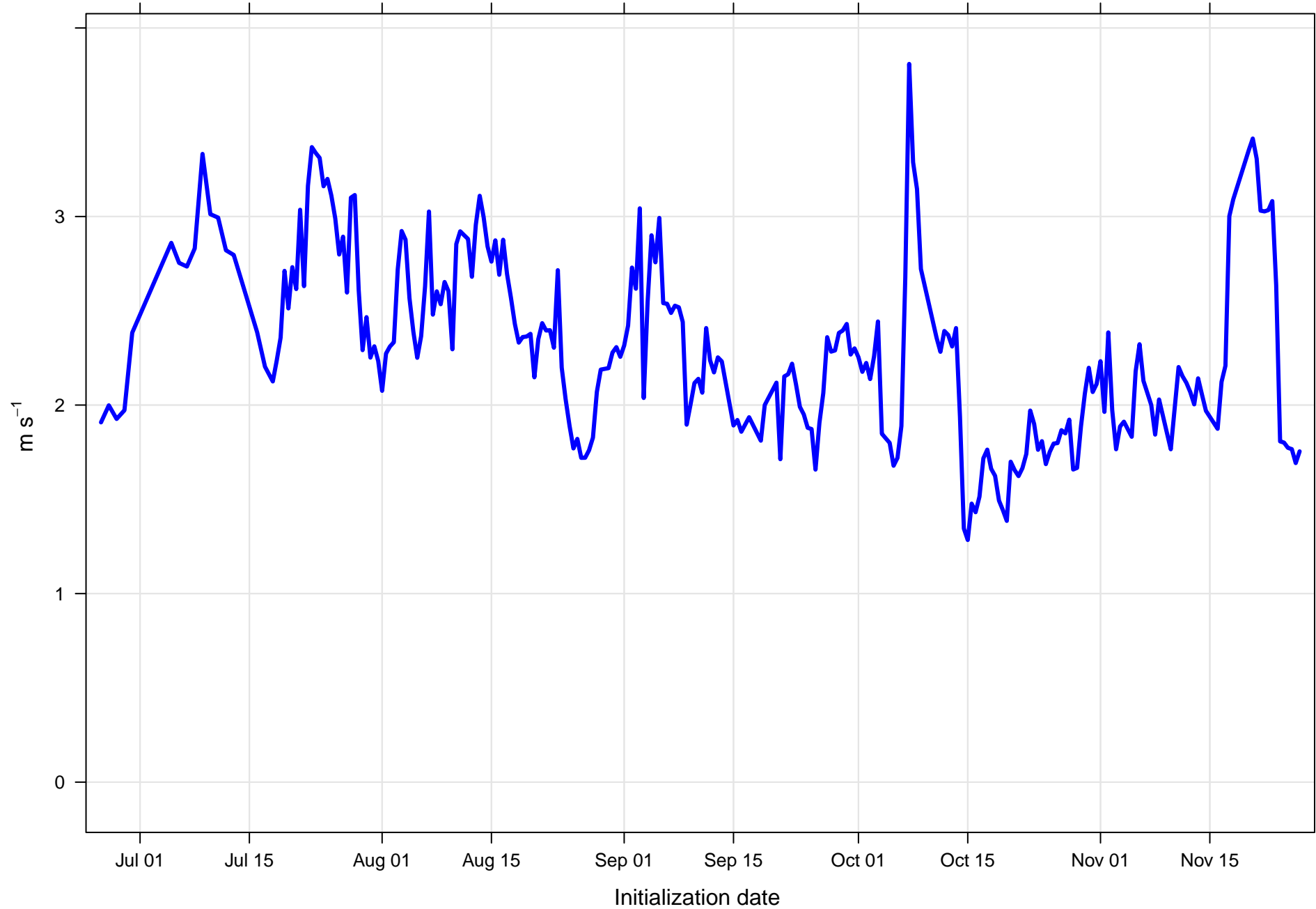
Surface wind speed RMSE at KPNS all forecast hours and members
