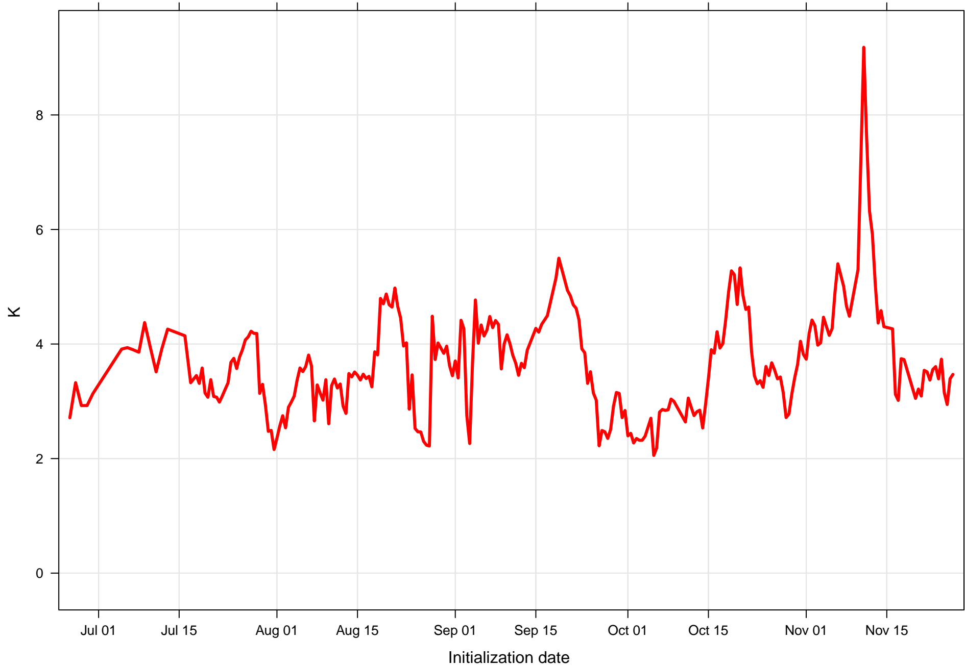
Surface temperature RMSE at KPNS all forecast hours and members
