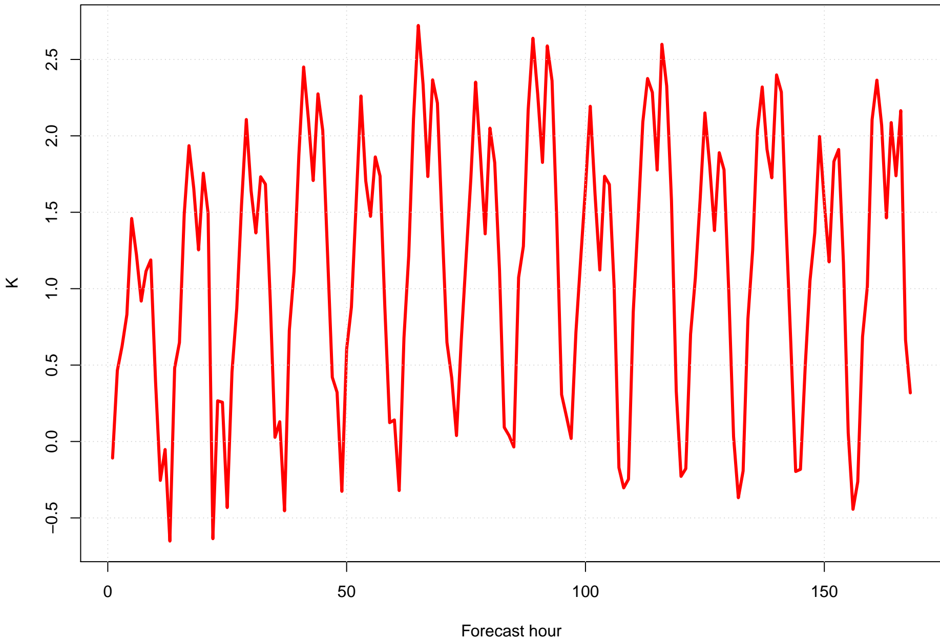
Surface temperature bias at KPNS by forecast hour
