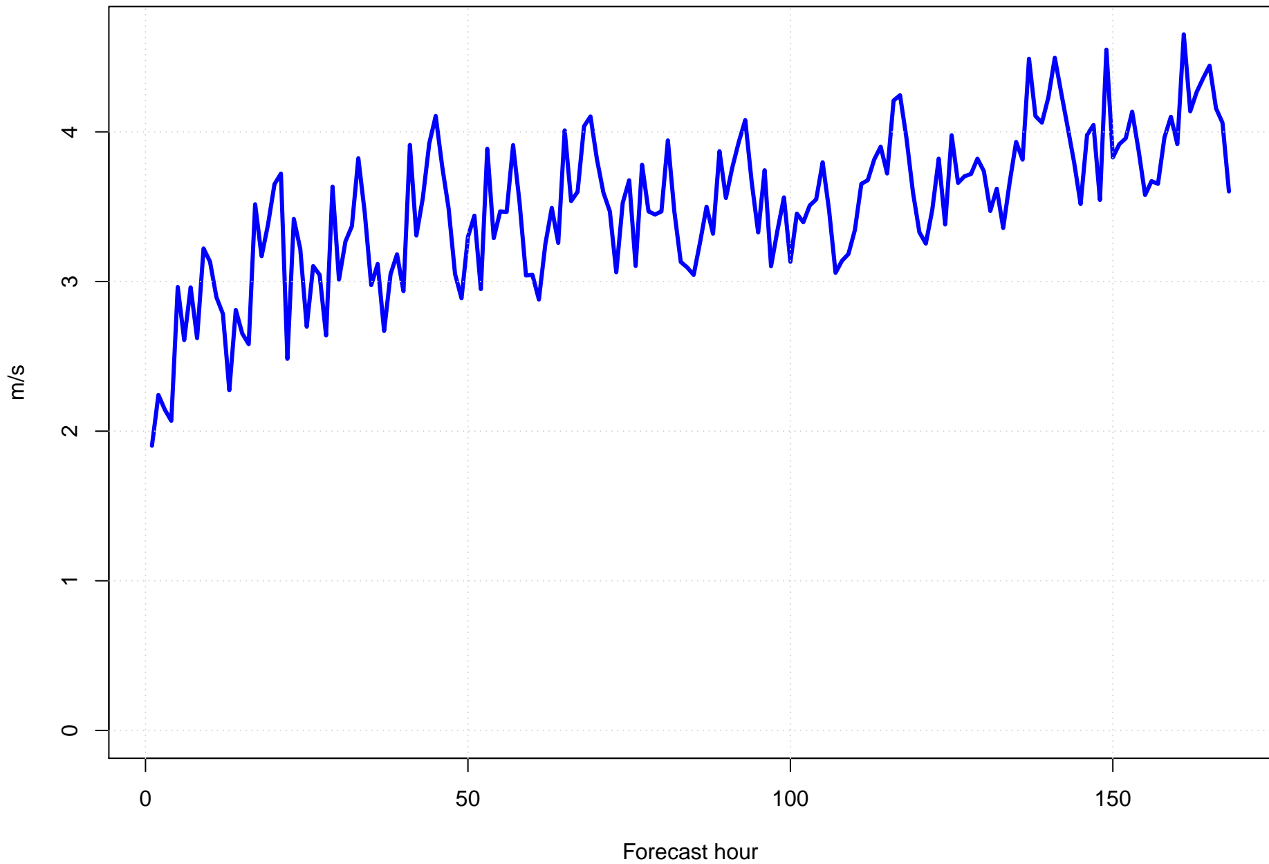
Surface vector wind error at KPNS by forecast hour
