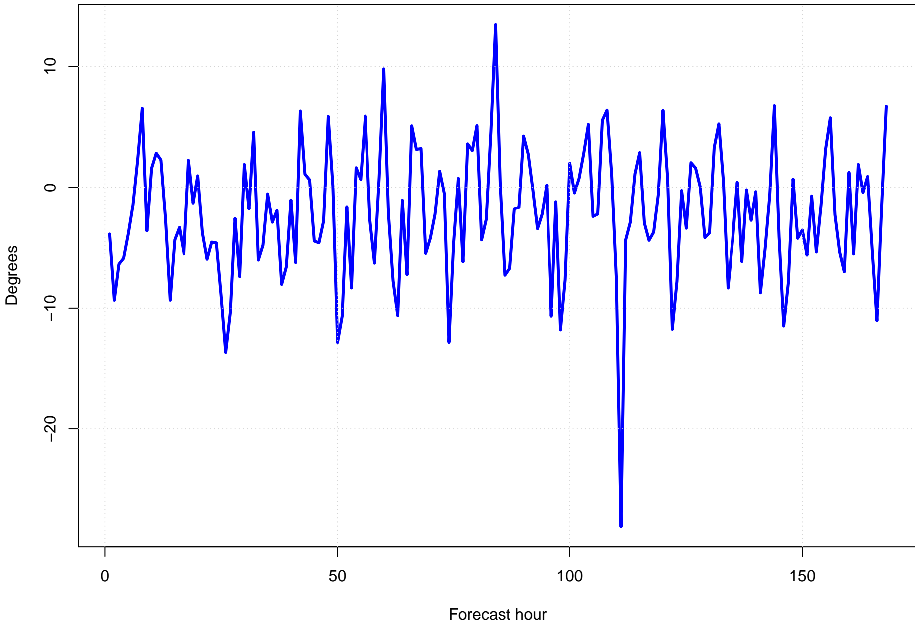
Surface wind direction bias at KPNS by forecast hour
