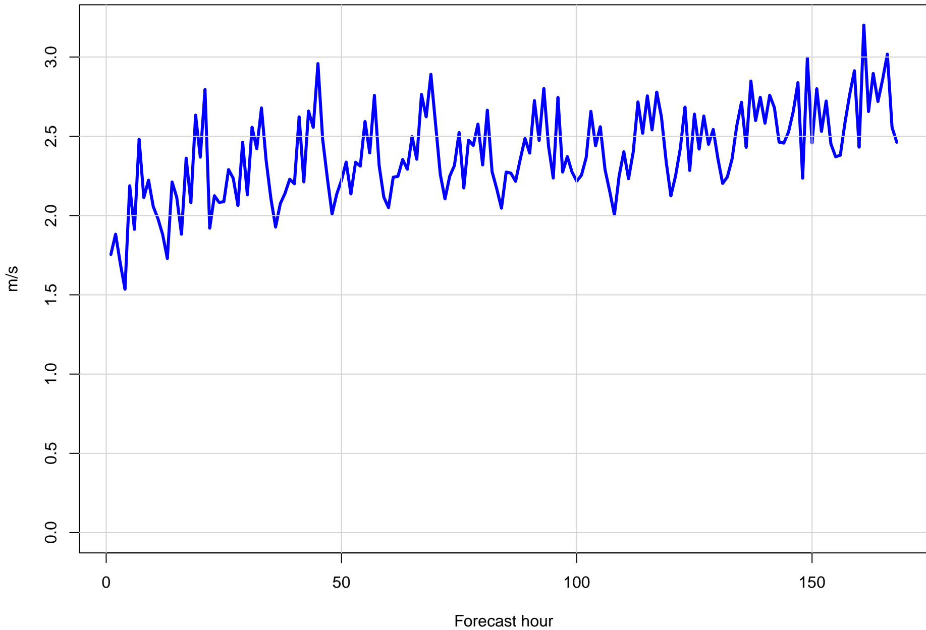
Surface wind speed RMSE at KPNS by forecast hour
