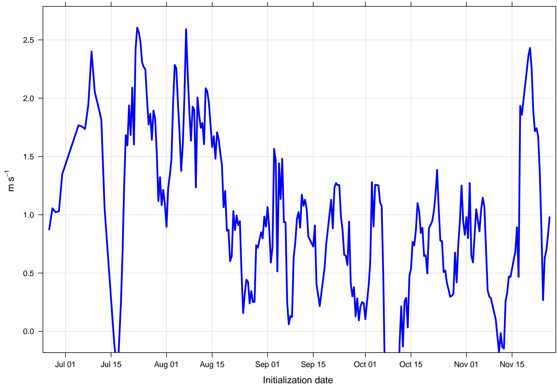
Surface wind speed bias at KPNS all forecast hours and members
