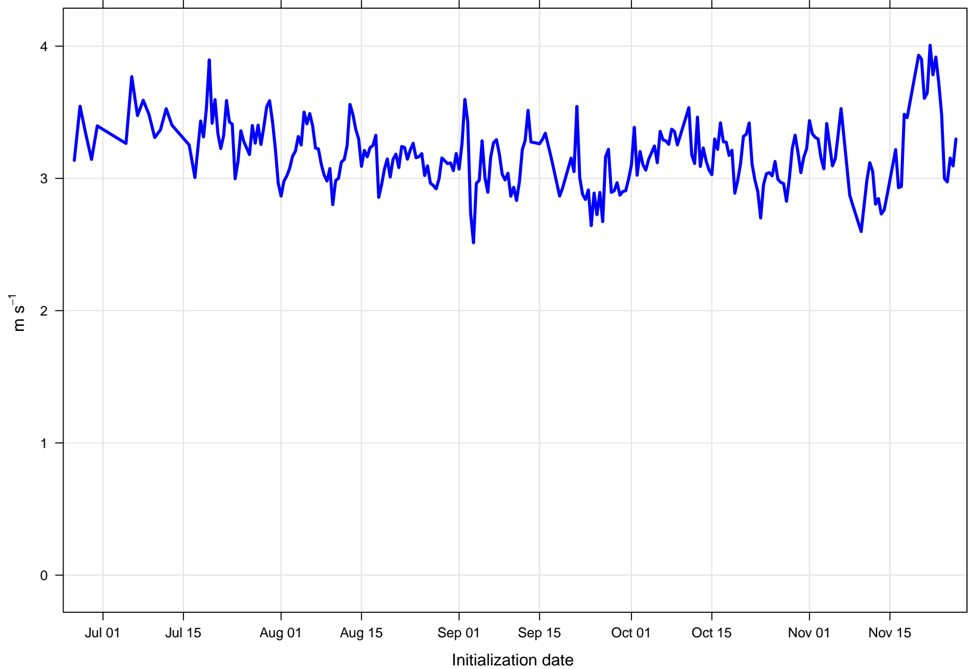
Surface vector wind mean error KRQU all forecast hours and members
