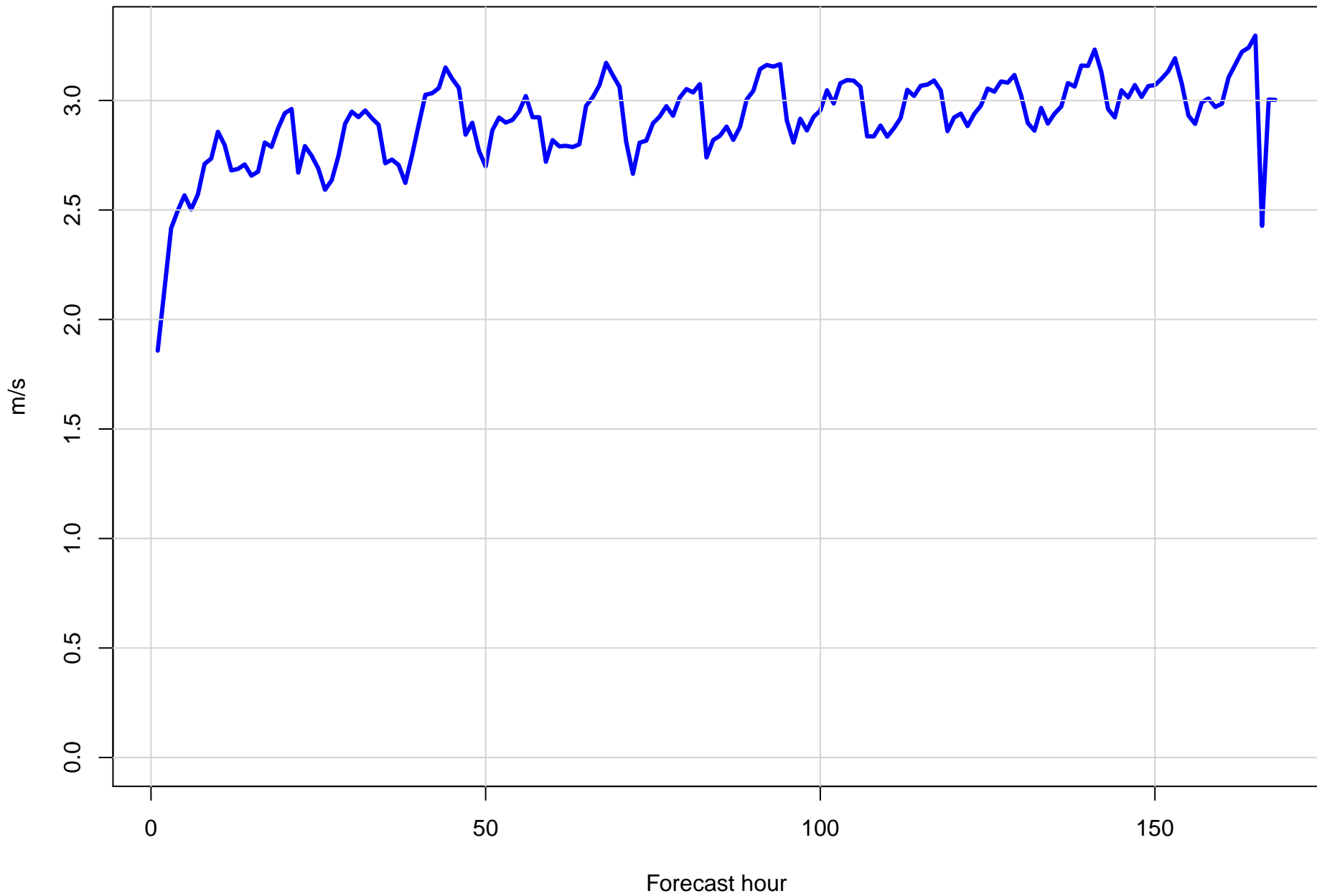
Surface wind speed RMSE at KRUQ by forecast hour
