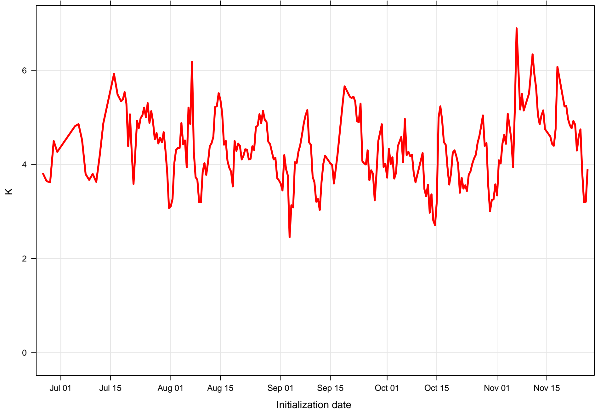
Surface temperature RMSE at KRUQ all forecast hours and members
