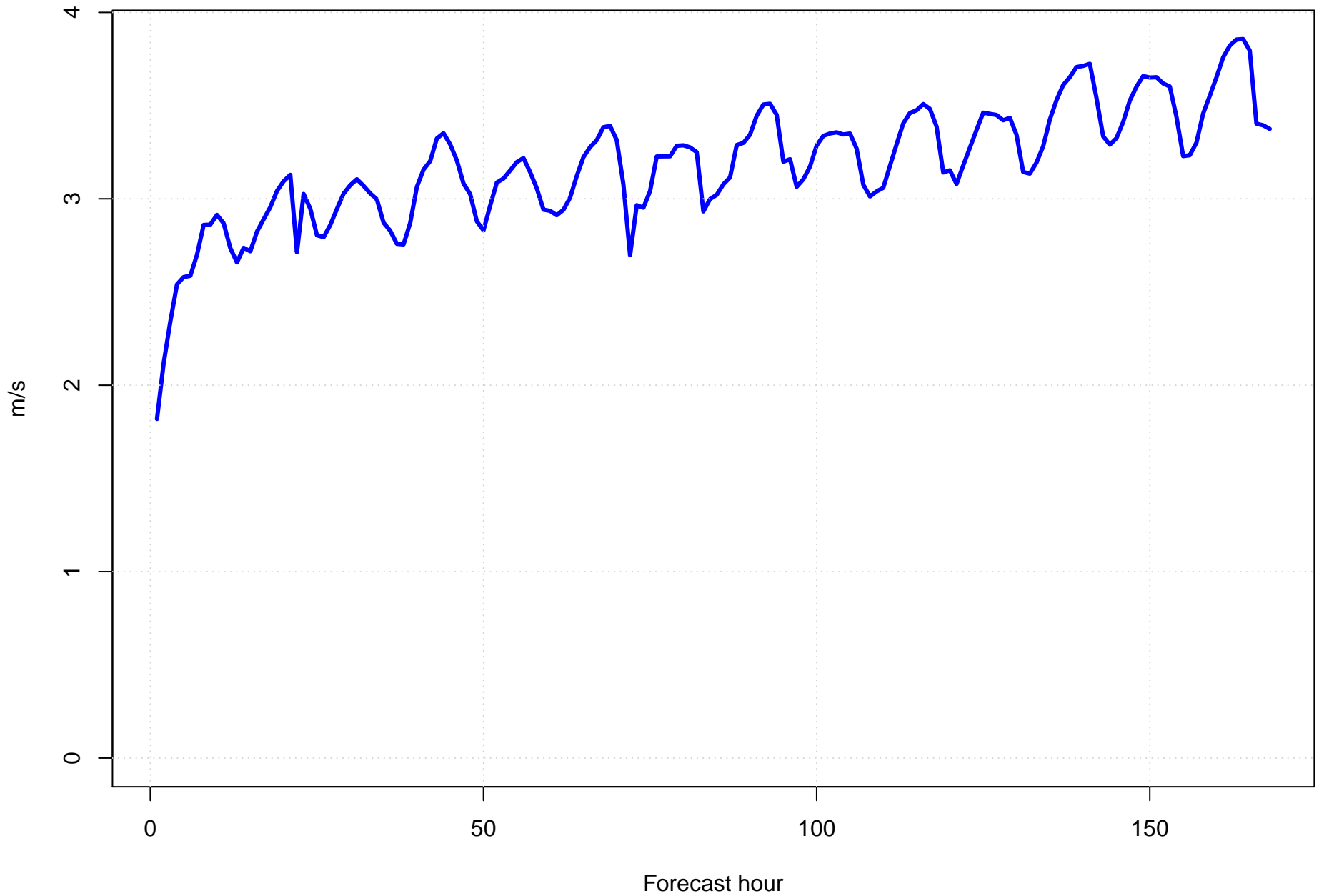
Surface vector wind error at KRUQ by forecast hour
