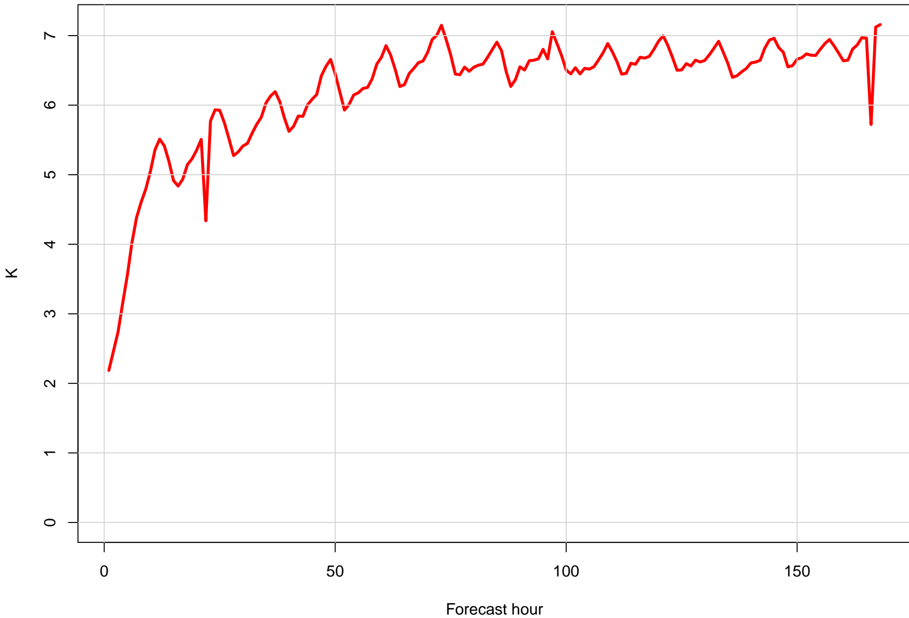
Surface dew point RMSE at KRUQ by forecast hour
