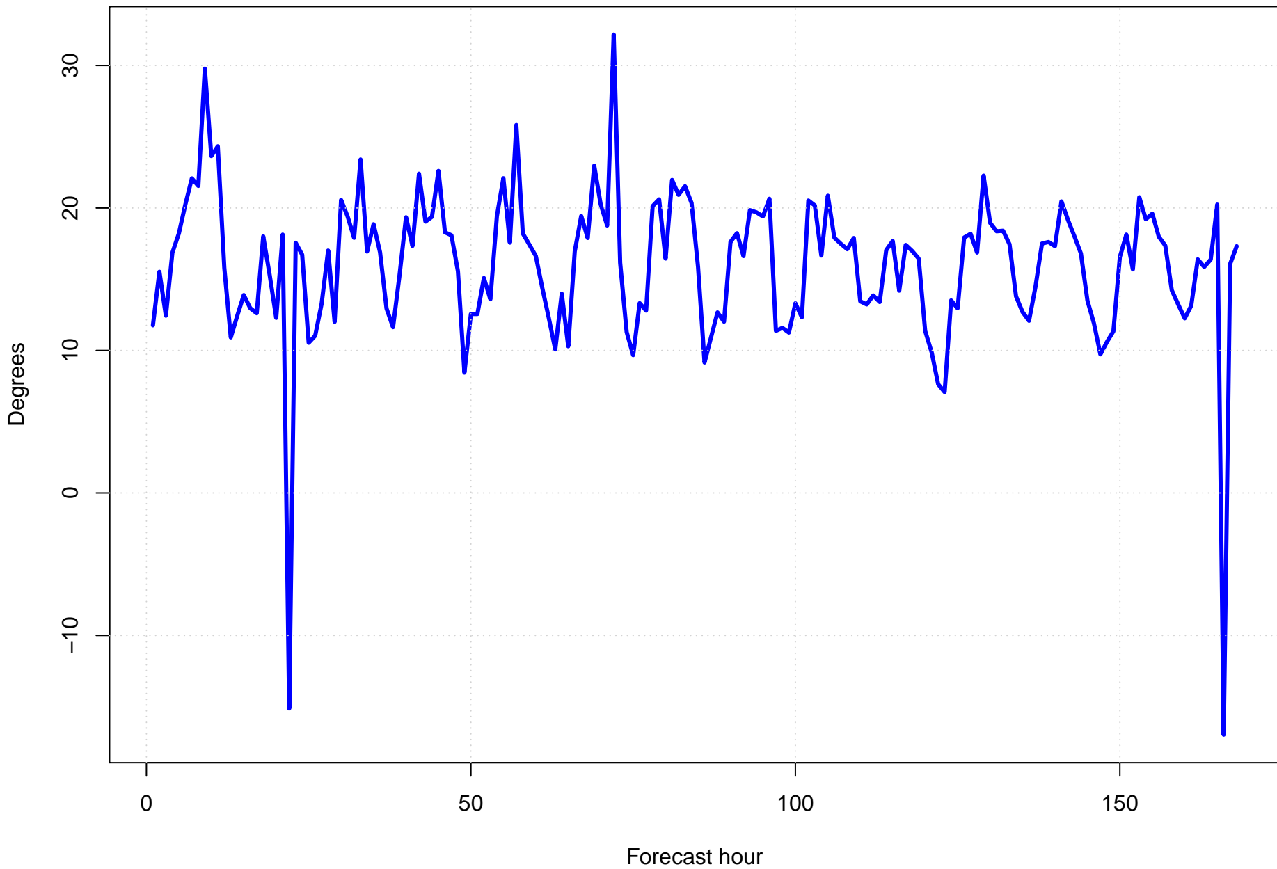
Surface wind direction bias at KRUQ by forecast hour
