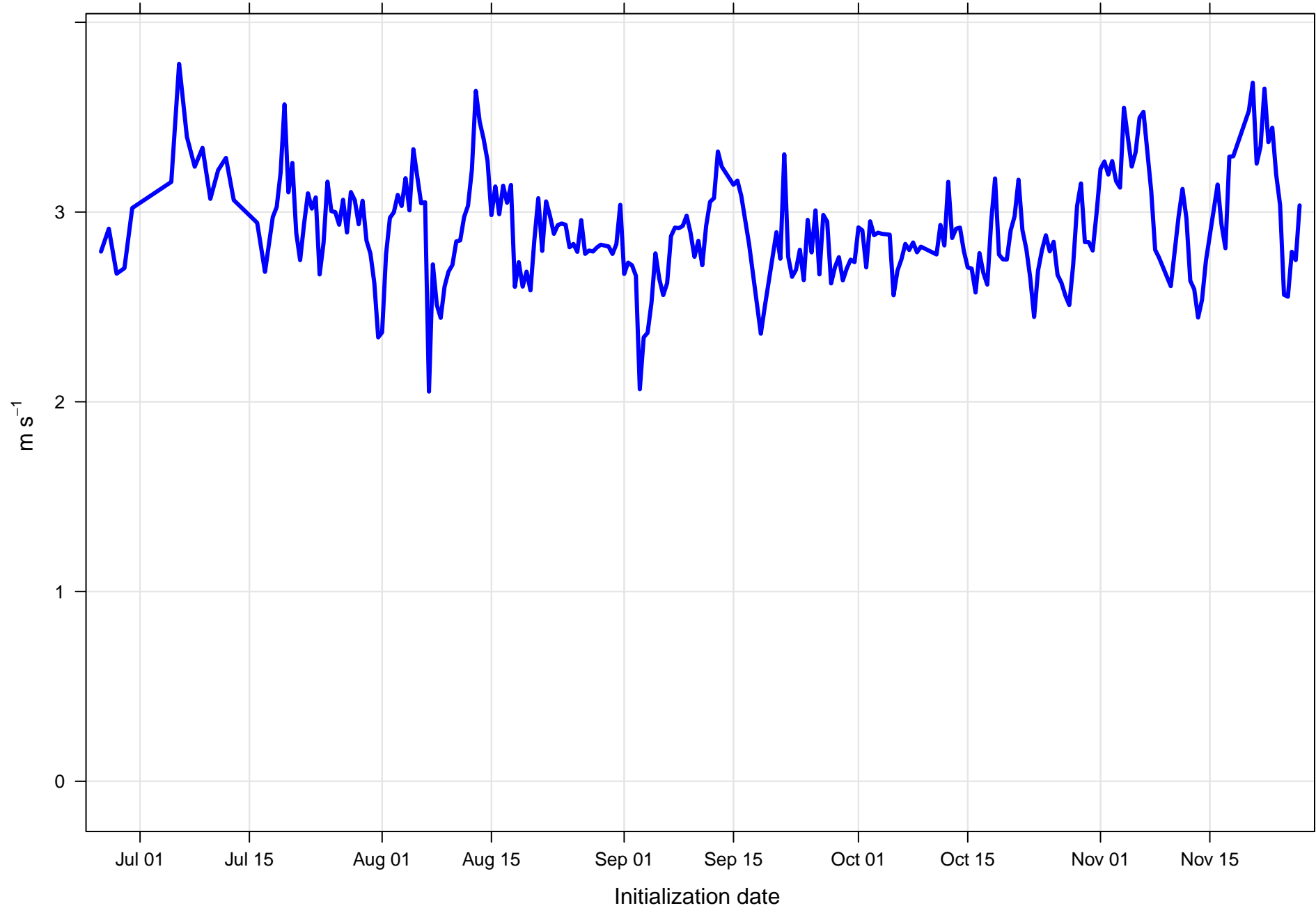
Surface wind speed RMSE at KRUQ all forecast hours and members
