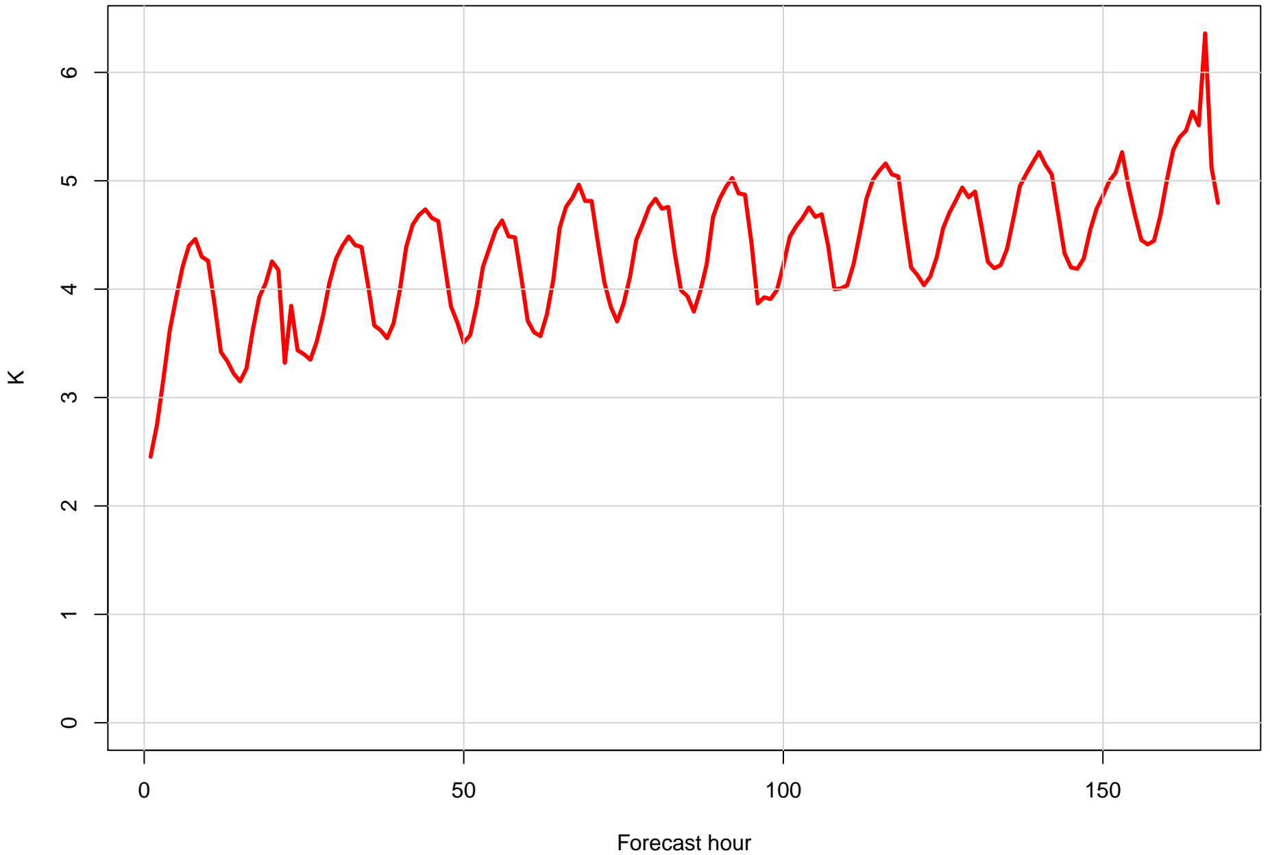
Surface temperature RMSE at KRUQ by forecast hour
