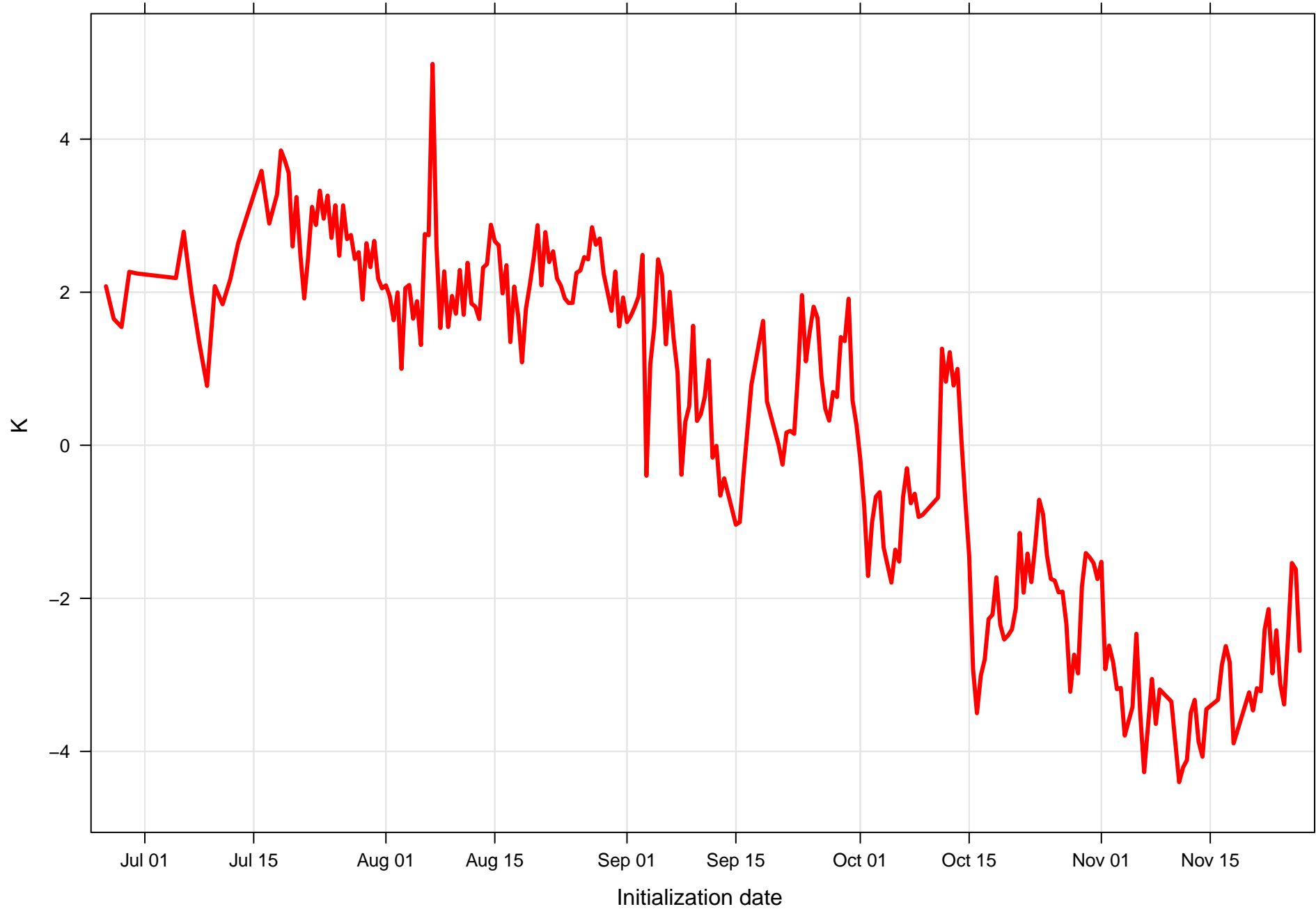
Surface temperature bias at KRUQ all forecast hours and members
