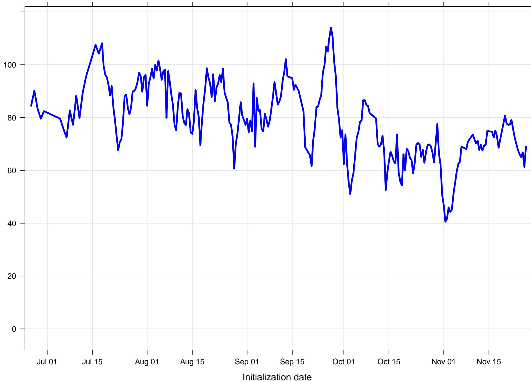
Surface wind direction RMSE at KRUQ all forecast hours and members
