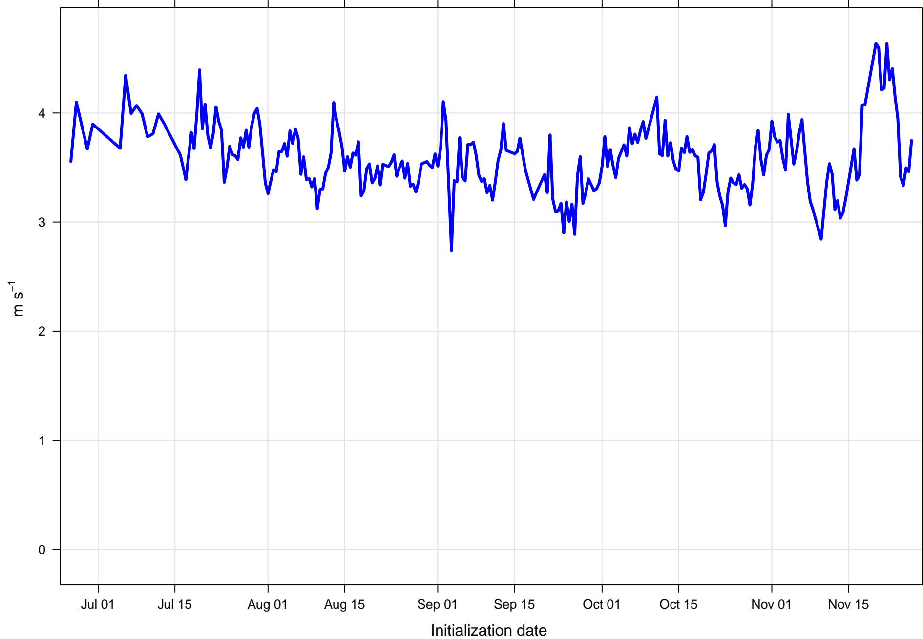
Surface vector wind RMSE at KRUQ all forecast hours and members
