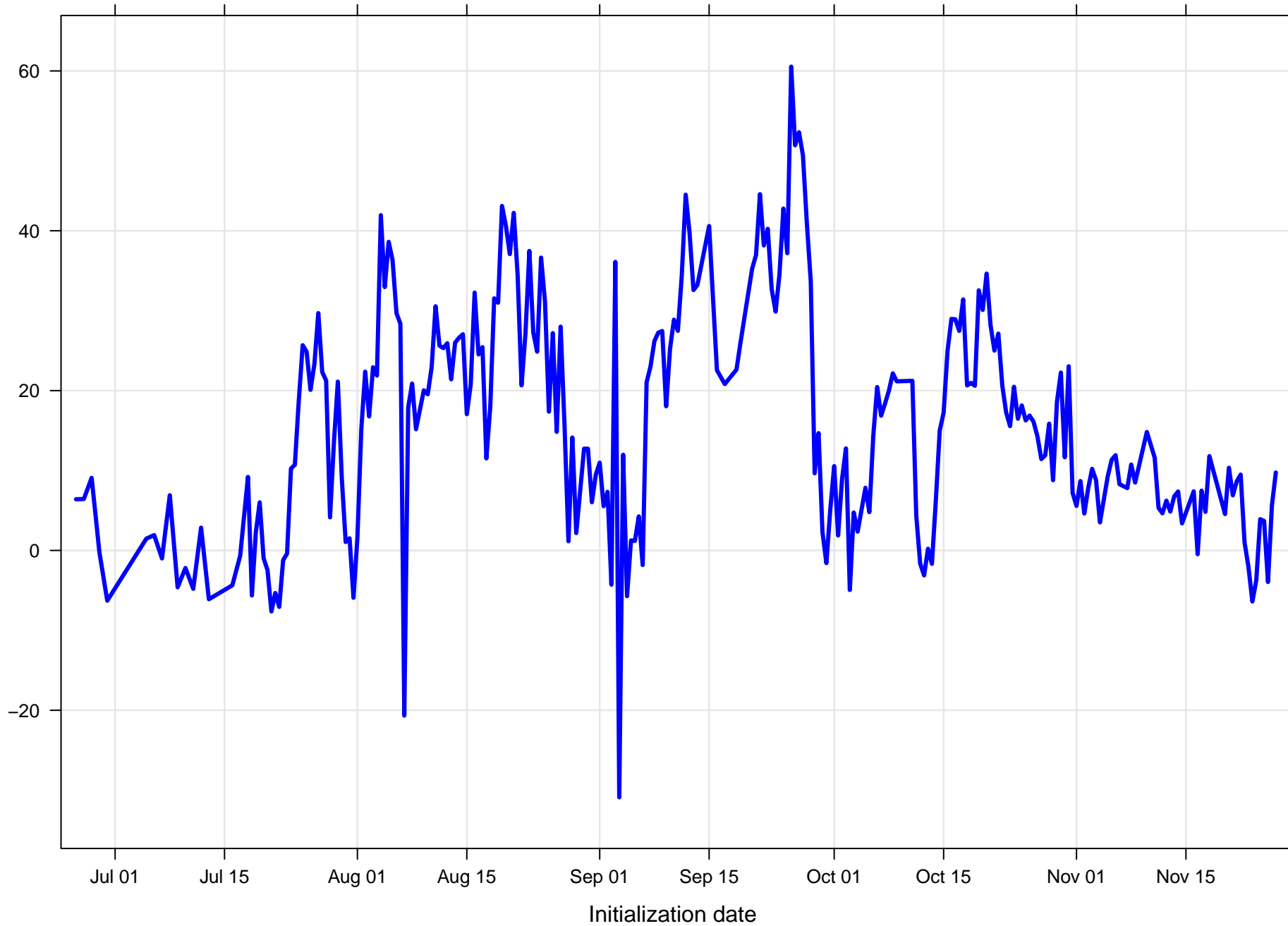
Surface wind direction bias at KRUQ all forecast hours and members
