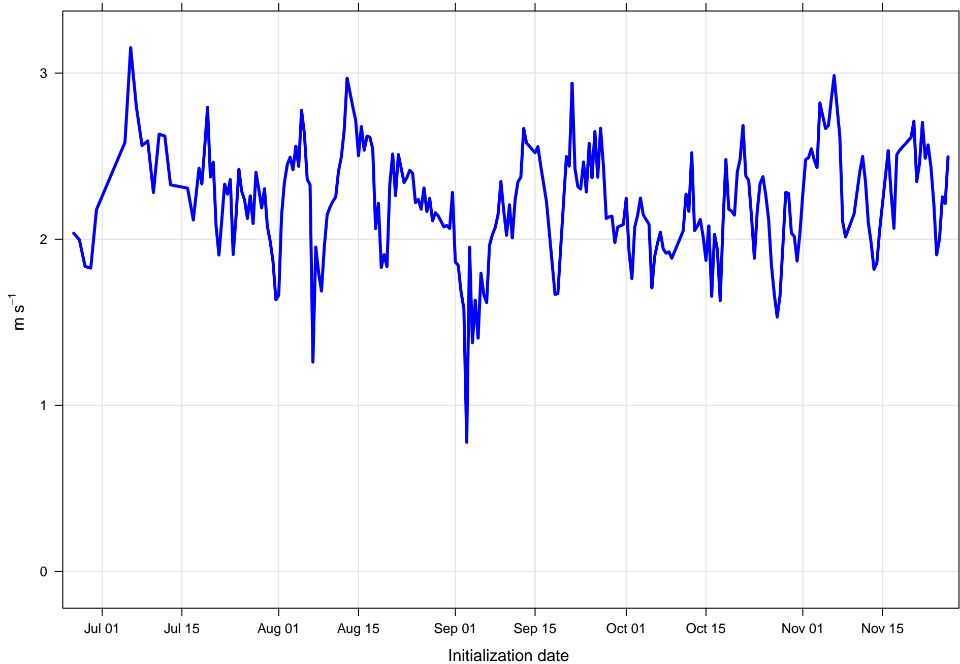
Surface wind speed bias at KRUQ all forecast hours and members
