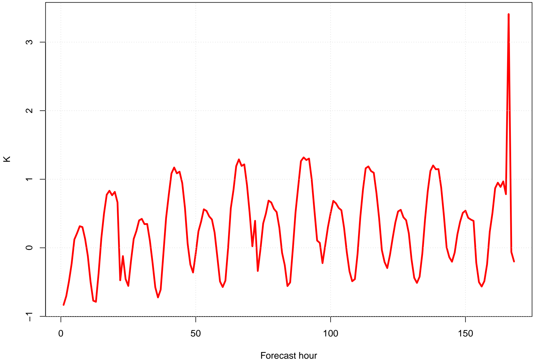
Surface temperature bias at KRUQ by forecast hour
