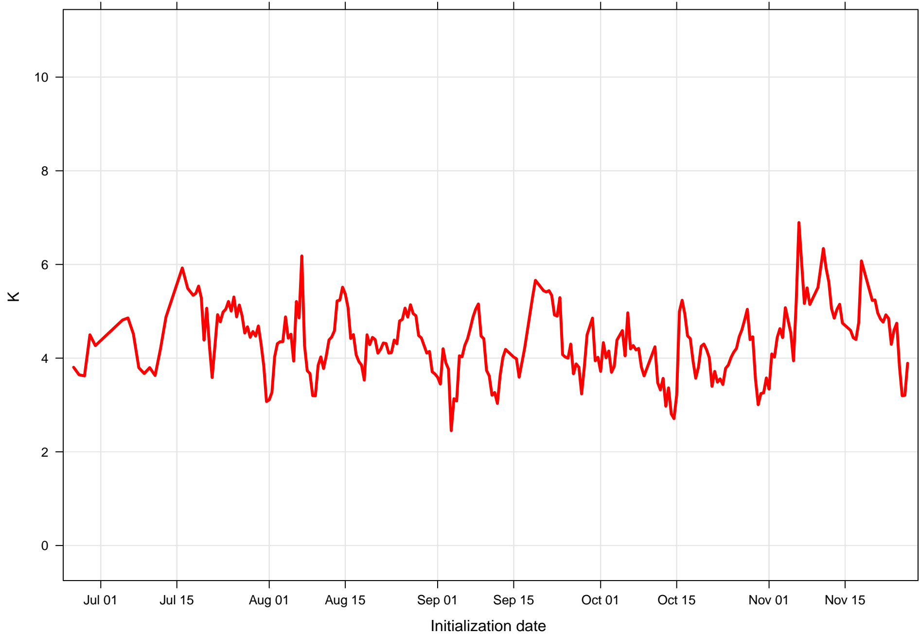
Surface dew point RMSE at KRUQ all forecast hours and members
