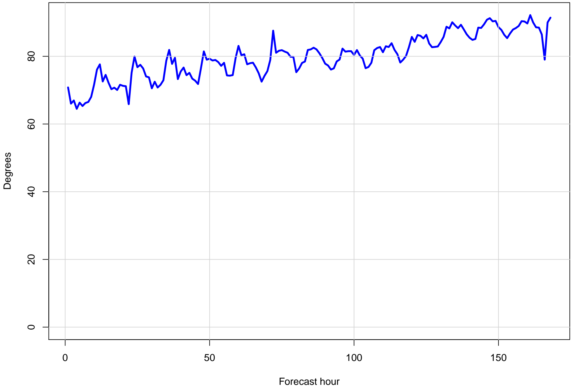
Surface wind direction RMSE at KRUQ by forecast hour
