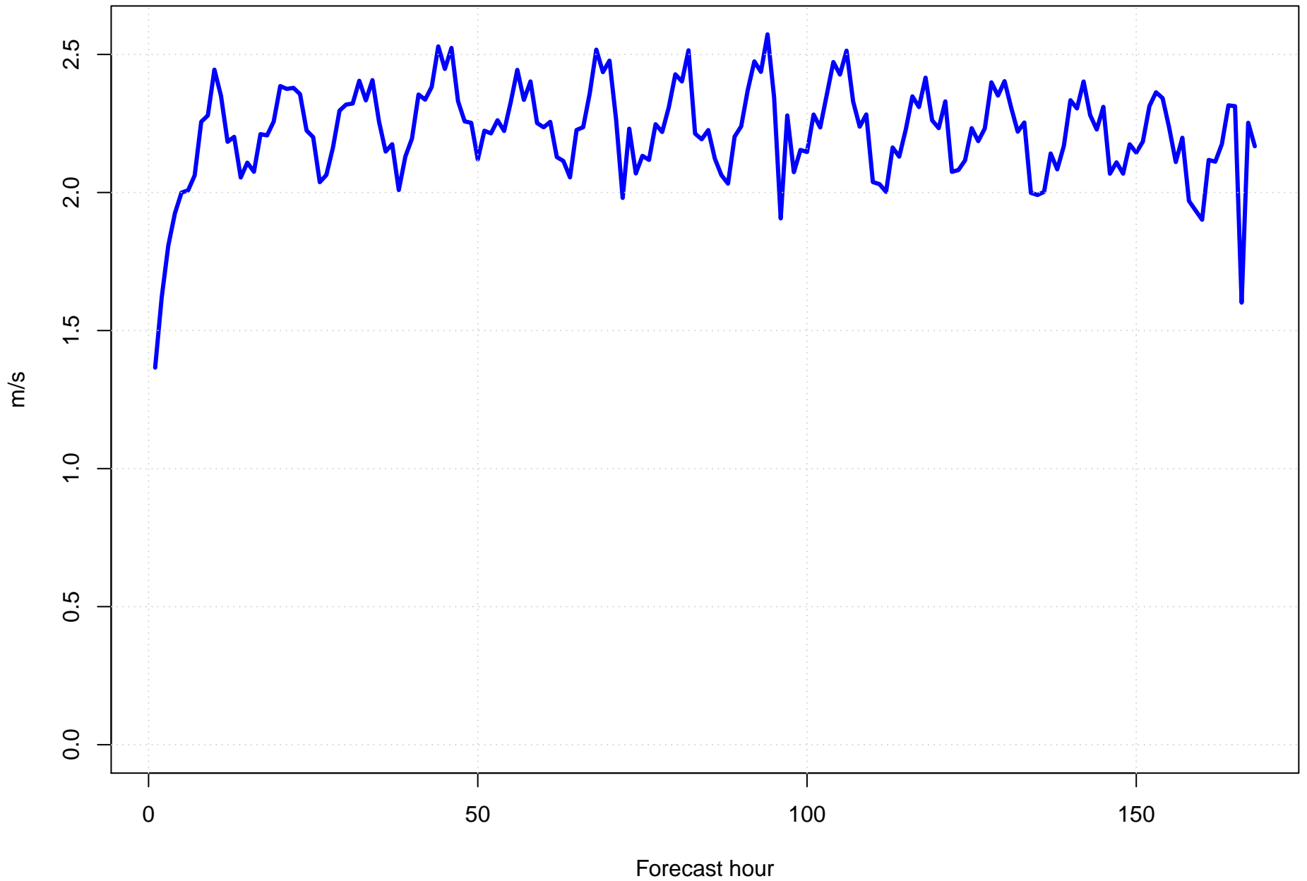
Surface wind speed bias at KRUQ by forecast hour
