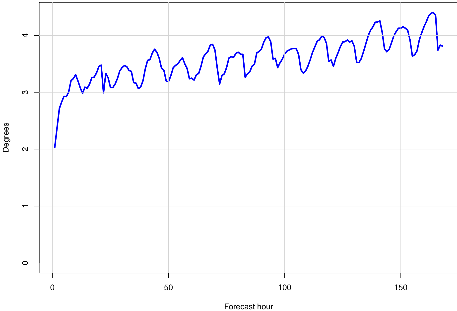
Surface vector wind RMSE at KRUQ by forecast hour
