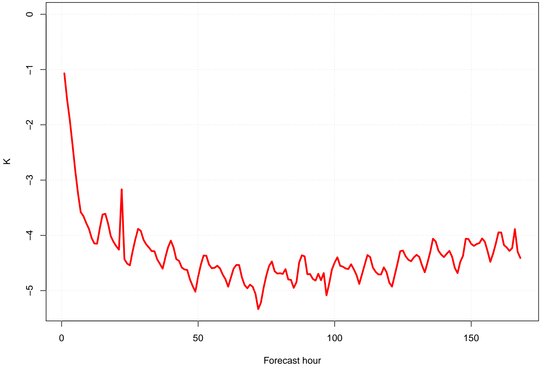
Surface dew point bias at KRUQ by forecast hour
