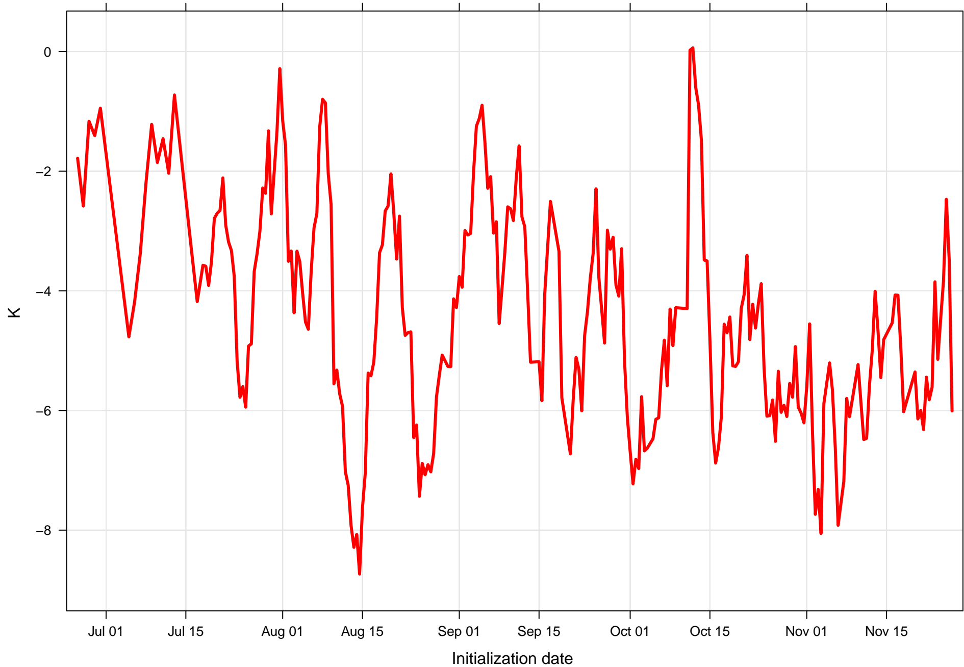
Surface dew point bias at KRUQ all forecast hours and members
