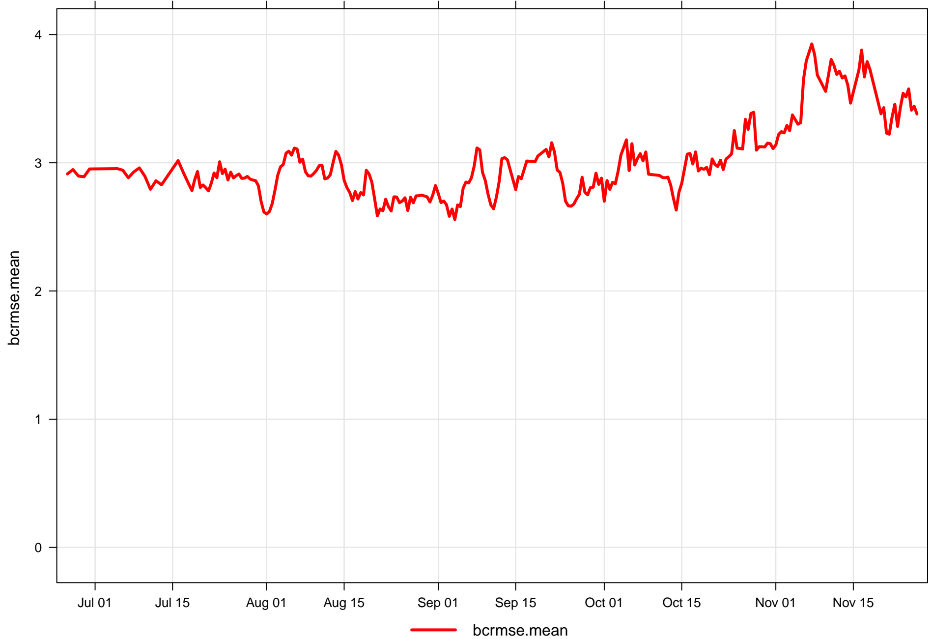
Surface Temperature Bias-corrected RMSE : All Stations, all dates and ensemble members
